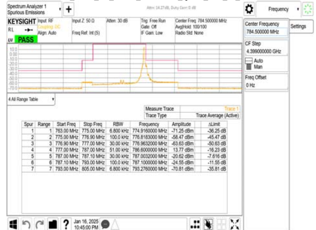
Band13_5MHz_CP_OFDM_SCS15kHz_QPSK_RB25_0_CH156900
