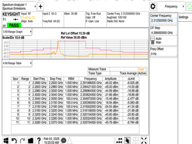
Band30 10MHz DFT s OFDM SCS15kHz BPSK RB1_51 CH462000
