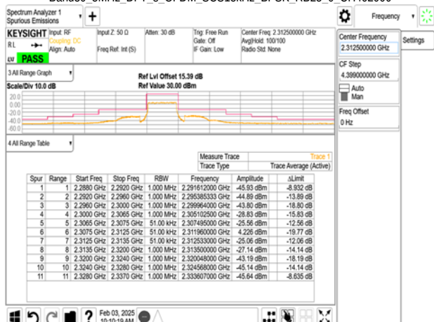
Band30_5MHz_DFT_s_OFDM_SCS15kHz_BPSK_RB25_0_CH462000
