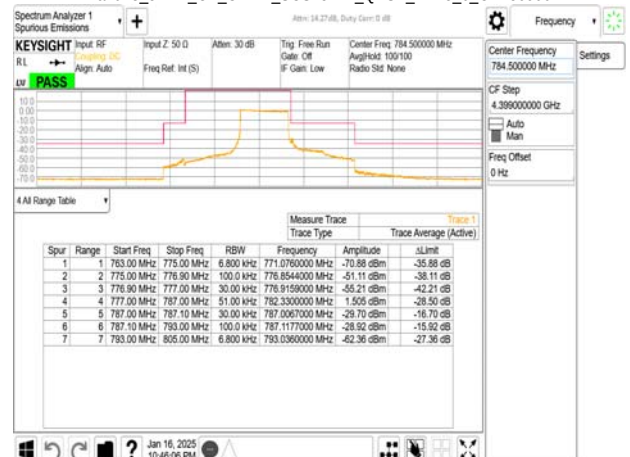
Band13_5MHz_CP_OFDM_SCS15kHz_QPSK_RB25_0_CH156900
