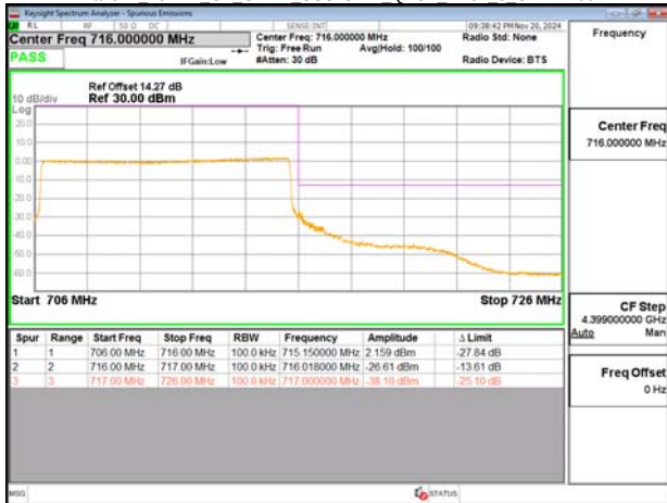
Band12 15MHz DFT s OFDM SCS15kHz BPSK RB1 0 CH141300
