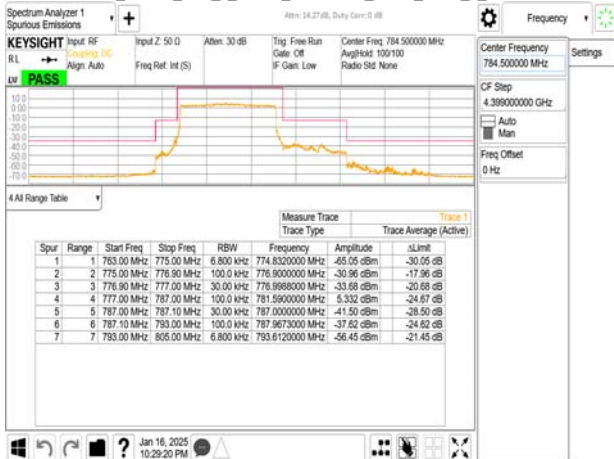
Band13 10MHz CP_OFDM_SCS15kHz QPSK_RB1_0_CH156400
