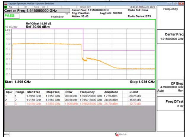
Band25 20MHz CP OFDM SCS15kHz QPSK RB1 105 CH381000
