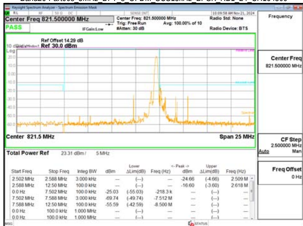
Band26-Part90s 5MHz DFT s OFDM SCS15kHz BPSK RB1 24 CH164300
