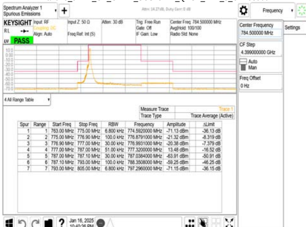
Band13_5MHz_CP_OFDM_SCS15kHz_QPSK_RB1_0_CH155900
