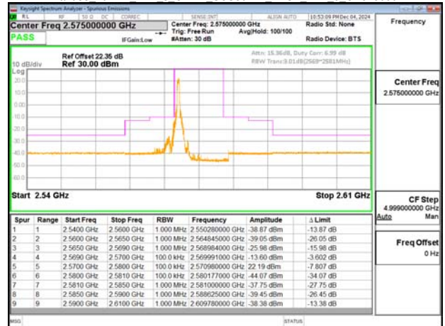
Band38 10MHz DFT s OFDM SCS30kHz BPSK RB1_23 CH515000
