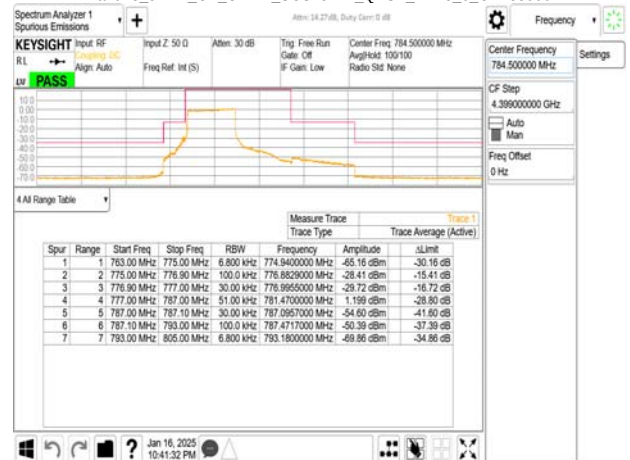
Band13_5MHz_CP_OFDM_SCS15kHz_QPSK_RB1_24_CH156900
