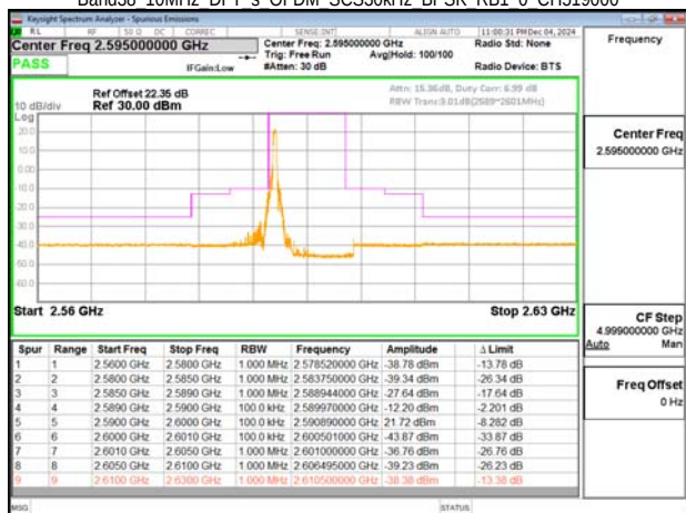
Band38 10MHz DFT s OFDM SCS30kHz BPSK RB1 23 CH519000
