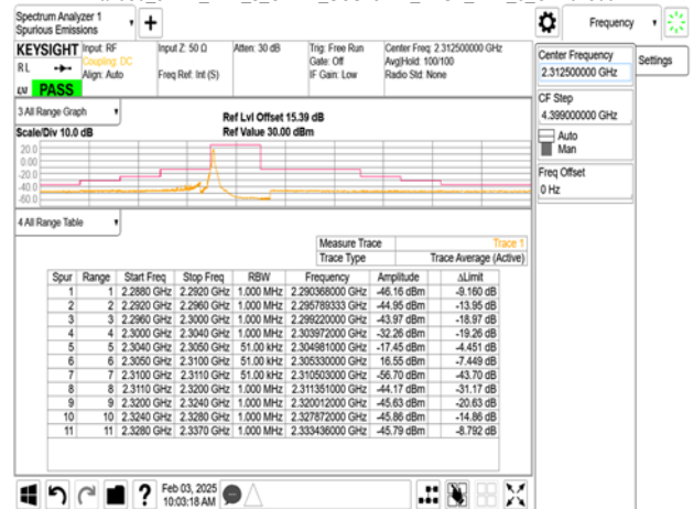
Band30 5MHz DFT_s OFDM SCS15kHz BPSK RB1_24 CH461500
