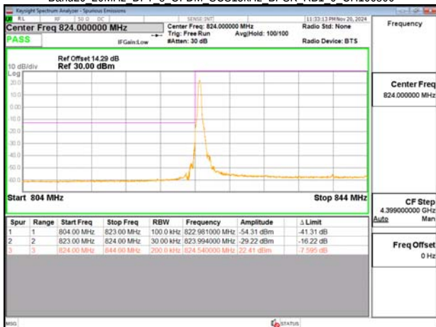
Band26 20MHz DFT s OFDM SCS15kHz BPSK RB1 0 CH166800
