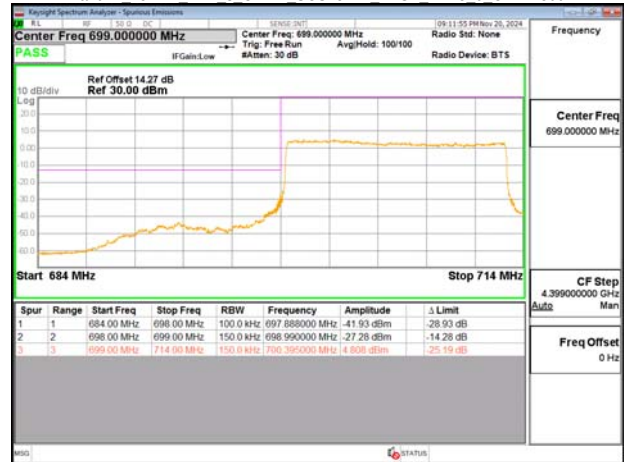
Band12 15MHz DFT s OFDM SCS15kHz BPSK RB1 78 CH141700
