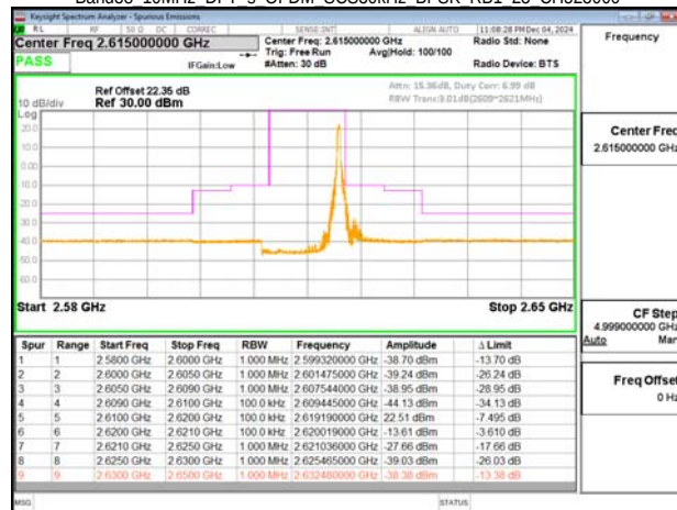
Band38 10MHz DFT s OFDM SCS30kHz BPSK RB24 0 CH523000
