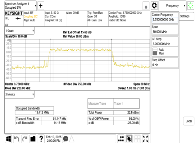
Band43-Part27_15MHz_QPSK_RB75_0_CH45515
