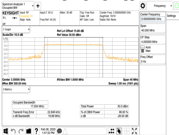
Band42-Part27_20MHz_16QAM_RB100_0_CH42590
