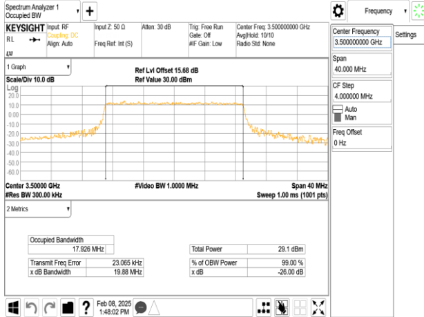
Band42-Part27_20MHz_64QAM_RB100_0_CH42590
