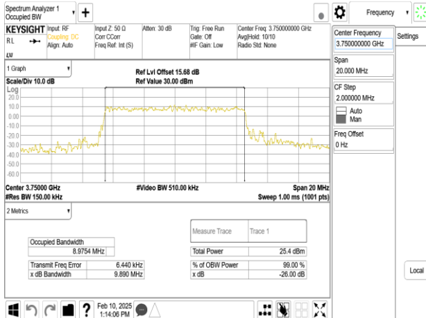
Band43-Part27_10MHz_64QAM_RB50_0_CH45090
