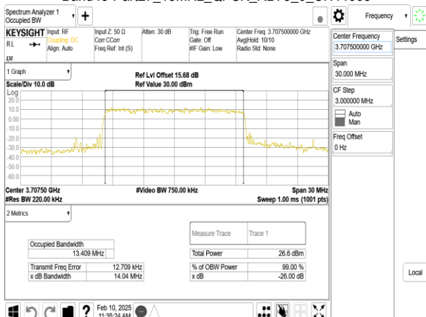
Band43-Part27_15MHz_QPSK_RB75_0_CH44665
