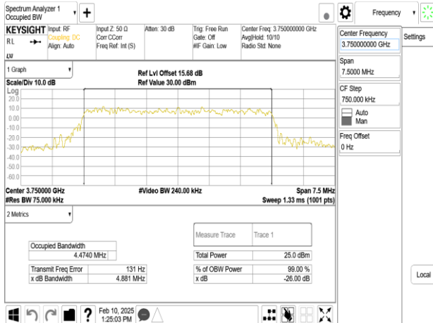
Band43-Part27_5MHz_64QAM_RB25_0_CH45090
