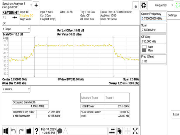
Band43-Part27_5MHz_16QAM_RB25_0_CH45090
