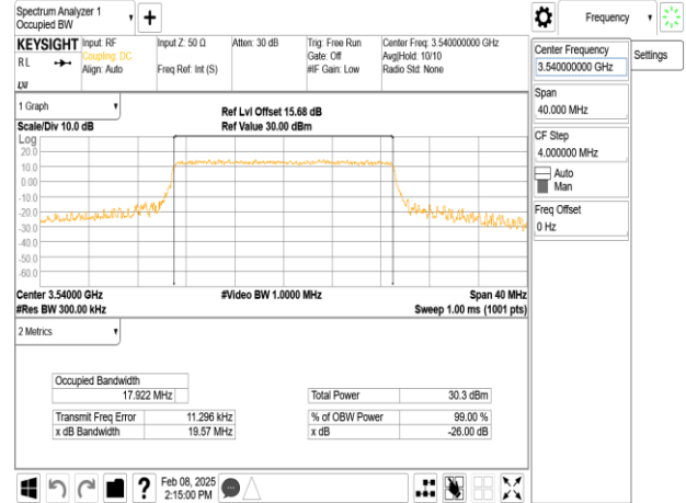
Band42-Part27_20MHz_16QAM_RB100_0_CH42990
