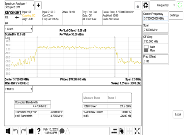
Band43-Part27_5MHz_QPSK_RB25_0_CH45565
