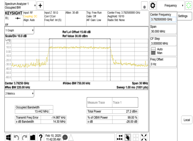
Band43-Part27_15MHz_16QAM_RB75_0_CH45515
