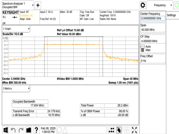
Band42-Part27_20MHz_256QAM_RB100_0_CH42990
