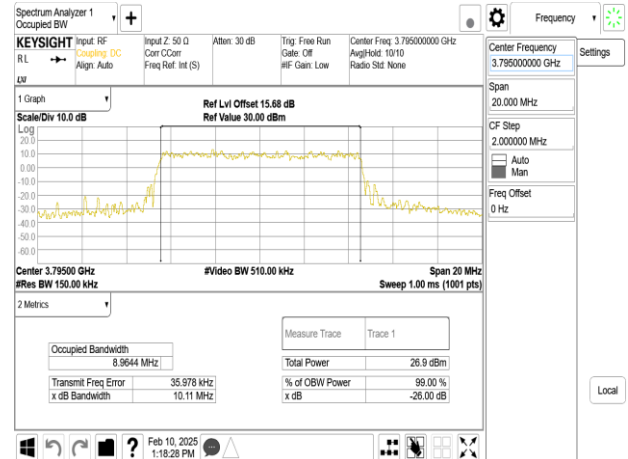
Band43-Part27_10MHz_16QAM_RB50_0_CH45540
