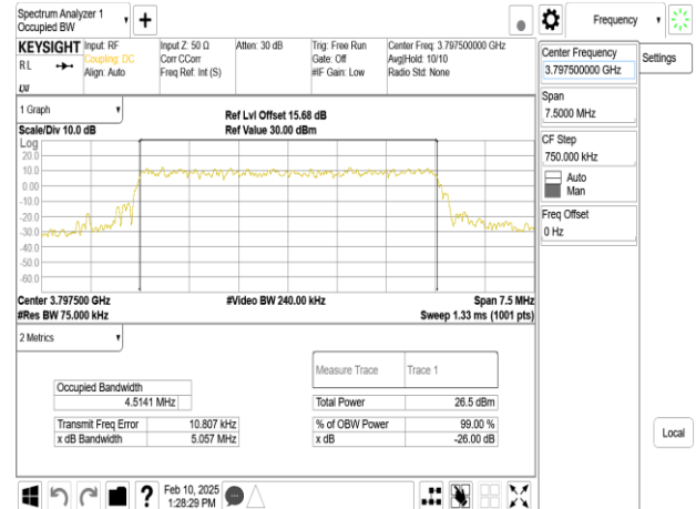
Band43-Part27_5MHz_16QAM_RB25_0_CH45565
