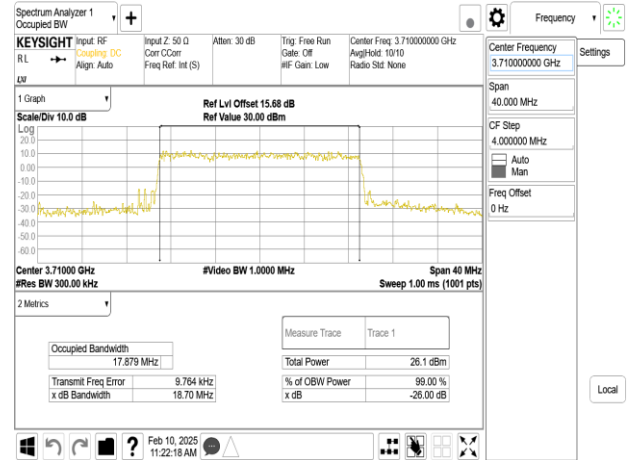
Band43-Part27_20MHz_64QAM_RB100_0_CH44690
