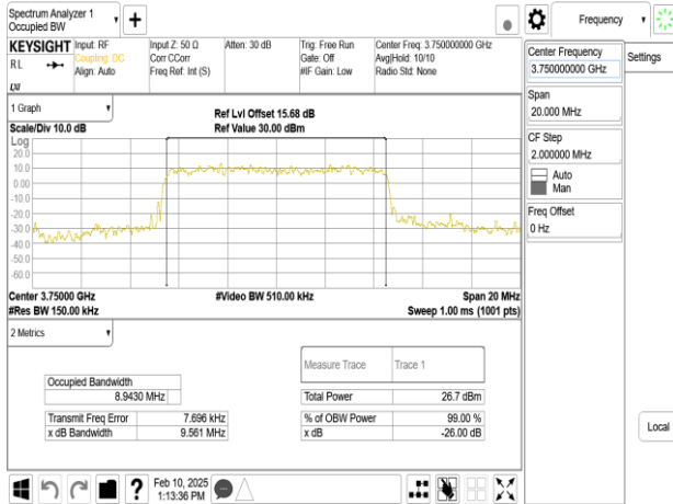
Band43-Part27_10MHz_16QAM_RB50_0_CH45090
