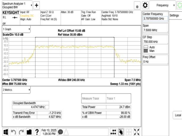
Band43-Part27_5MHz_256QAM_RB25_0_CH45565
