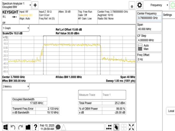
Band43-Part27_20MHz_256QAM_RB100_0_CH45490
