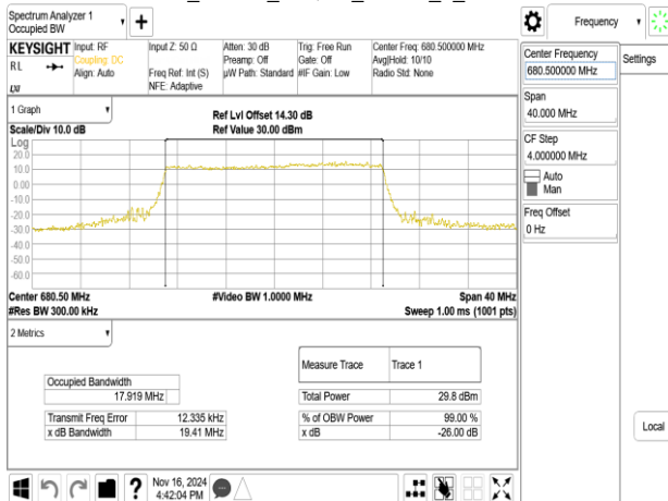
Band71_20MHz_256QAM_RB100_0_CH133297
