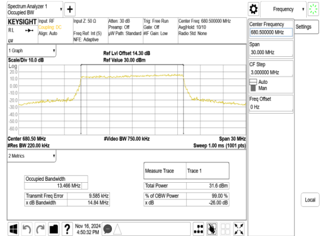
Band71_15MHz_16QAM_RB75_0_CH133297
