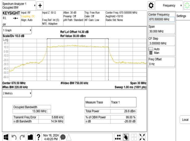
Band71_15MHz_64QAM_RB75_0_CH133197
