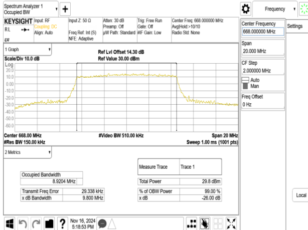
Band71_10MHz_64QAM_RB50_0_CH133172
