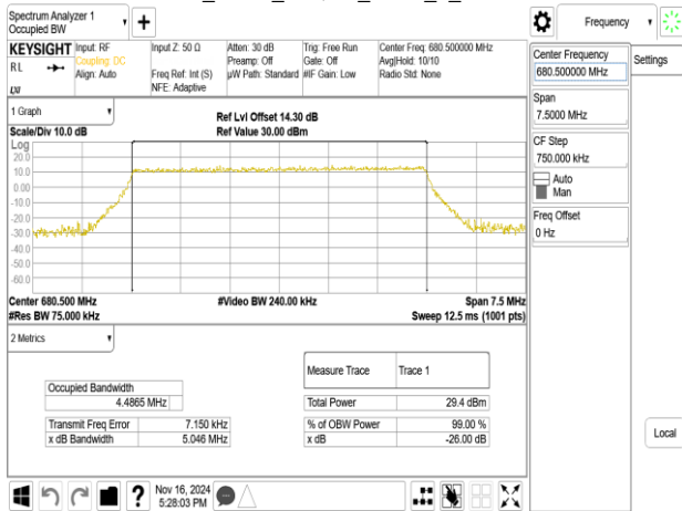
Band71_5MHz_256QAM_RB25_0_CH133297
