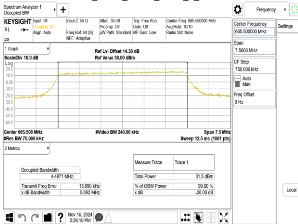
Band71_5MHz_16QAM_RB25_0_CH133147
