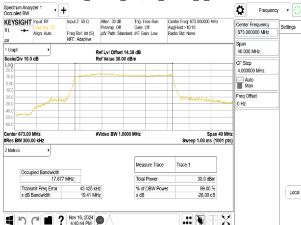
Band71_20MHz_64QAM_RB100_0_CH133222
