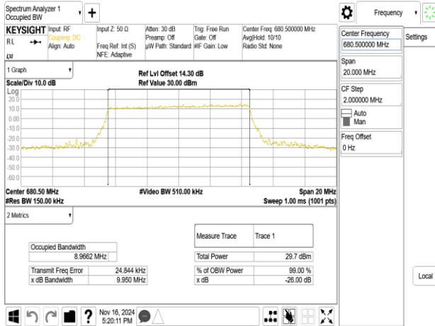
Band71_10MHz_256QAM_RB50_0_CH133297
