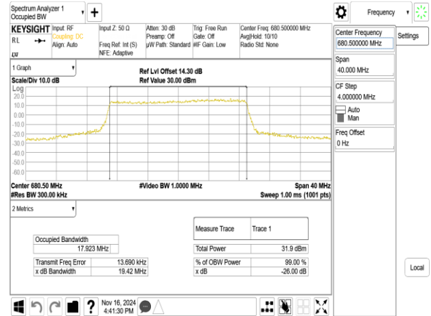
Band71_20MHz_16QAM_RB100_0_CH133297
