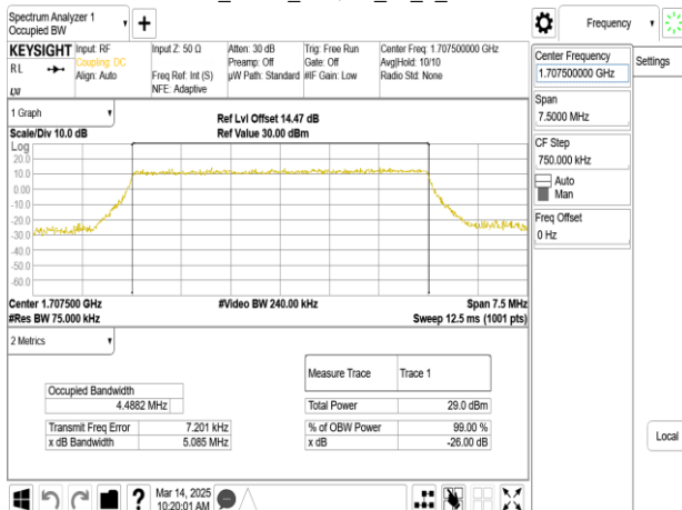
Band70_5MHz_64QAM_25_0_CH133097
