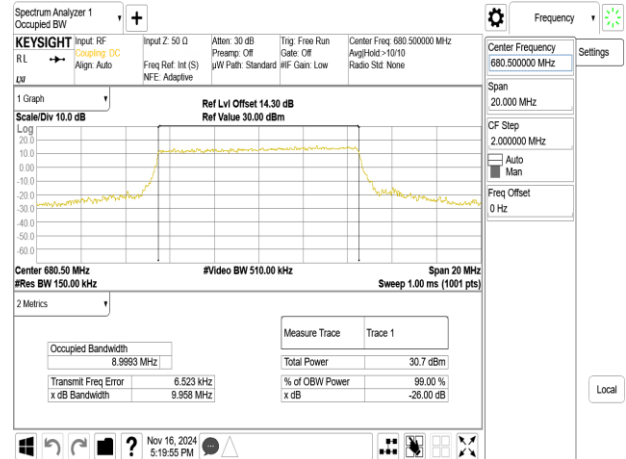
Band71_10MHz_16QAM_RB50_0_CH133297
