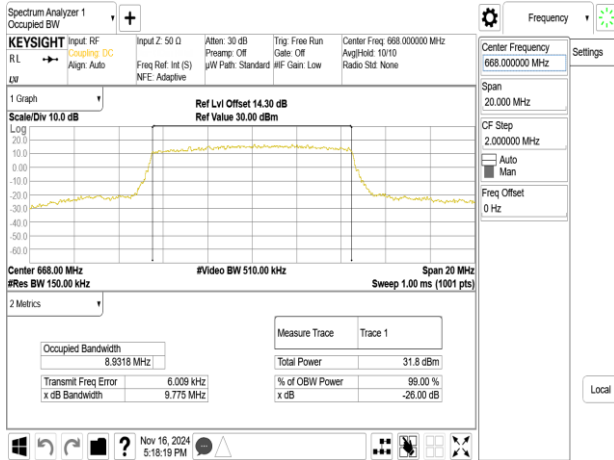
Band71_10MHz_16QAM_RB50_0_CH133172
