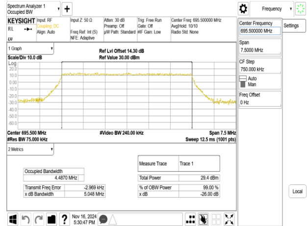
Band71_5MHz_256QAM_RB25_0_CH133447
