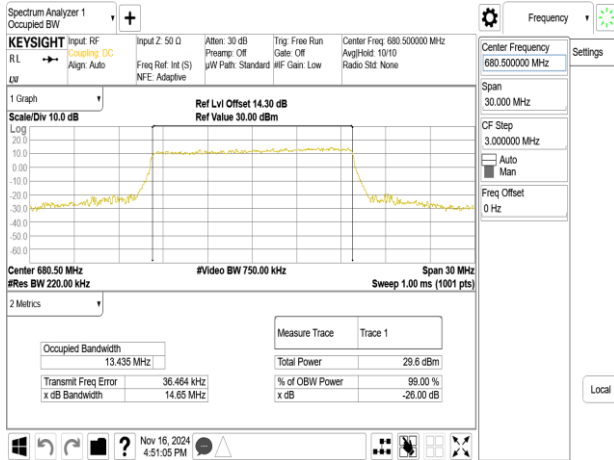
Band71_15MHz_256QAM_RB75_0_CH133297
