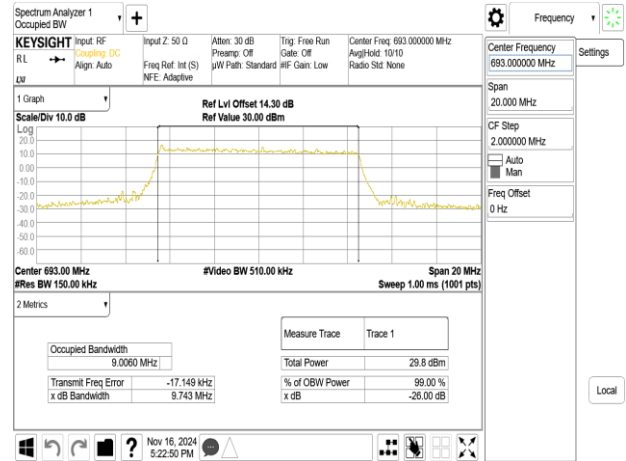
Band71_10MHz_256QAM_RB50_0_CH133422
