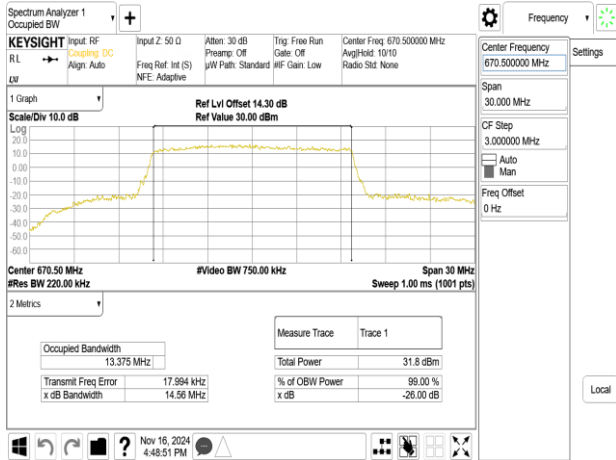
Band71_15MHz_16QAM_RB75_0_CH133197
