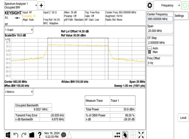
Band71_10MHz_64QAM_RB50_0_CH133422
