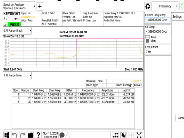
Band2_3MHz_QPSK_RB15_0_CH18615
