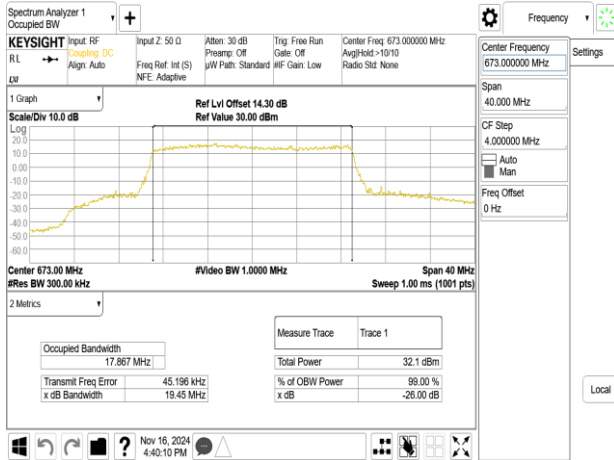
Band71_20MHz_16QAM_RB100_0_CH133222
