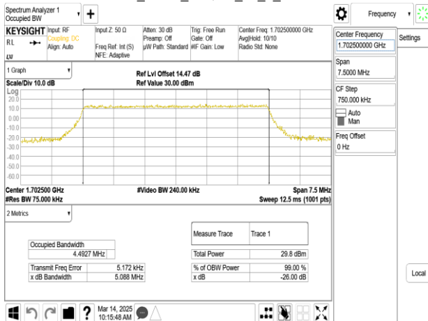
Band70_5MHz_16QAM_25_0_CH133097
