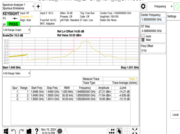
Band2_1.4MHz_QPSK_RB6_0_CH18607
