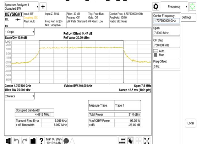
Band70_5MHz_QPSK_25_0_CH133097
