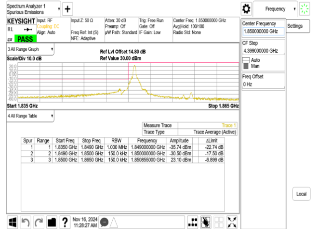
Band25_15MHz_QPSK_RB75_0_CH26115
