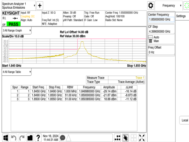
Band25_5MHz_QPSK_RB25_0_CH26065
