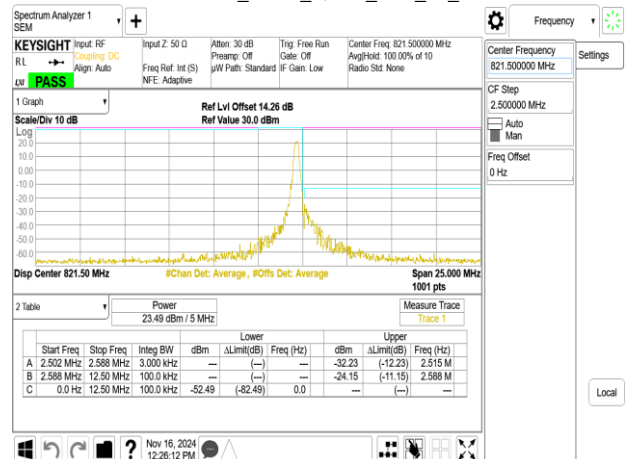
Band26-Part90s_5MHz_QPSK_RB1_24_CH26765
