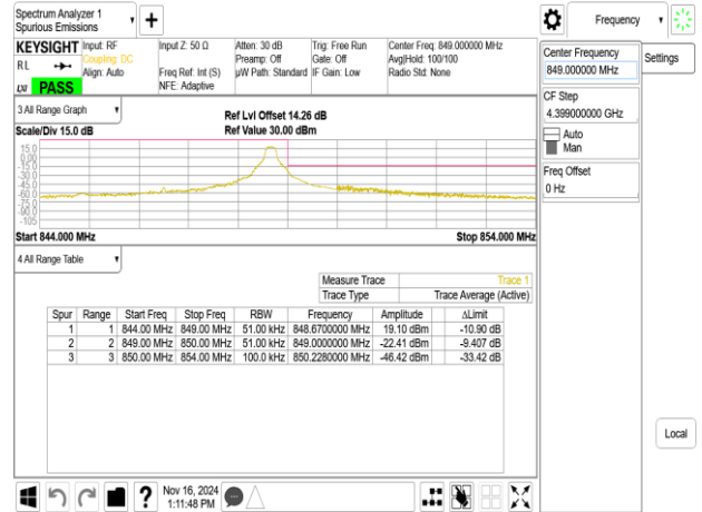
Band26_5MHz_QPSK_RB25_0_CH27015
