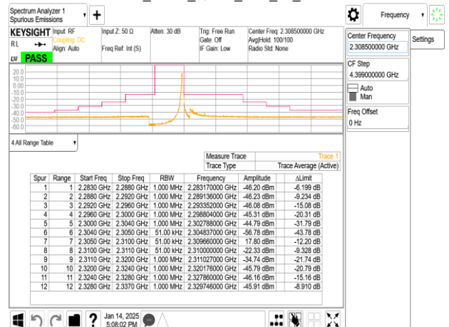
Band30_5MHz_QPSK_RB1_24_CH27685
