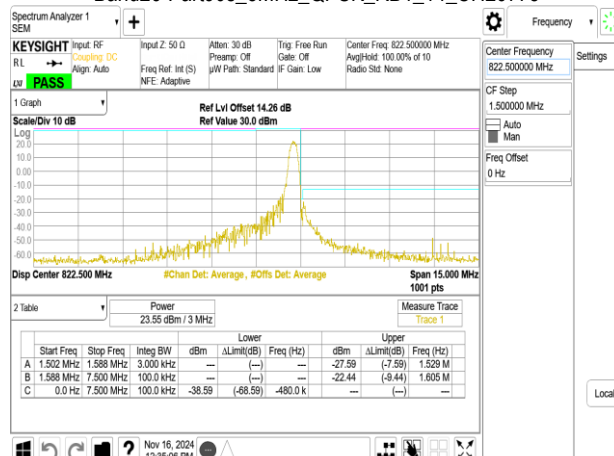
Band26-Part90s_3MHz_QPSK_RB15_0_CH26775
