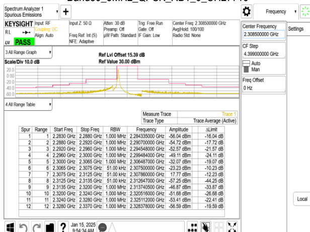
Band30_5MHz_QPSK_RB1_24_CH27710
