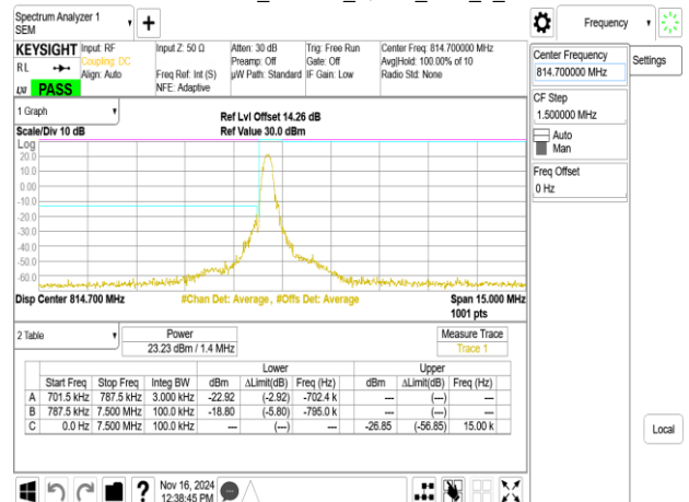
Band26-Part90s_1.4MHz_QPSK_RB1_0_CH26697
