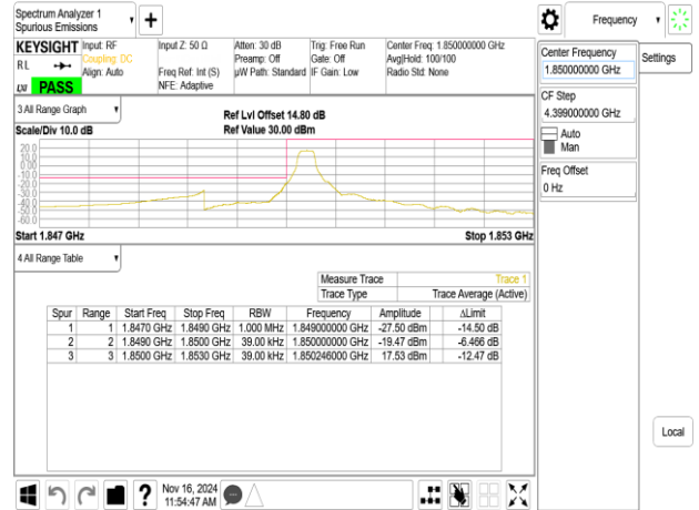
Band25_3MHz_QPSK_RB15_0_CH26055
