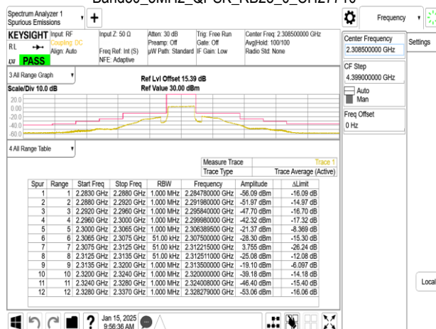
Band30_5MHz_QPSK_RB1_0_CH27735
