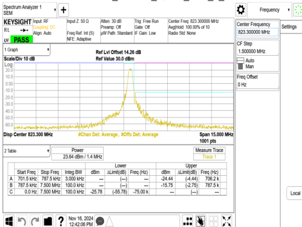
Band26-Part90s_1.4MHz_QPSK_RB6_0_CH26783
