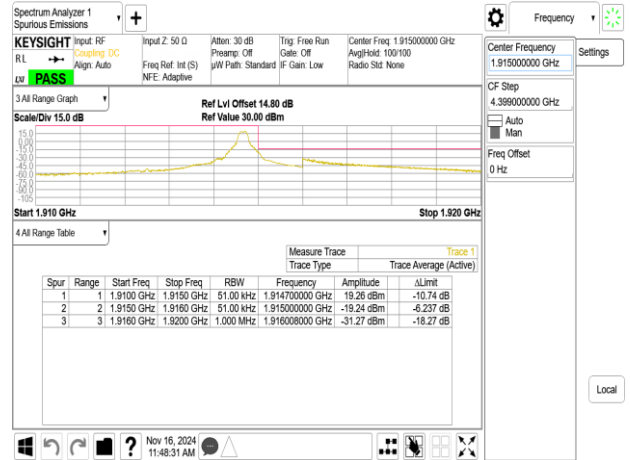
Band25_5MHz_QPSK_RB25_0_CH26665
