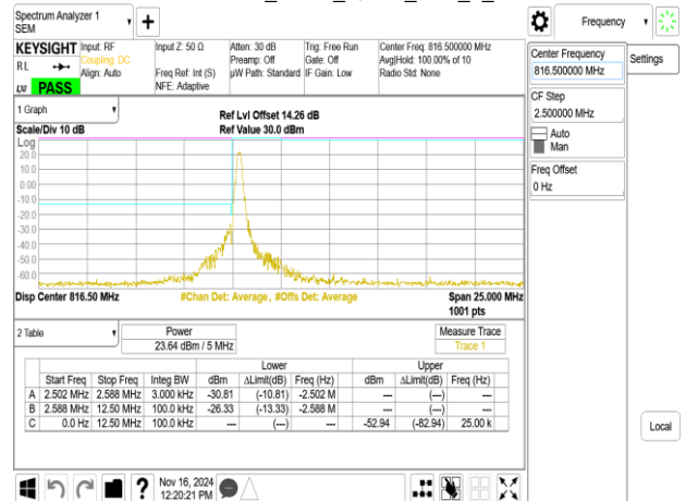
Band26-Part90s_5MHz_QPSK_RB25_0_CH26715
