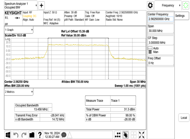
Band7_15MHz_64QAM_RB75_0_CH21375
