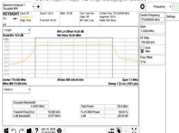
Band13_5MHz_64QAM_RB25_0_CH23205
