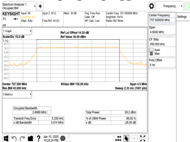
Band12_3MHz_256QAM_RB15_0_CH23095
