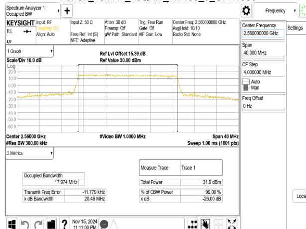
Band7_20MHz_64QAM_RB100_0_CH21350
