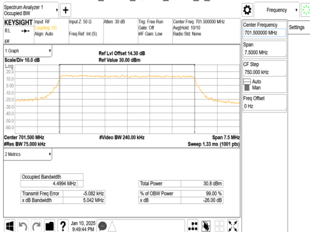
Band12_5MHz_16QAM_RB25_0_CH23035
