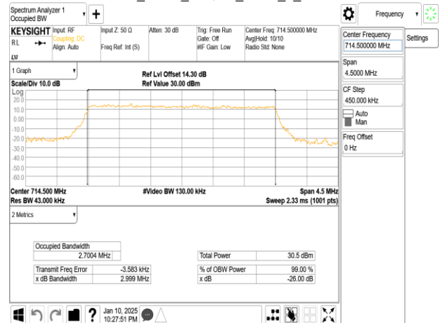
Band12_3MHz_64QAM_RB15_0_CH23165
