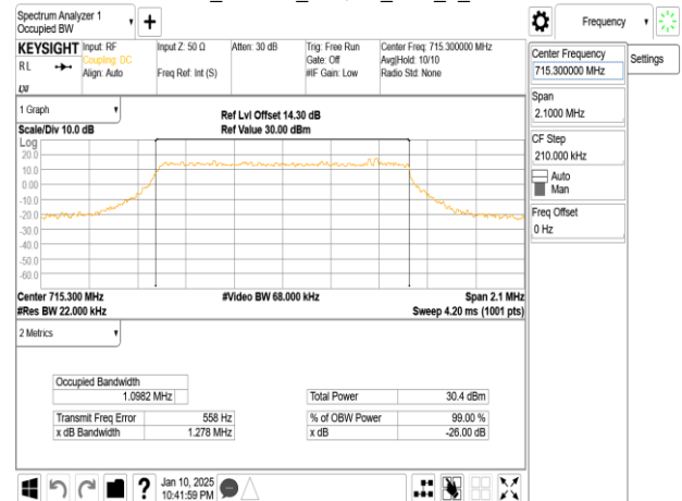
Band12_1.4MHz_64QAM_RB6_0_CH23173
