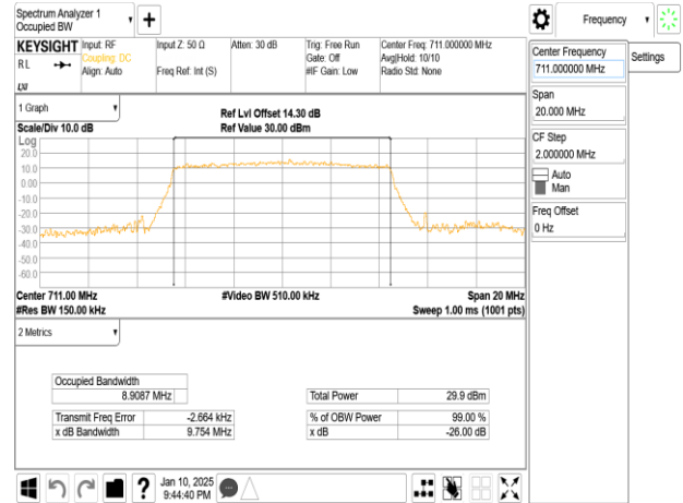
Band12_10MHz_256QAM_RB50_0_CH23130
