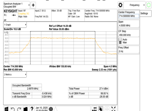
Band12_3MHz_256QAM_RB15_0_CH23165
