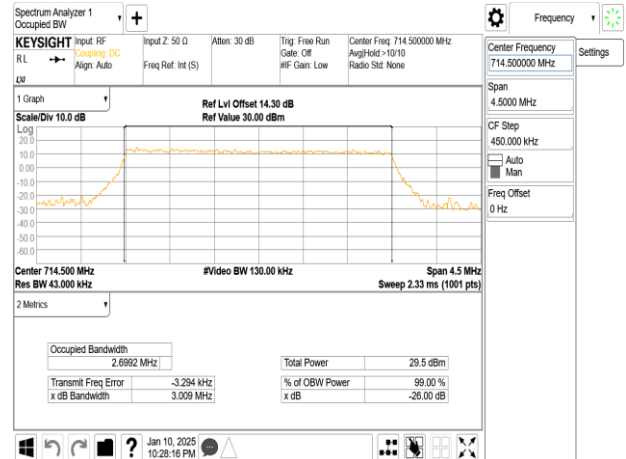
Band12_3MHz_256QAM_RB15_0_CH23165
