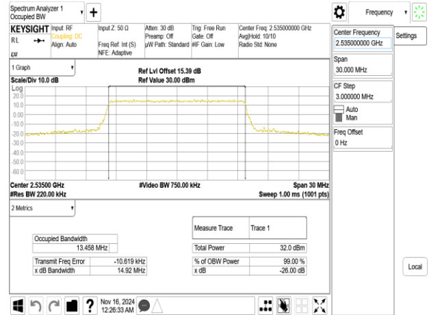
Band7_15MHz_16QAM_RB75_0_CH21100
