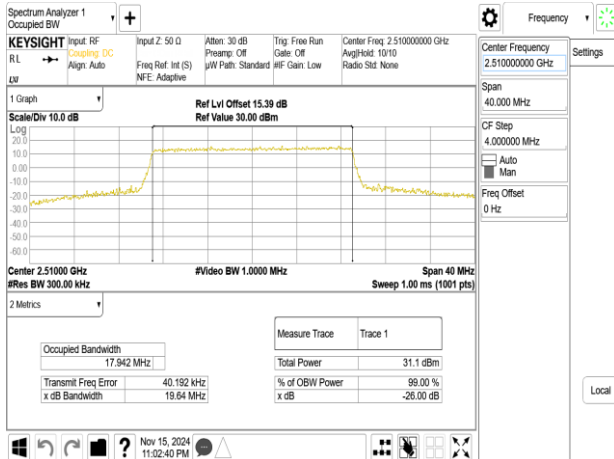
Band7_20MHz_64QAM_RB100_0_CH20850
