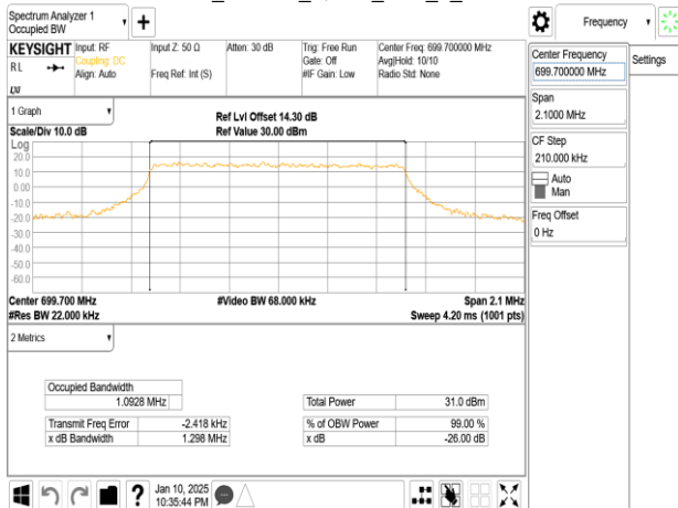
Band12_1.4MHz_16QAM_RB6_0_CH23017
