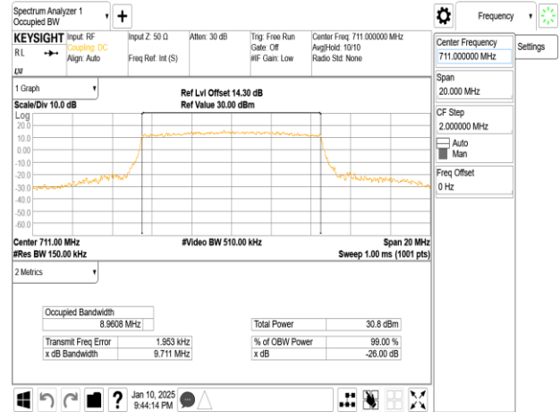
Band12_10MHz_64QAM_RB50_0_CH23130
