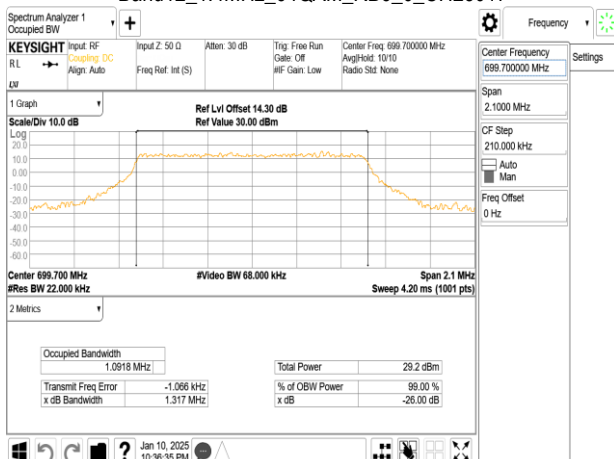
Band12_1.4MHz_64QAM_RB6_0_CH23017
