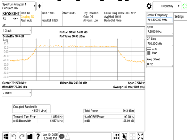
Band12_5MHz_64QAM_RB25_0_CH23035
