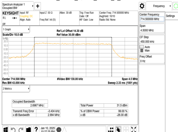
Band12_3MHz_QPSK_RB15_0_CH23165
