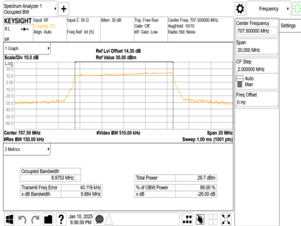
Band12_10MHz_256QAM_RB50_0_CH23095
