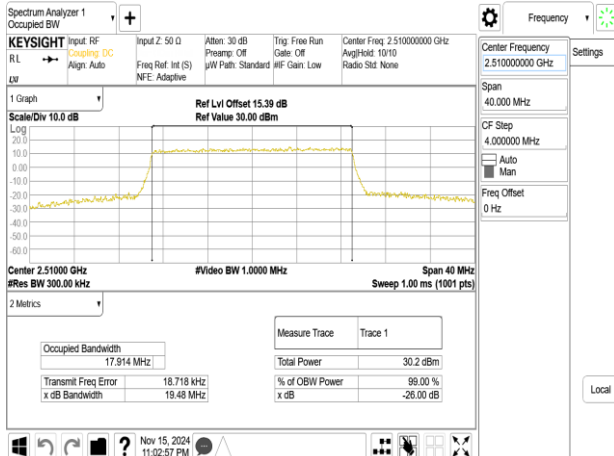
Band7_20MHz_64QAM_RB100_0_CH20850
