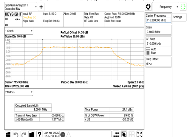
Band12_1.4MHz_256QAM_RB6_0_CH23173
