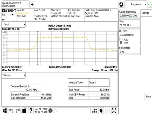
Band7_15MHz_256QAM_RB75_0_CH21100
