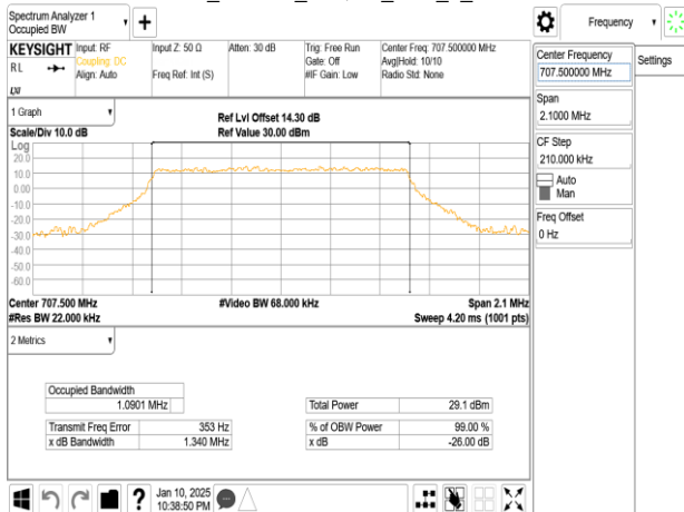
Band12_1.4MHz_256QAM_RB6_0_CH23095
