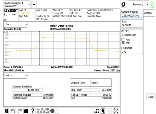
Band7_15MHz_256QAM_RB75_0_CH21375
