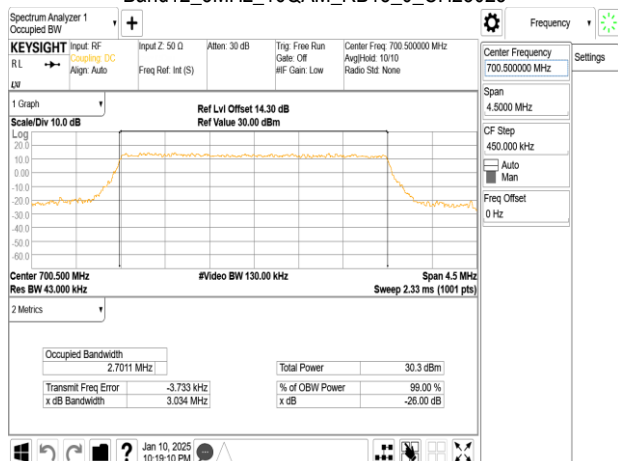
Band12_3MHz_64QAM_RB15_0_CH23025
