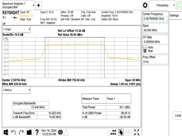
Band7_15MHz_64QAM_RB75_0_CH20825
