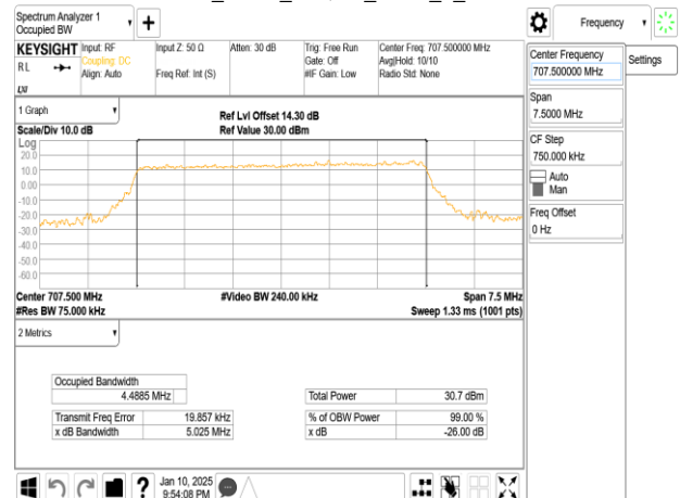
Band12_5MHz_16QAM_RB25_0_CH23095
