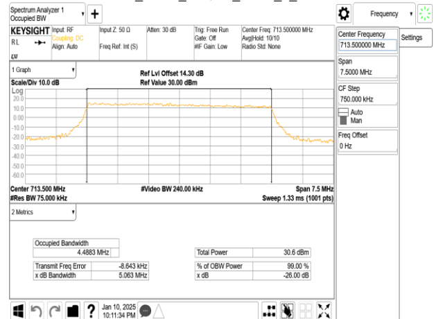
Band12_5MHz_64QAM_RB25_0_CH23155
