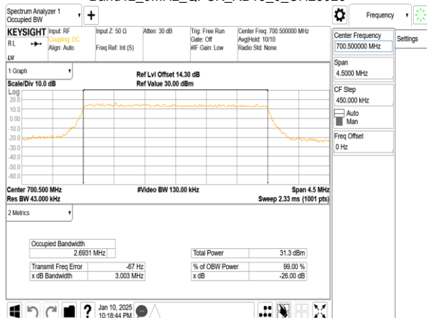
Band12_3MHz_16QAM_RB15_0_CH23025
