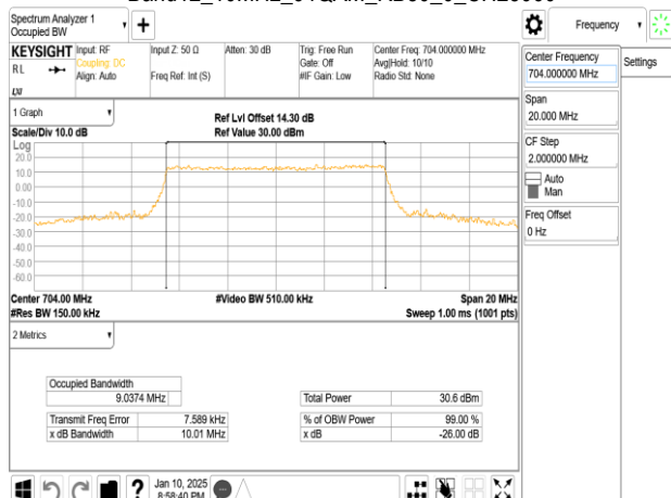
Band12_10MHz_64QAM_RB50_0_CH23060
