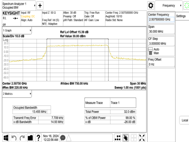
Band7_15MHz_16QAM_RB75_0_CH20825
