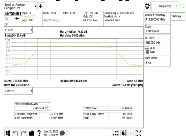
Band12_5MHz_256QAM_RB25_0_CH23155
