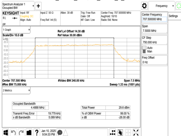
Band12_5MHz_256QAM_RB25_0_CH23095
