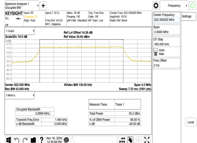
Band26-Part90s_3MHz_16QAM_RB15_0_CH26775
