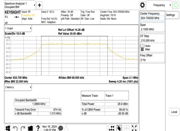
Band26_1.4MHz_256QAM_RB6_0_CH26797
