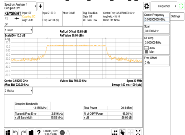
Band42-Part27_15MHz_16QAM_RB75_0_CH43015
