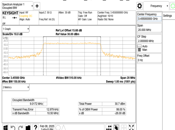
Band42-Part27_10MHz_QPSK_RB50_0_CH42140
