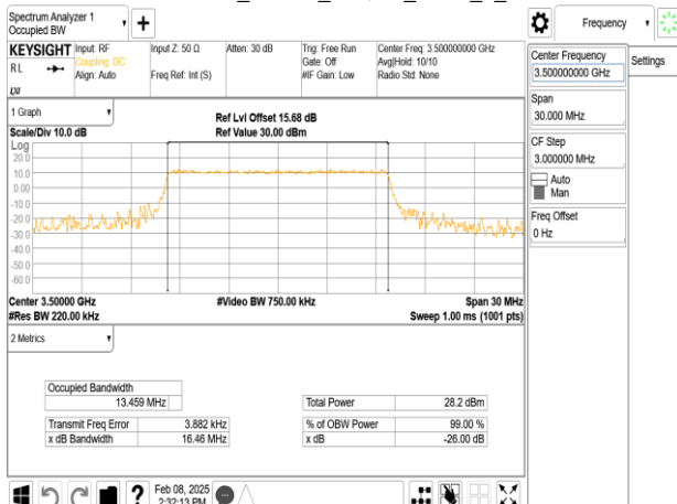
Band42-Part27_15MHz_64QAM_RB75_0_CH42590
