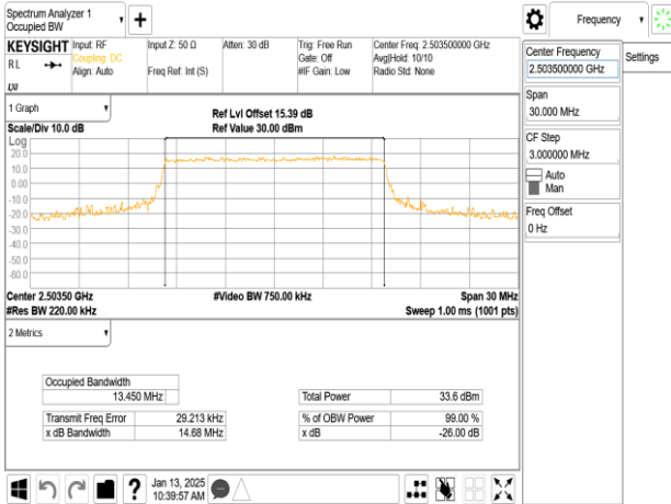
Band41_15MHz_16QAM_RB75_0_CH39725
