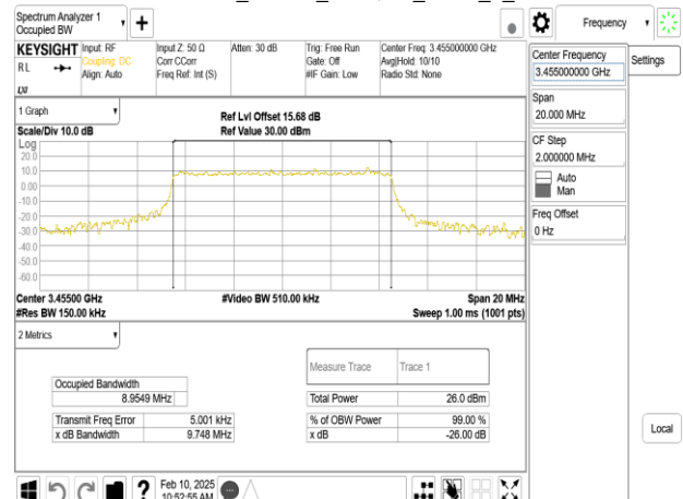
Band42-Part27_10MHz_256QAM_RB50_0_CH42140
