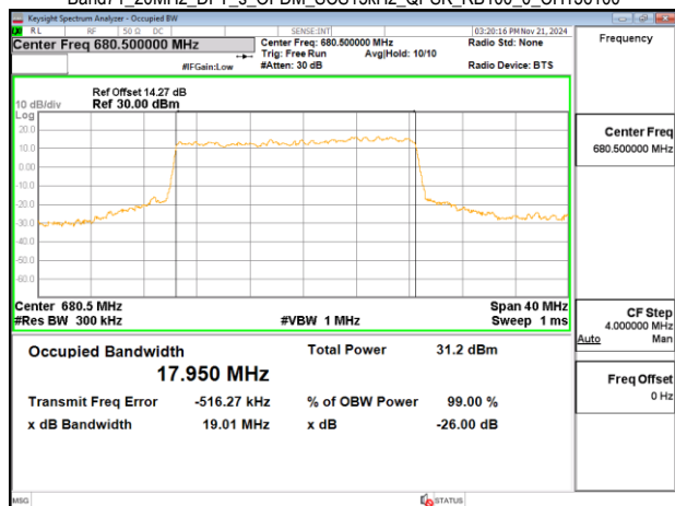
Band71_20MHz_DFT_s_OFDM_SCS15kHz_QPSK_RB100_0_CH136100
