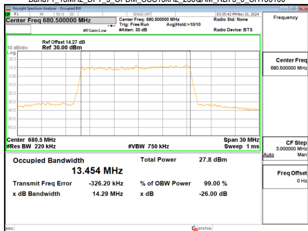
Band71_15MHz_DFT_s_OFDM_SCS15kHz_256QAM_RB75_0_CH136100
