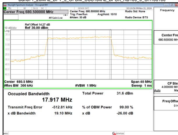
Band71_20MHz_DFT_s_OFDM_SCS15kHz_BPSK_RB100_0_CH136100
