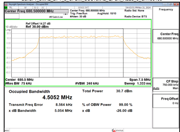
Band71_5MHz_DFT_s_OFDM_SCS15kHz_QPSK_RB25_0_CH136100
