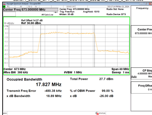
Band71_20MHz_DFT_s_OFDM_SCS15kHz_256QAM_RB100_0_CH136100
