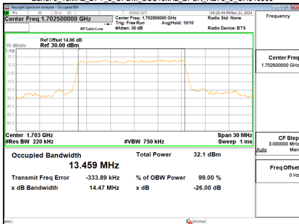
Band70_15MHz_DFT_s_OFDM_SCS15kHz_BPSK_RB75_0_CH340500
