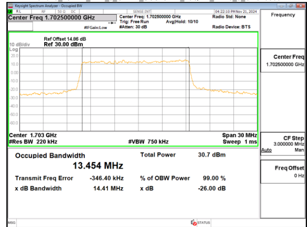
Band70_15MHz_DFT_s_OFDM_SCS15kHz_64QAM_RB75_0_CH340500
