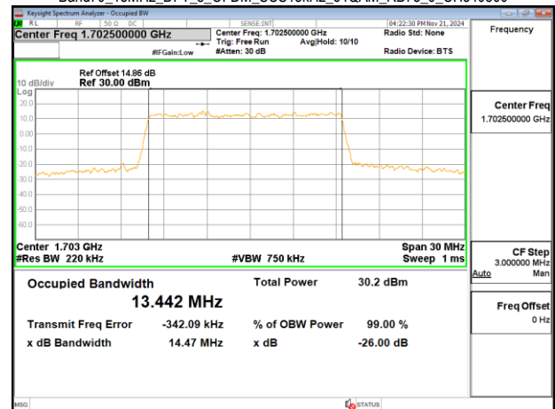
Band70_15MHz_DFT_s_OFDM_SCS15kHz_64QAM_RB75_0_CH340500
