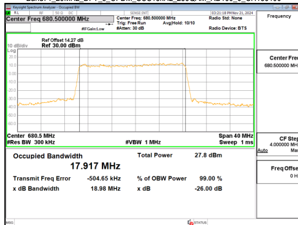
Band71_20MHz_DFT_s_OFDM_SCS15kHz_256QAM_RB100_0_CH136100
