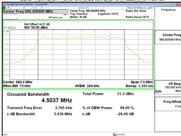
Band71_5MHz_DFT_s_OFDM_SCS15kHz_BPSK_RB25_0_CH136100
