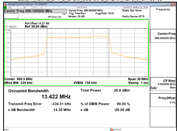
Band71_15MHz_DFT_s_OFDM_SCS15kHz_64QAM_RB75_0_CH136100
