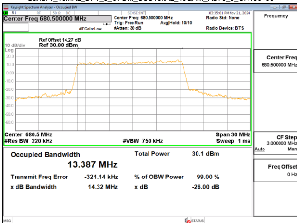
Band71_15MHz_DFT_s_OFDM_SCS15kHz_16QAM_RB75_0_CH136100
