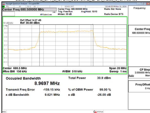
Band71_10MHz_DFT_s_OFDM_SCS15kHz_QPSK_RB50_0_CH136100
