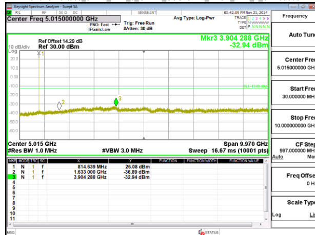
Band26-Part90s_5MHz_DFT_s_OFDM_SCS15kHz_BPSK_RB1_1_CH163300
