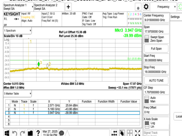
Band38_20MHz_DFT_s_OFDM_SCS30kHz_BPSK_RB1_1_CH516000 below 18G
