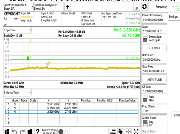
Band30_10MHz_DFT_s_OFDM_SCS30kHz_BPSK_RB1_1_CH515000 below 18G
