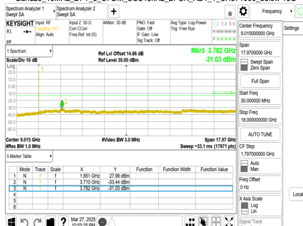
Band25_10MHz_DFT_s_OFDM_SCS15kHz_BPSK_RB1_1_CH371000_below 18G
