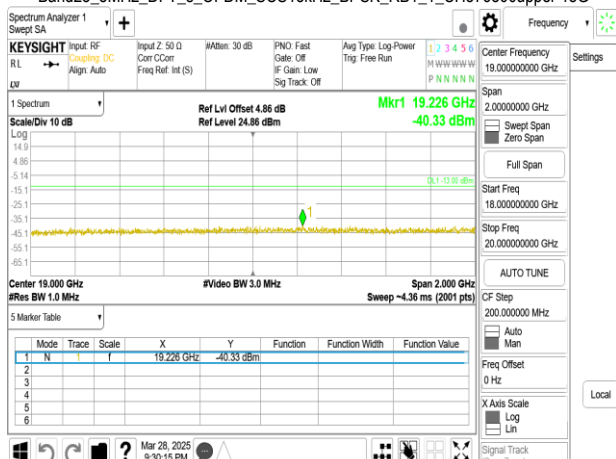
Band25_5MHz_DFT_s_OFDM_SCS15kHz_BPSK_RB1_1_CH376500upper 18G
