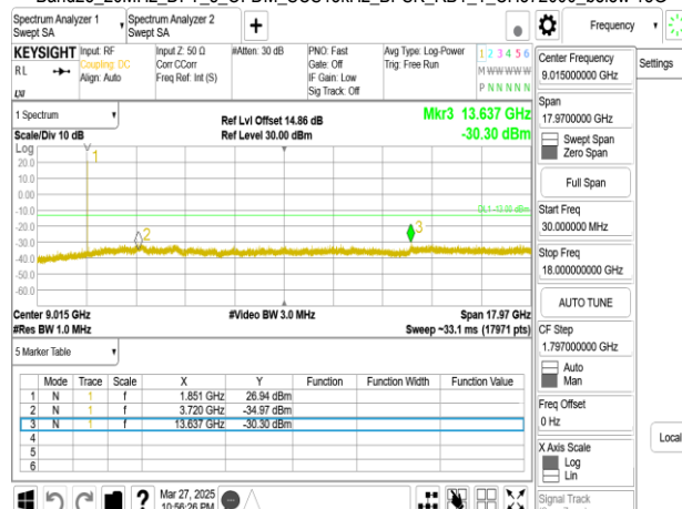
Band25_20MHz_DFT_s_OFDM_SCS15kHz_BPSK_RB1_1_CH372000 below 18G
