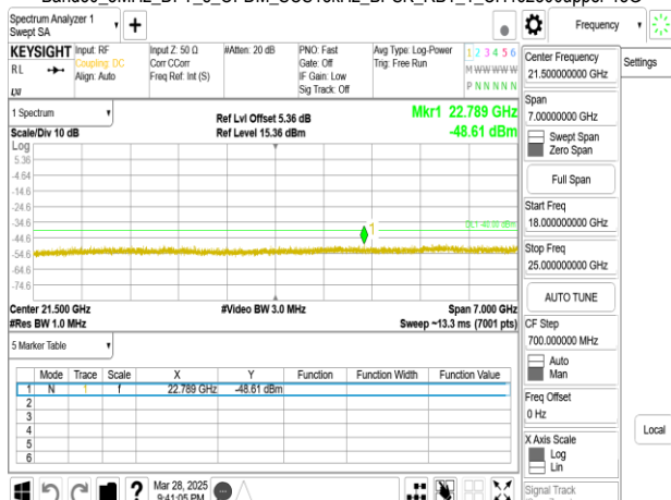
Band30_5MHz_DFT_s_OFDM_SCS15kHz_BPSK_RB1_1_CH462500upper 18G
