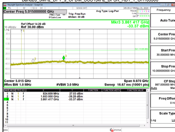
Band26 5MHz DFT s OFDM_SCS15kHz BPSK RB1_1 CH167300
