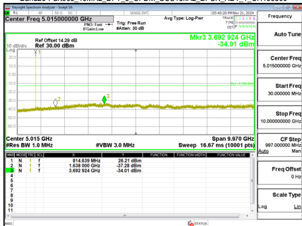
Band26-Part90s 10MHz DFT s OFDM_SCS15kHz BPSK RB1_1 CH163800
