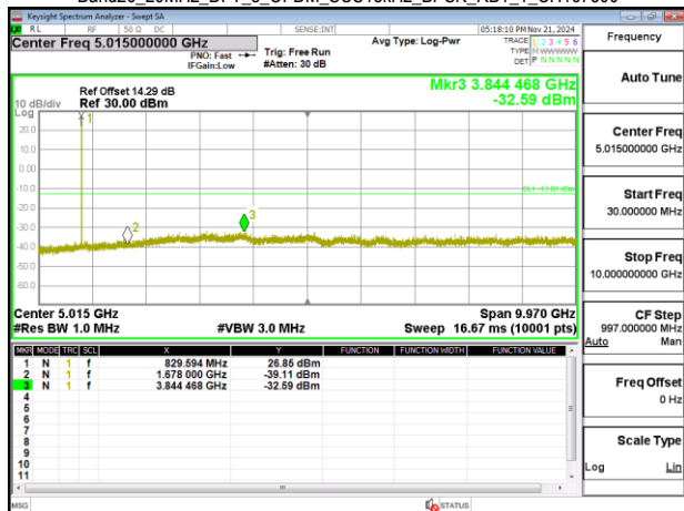
Band26_20MHz_DFT_s_OFDM_SCS15kHz_BPSK_RB1_1_CH167800
