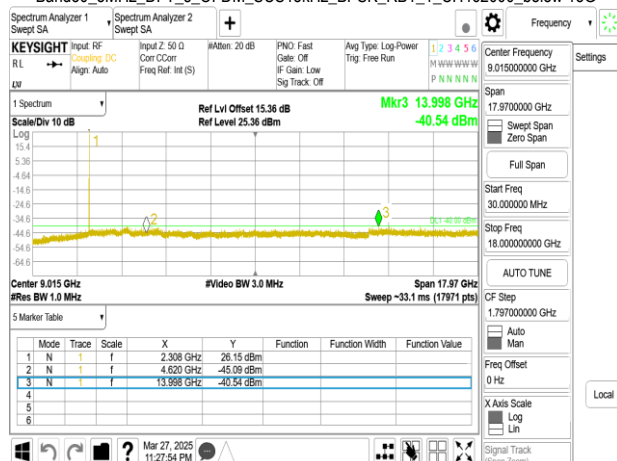
Band30_5MHz_DFT_s_OFDM_SCS15kHz_BPSK_RB1_1_CH462000_below 18G
