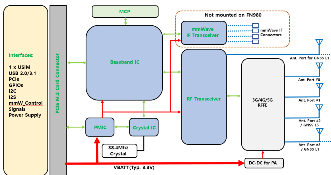
FN980 Family Block Diagram
