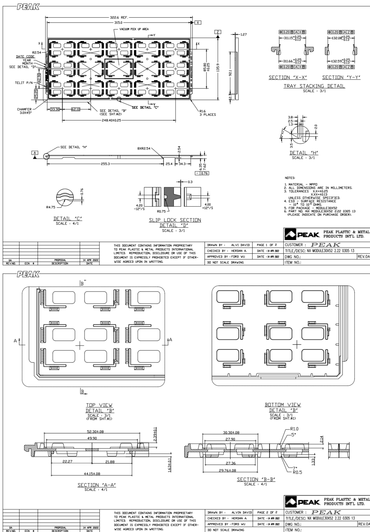
Figure 25: Tray Construction
