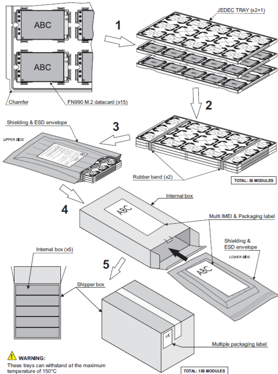
Figure 23: Tray Packaging
