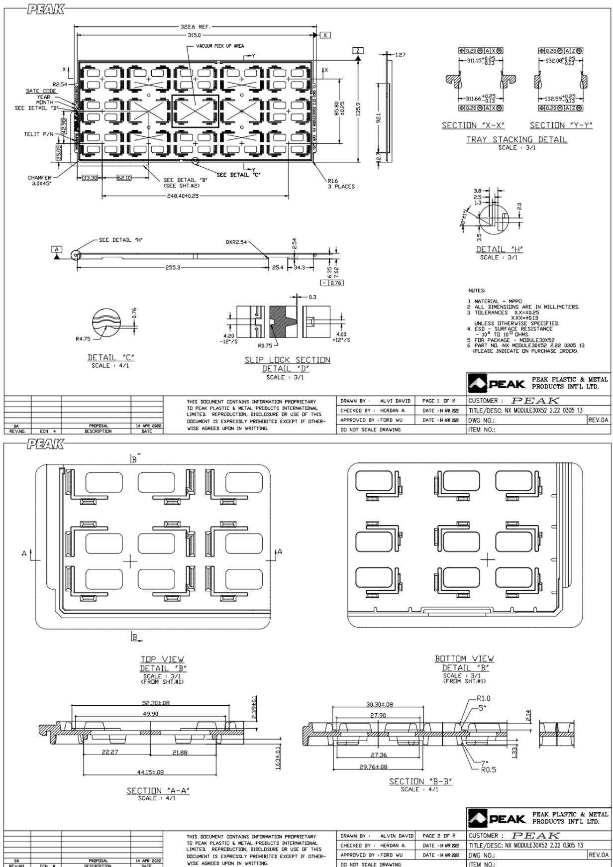
Figure 24: Tray Construction
