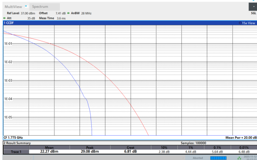
Band 66-10M-HIGH-16QAM-1RB Low
