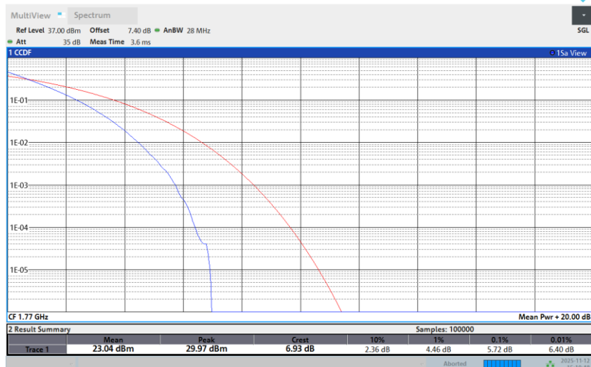
Band 66-20M-HIGH-16QAM-1RB Low
