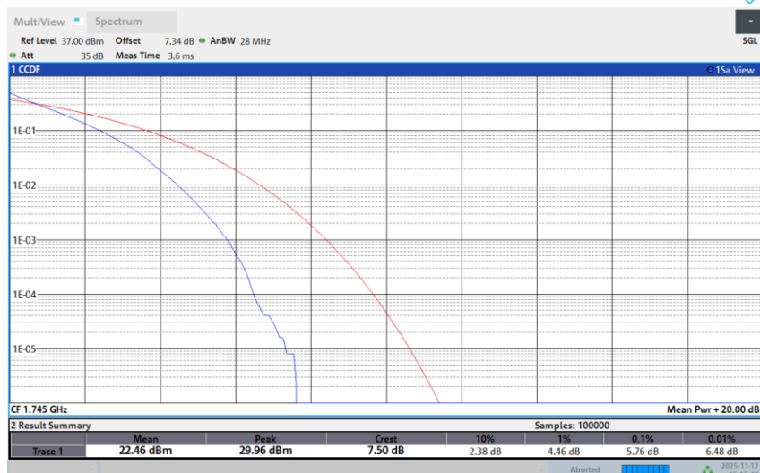
Band 66-10M-MID-16QAM-1RB Low
