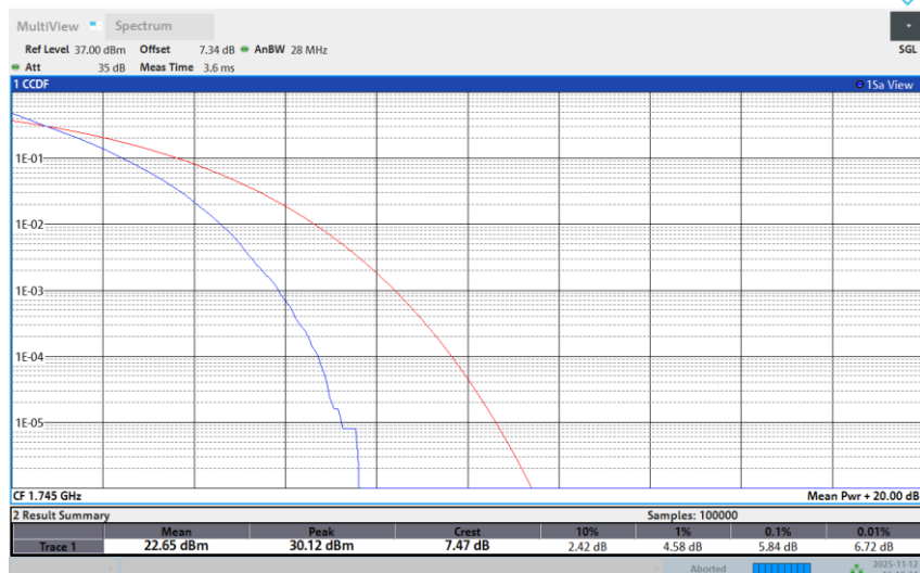
Band 66-20M-MID-16QAM-1RB Low
