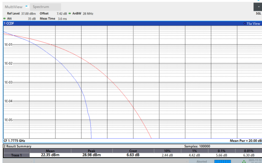
Band 66-5M-HIGH-16QAM-1RB Low
