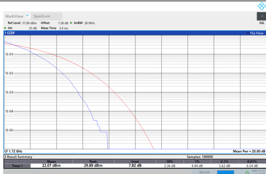
Band 66-20M-LOW-16QAM-1RB Low
