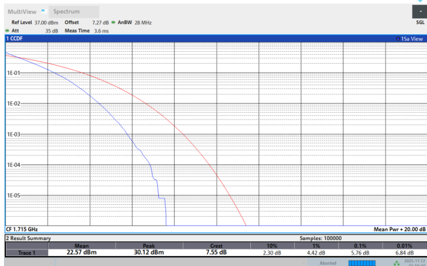
Band 66-10M-LOW-16QAM-1RB Low
