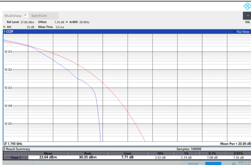
Band 66-10M-MID-16QAM-Full RB
