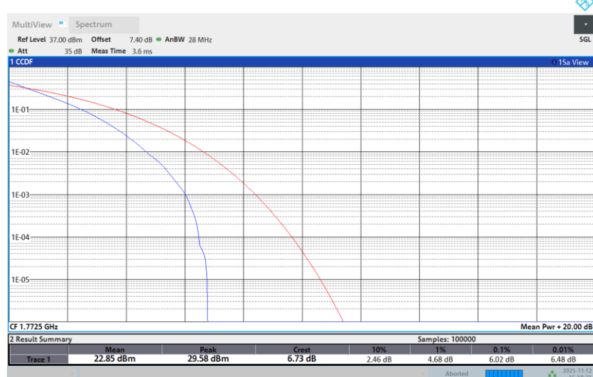
Band 66-15M-HIGH-16QAM-1RB Low
