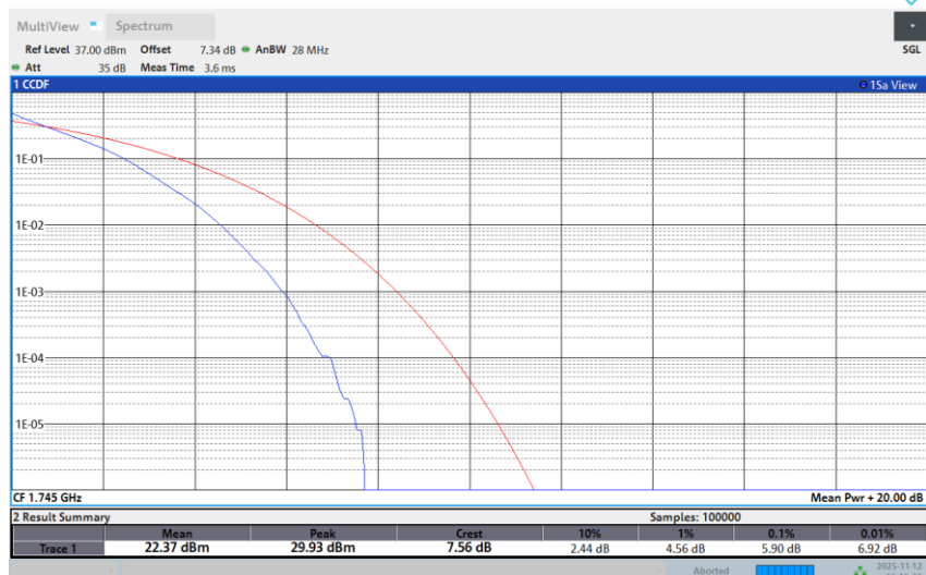
Band 66-5M-MID-16QAM-1RB Low
