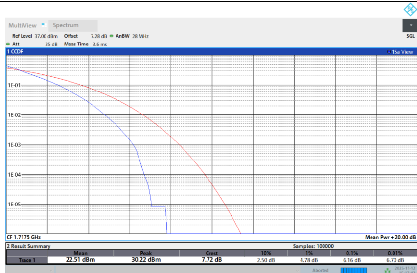
Band 66-15M-LOW-16QAM-1RB Low
