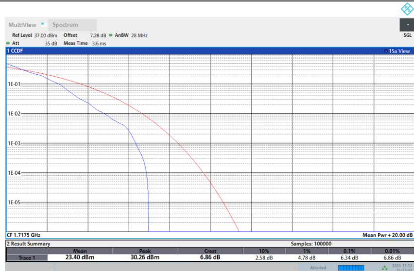
Band 66-15M-LOW-QPSK-Full RB
