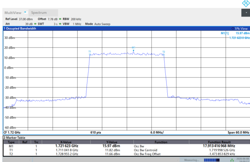
Band 66-20M-LOW-16QAM-Full RB
