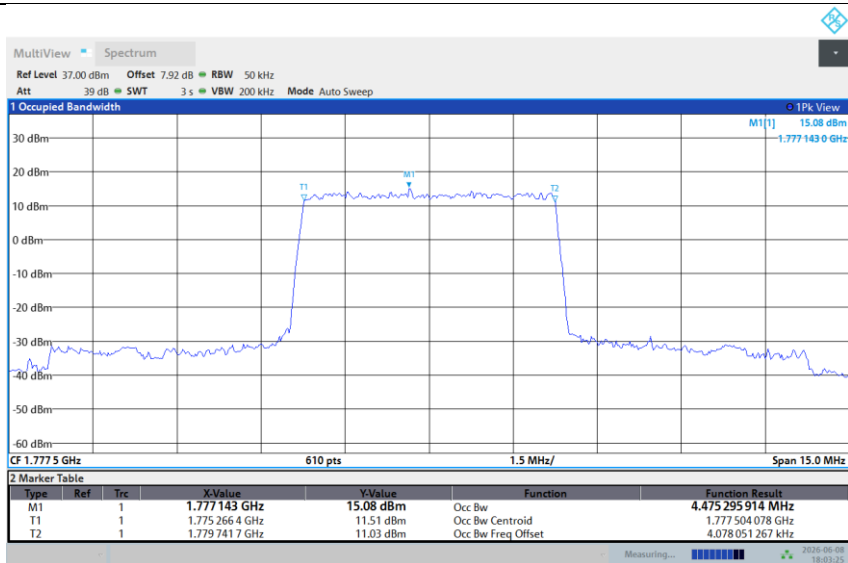
Band 66-5M-HIGH-16QAM-Full RB
