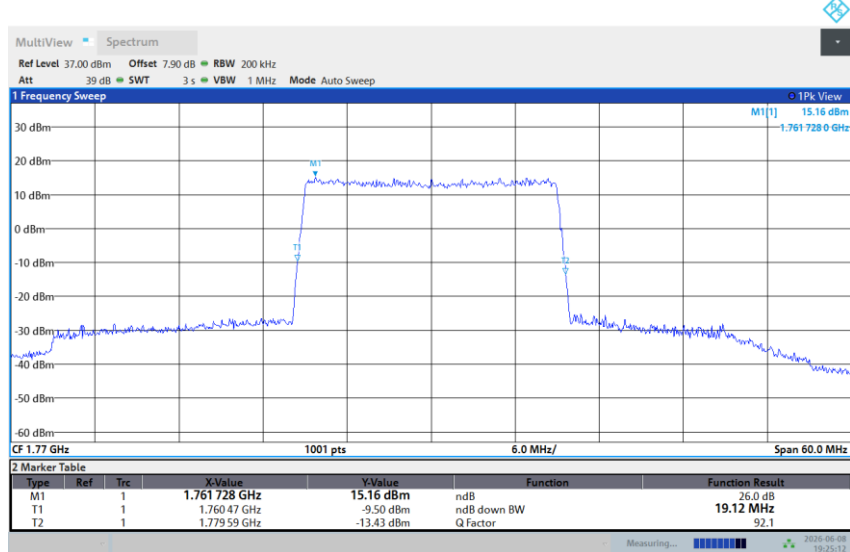
Band 66-20M-HIGH-16QAM-Full RB
