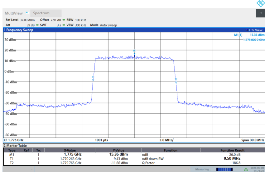
Band 66-10M-HIGH-16QAM-Full RB
