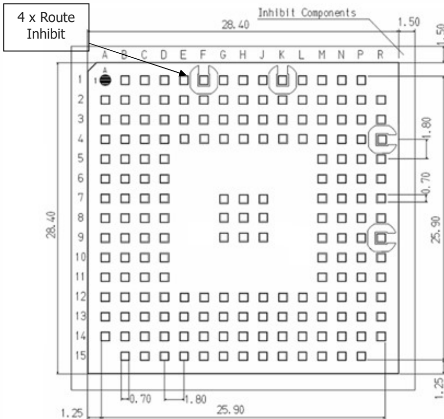
Figure 26: Recommended Footprint - Top View, 181 pads
