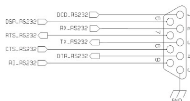
Figure 14: RS232 Serial Port Lines Connection Layout
