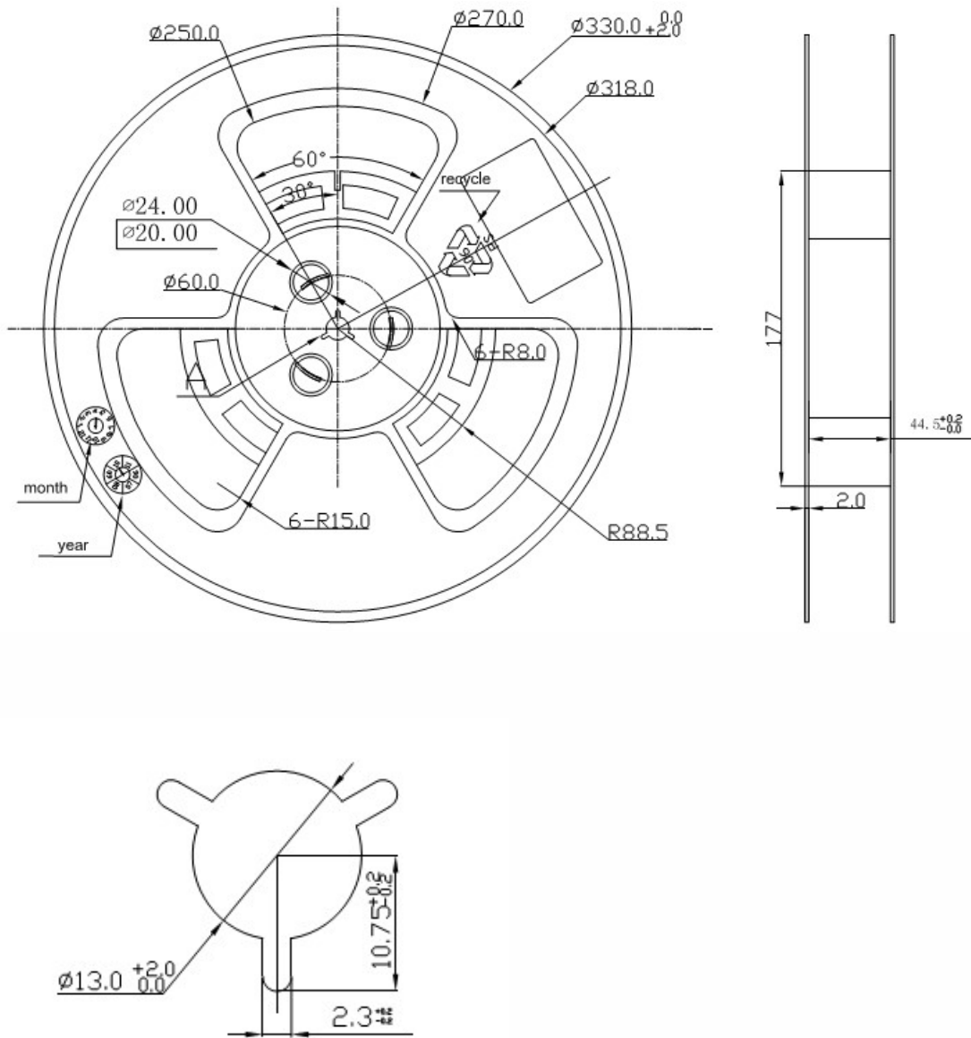
Figure 35: Reel Detail
