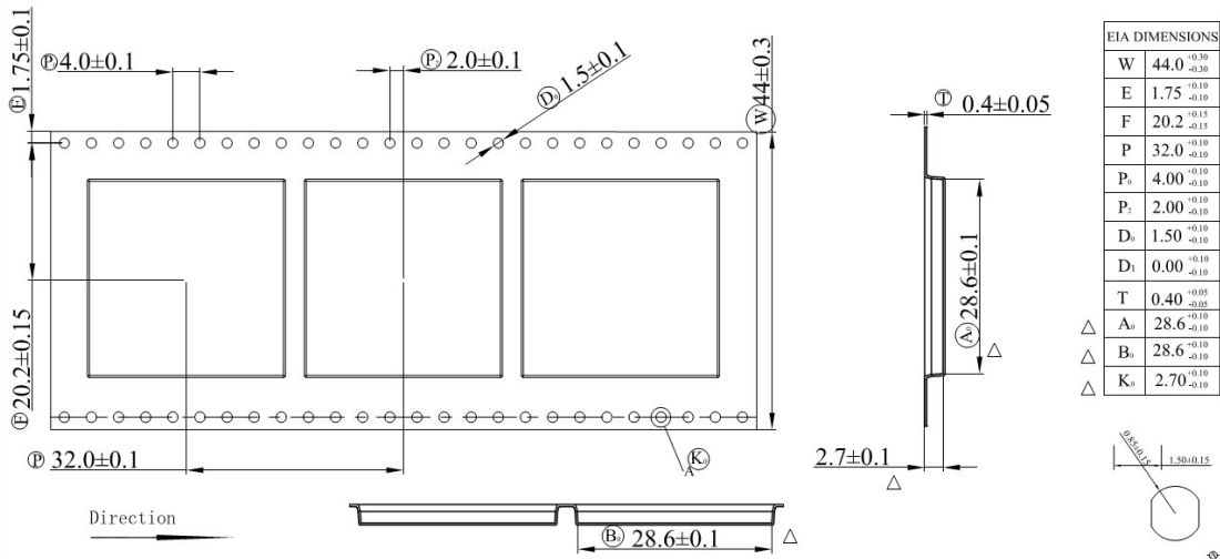
Figure 34: Carrier Tape Detail
