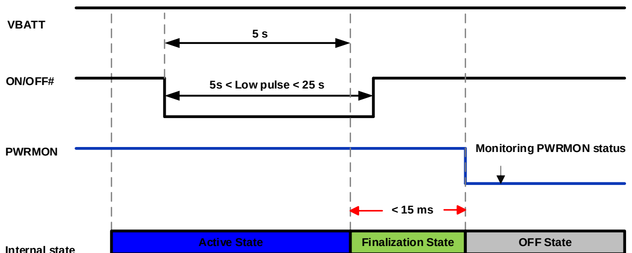
Figure 8: Hardware Shutdown
