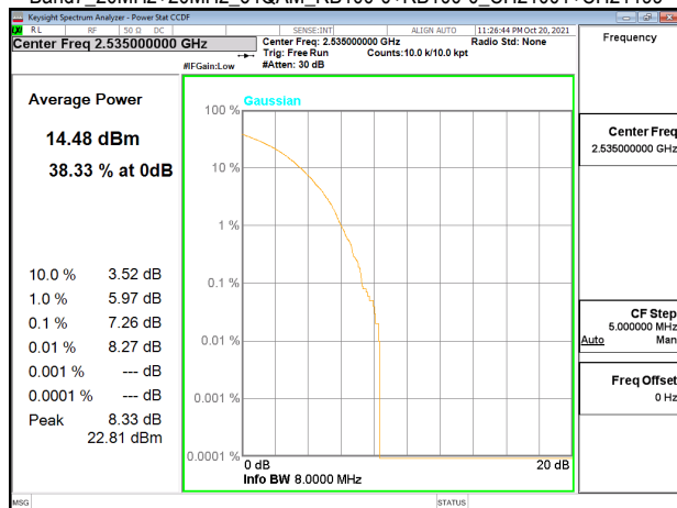
Band7_20MHz+20MHz_64QAM_RB100-0+RB100-0_CH21001+CH21199
