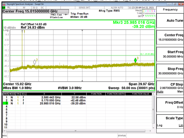
Band38_15MHz+15MHz_QPSK_RB1-74_1-0_CH37925-38075
