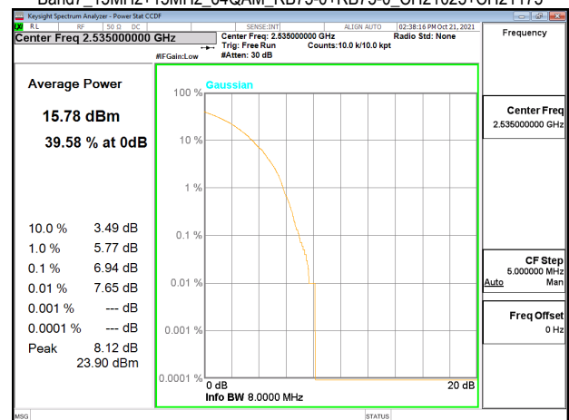
Band7_15MHz+15MHz_64QAM_RB75-0+RB75-0_CH21025+CH21175
