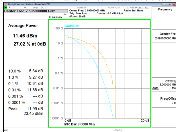
Band38_20MHz+20MHz_64QAM_RB100-0+RB100-0_CH37901+CH38099
