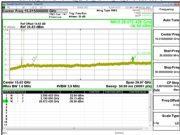
Band38_15MHz+15MHz_QPSK_RB1-74_1-0_CH38025-38175
