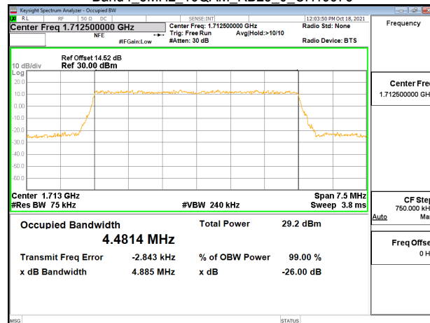
Band4_5MHz_16QAM_RB25_0_CH20175
