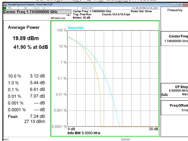
Band66_5MHz_64QAM_RB25_0_CH132322
