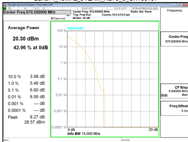
Band71_15MHz_64QAM_RB75_0_CH133297
