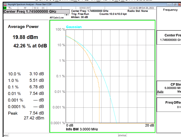
Band66_3MHz_64QAM_RB15_0_CH132322
