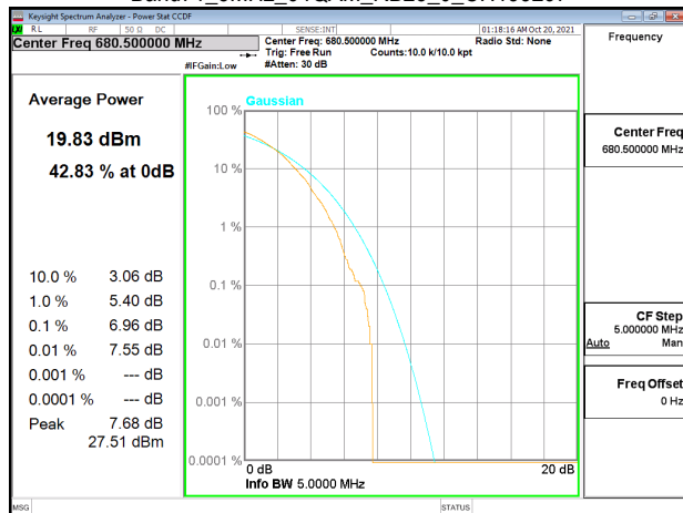
Band71_5MHz_64QAM_RB25_0_CH133297
