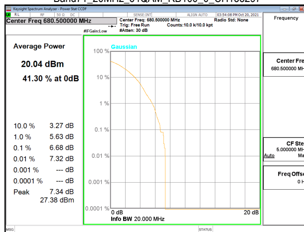
Band71_20MHz_64QAM_RB100_0_CH133297
