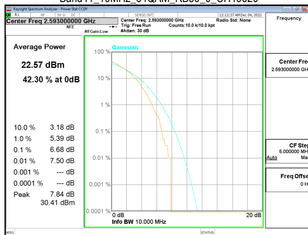
Band41_10MHz_64QAM_RB50_0_CH40620
