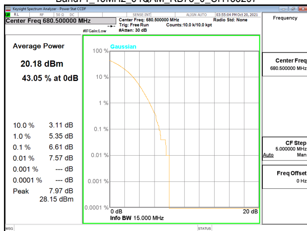
Band71_15MHz_64QAM_RB75_0_CH133297
