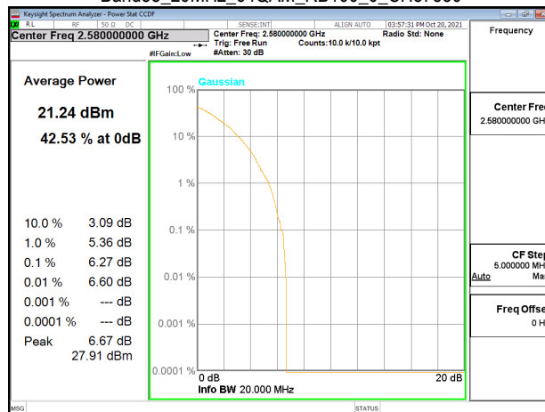
Band38_20MHz_64QAM_RB100_0_CH38000
