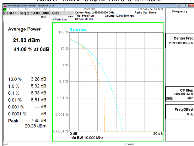
Band41_15MHz_64QAM_RB75_0_CH40620
