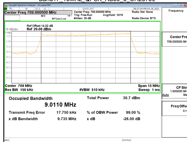
Band17_10MHz_QPSK_RB50_0_CH23790
