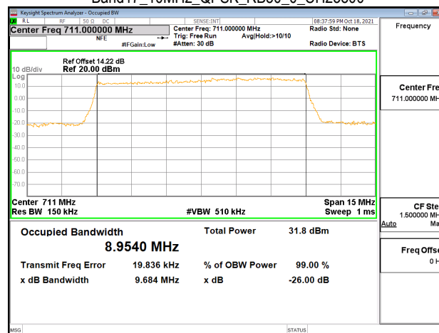
Band17_10MHz_QPSK_RB50_0_CH23800
