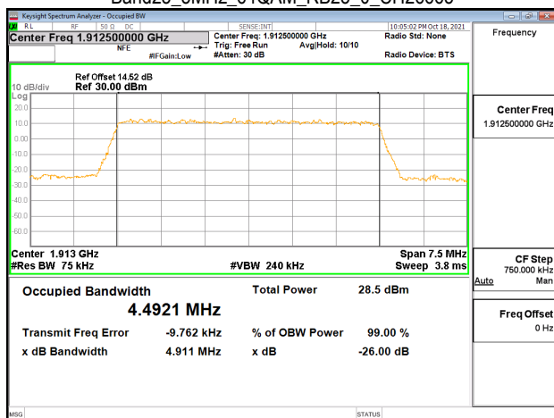
Band25_5MHz_64QAM_RB25_0_CH26665
