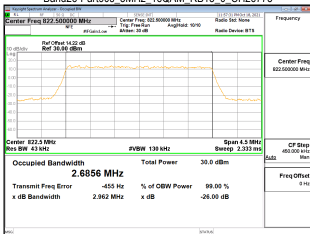
Band26-Part90s_3MHz_16QAM_RB15_0_CH26775
