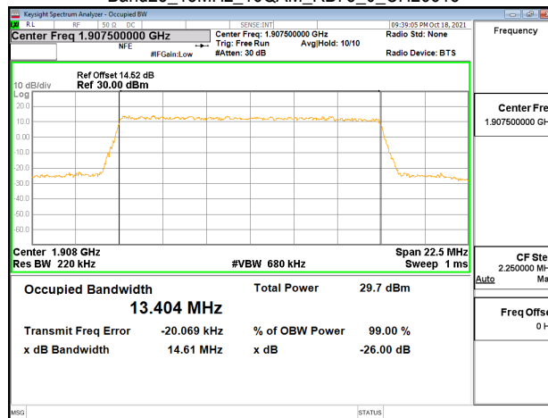
Band25 15MHz 16QAM RB75_0_CH26615
