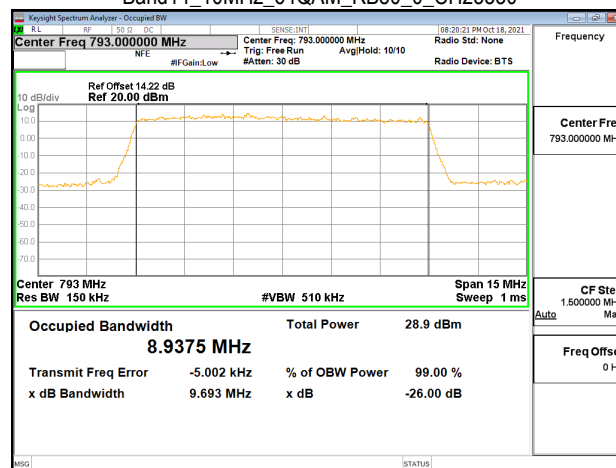
Band14_10MHz_64QAM_RB50_0_CH23330
