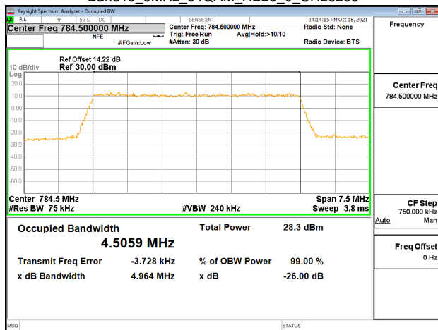
Band13_5MHz_64QAM_RB25_0_CH23255
