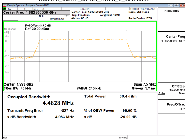
Band25_5MHz_QPSK_RB25_0_CH26665
