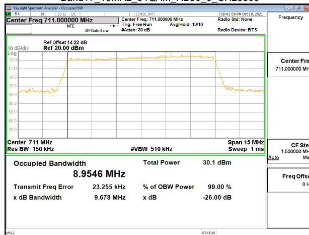
Band17_10MHz_64QAM_RB50_0_CH23800
