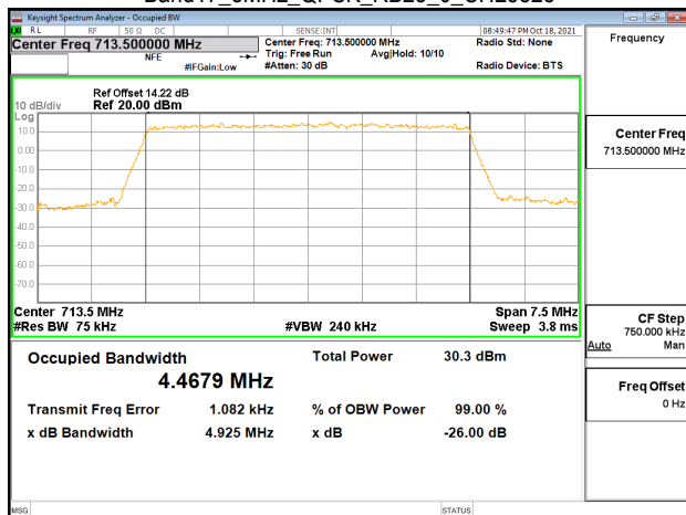
Band17_5MHz_QPSK_RB25_0_CH23825
