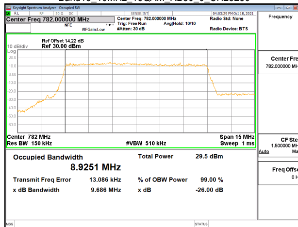
Band13_10MHz_64QAM_RB50_0_CH23230
