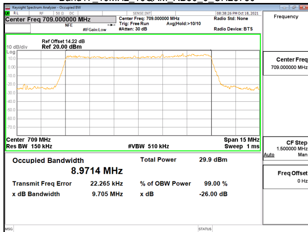
Band17_10MHz_16QAM_RB50_0_CH23790
