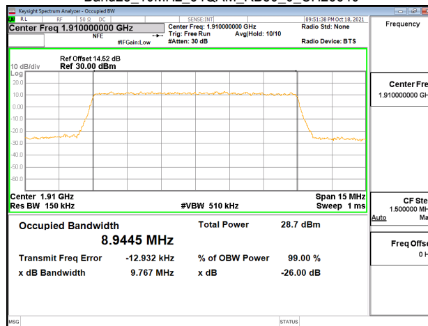
Band25_10MHz_64QAM_RB50_0_CH26640
