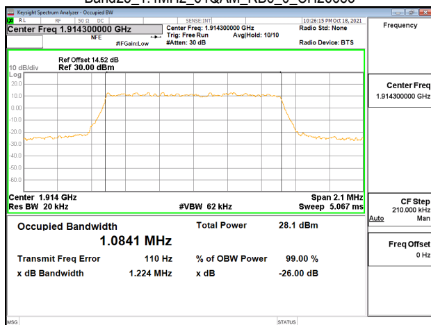
Band25_1.4MHz_64QAM_RB6_0_CH26683
