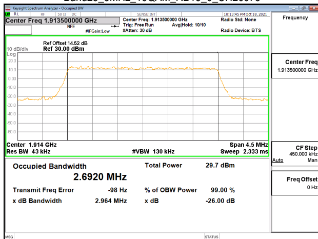
Band25_3MHz_16QAM_RB15_0_CH26675
