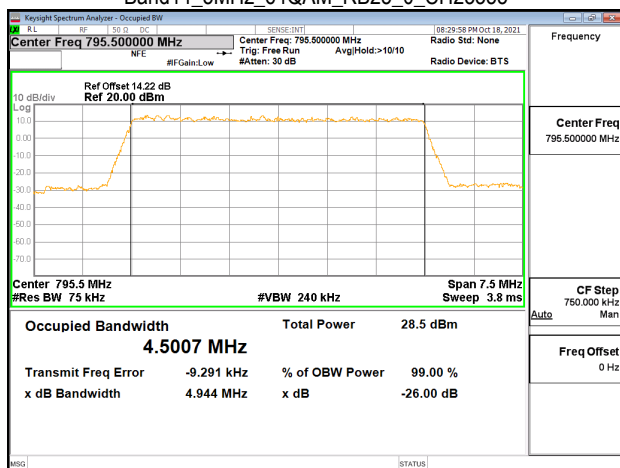
Band14_5MHz_64QAM_RB25_0_CH23355
