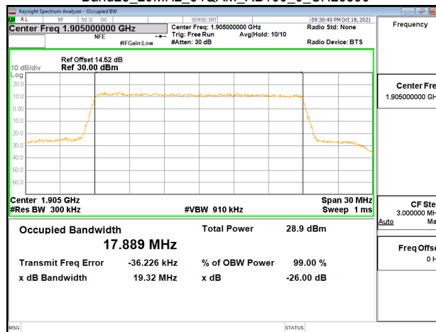
Band25_20MHz_64QAM_RB100_0_CH26590
