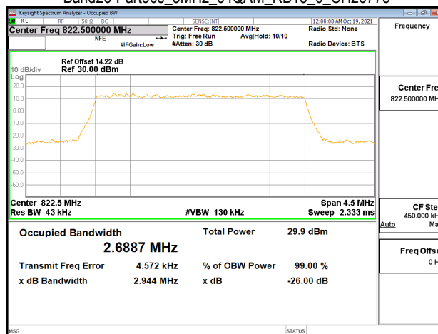
Band26-Part90s_3MHz_64QAM_RB15_0_CH26775
