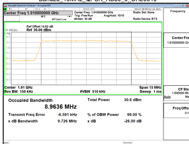
Band25_10MHz_QPSK_RB50_0_CH26640
