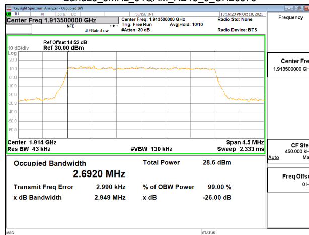
Band25_3MHz_64QAM_RB15_0_CH26675
