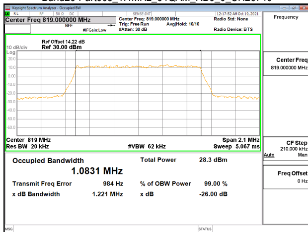
Band26-Part90s 1.4MHz 64QAM_RB6_0_CH26783
