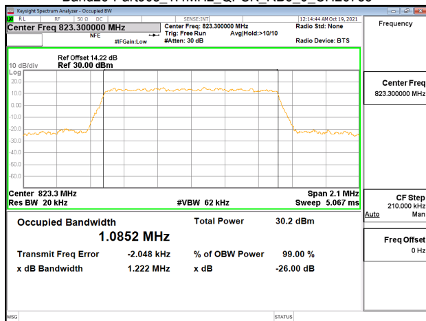
Band26-Part90s_1.4MHz_QPSK_RB6_0_CH26783
