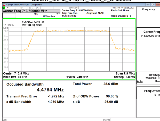
Band17_5MHz_64QAM_RB25_0_CH23825
