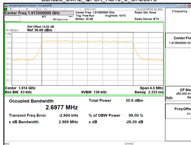
Band25_3MHz_QPSK_RB15_0_CH26675
