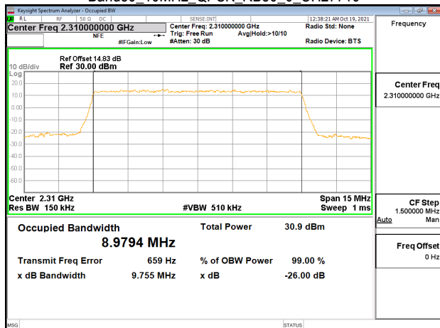
Band30_10MHz_16QAM_RB50_0_CH27710
