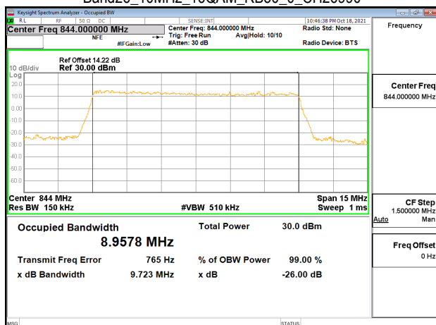
Band26_10MHz_16QAM_RB50_0_CH26990
