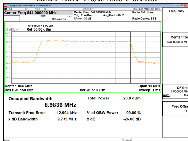
Band26_10MHz_64QAM_RB50_0_CH26990
