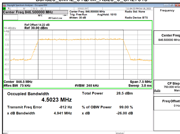
Band26_5MHz_64QAM_RB25_0_CH27015
