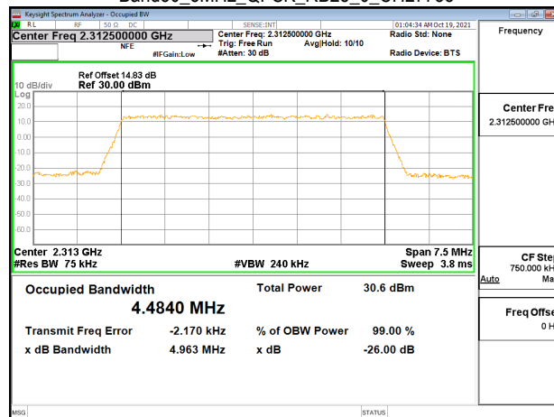
Band30_5MHz_QPSK_RB25_0_CH27735
