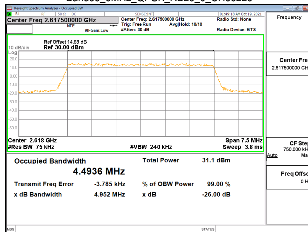
Band38_5MHz_QPSK_RB25_0_CH38225
