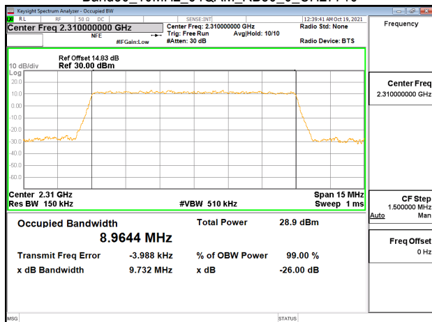
Band30_10MHz_64QAM_RB50_0_CH27710
