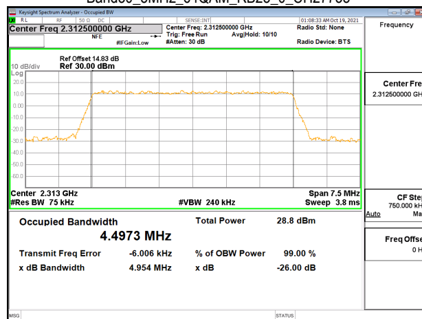
Band30 5MHz 64QAM RB25 0 CH27735
