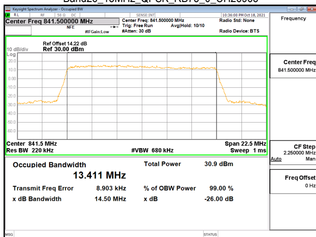
Band26_15MHz_QPSK_RB75_0_CH26965
