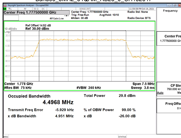
Band66_5MHz_64QAM_RB25_0_CH132647
