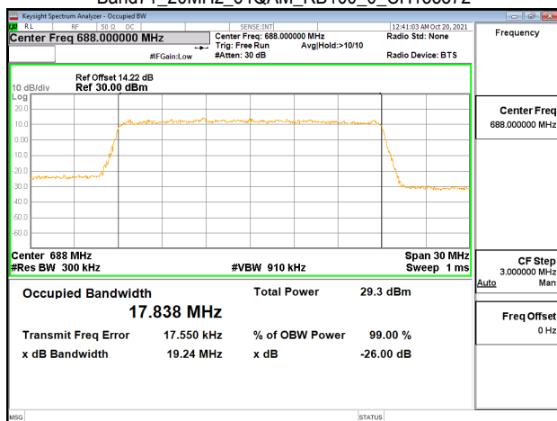
Band71_20MHz_64QAM_RB100_0_CH133372
