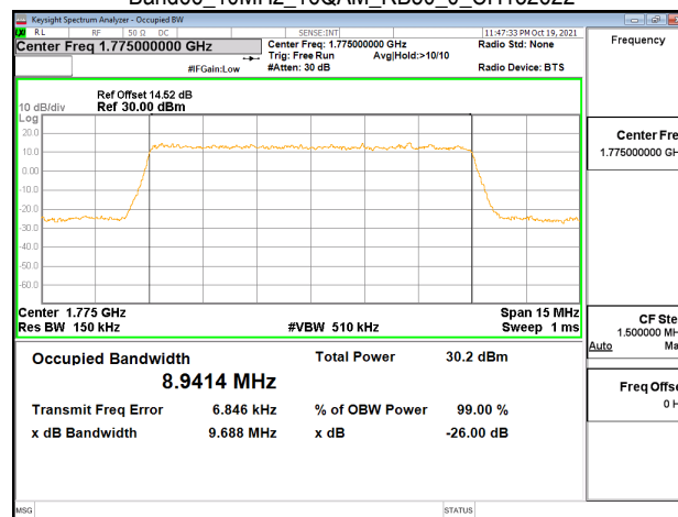
Band66_10MHz_16QAM_RB50_0_CH132622
