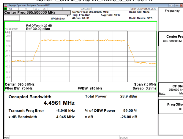
Band71_5MHz_64QAM_RB25_0_CH133447
