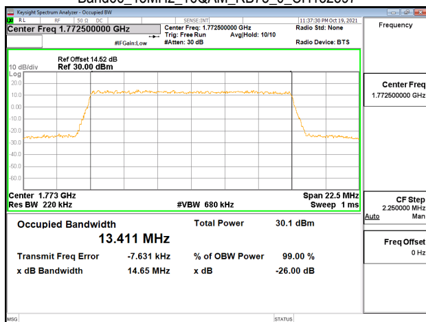
Band66_15MHz_16QAM_RB75_0_CH132597
