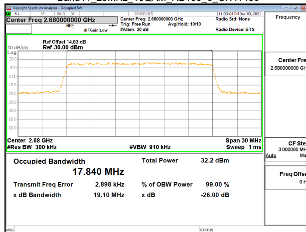
Band41_20MHz_16QAM_RB100_0_CH41490
