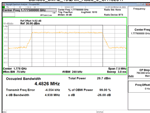
Band66_5MHz_16QAM_RB25_0_CH132647
