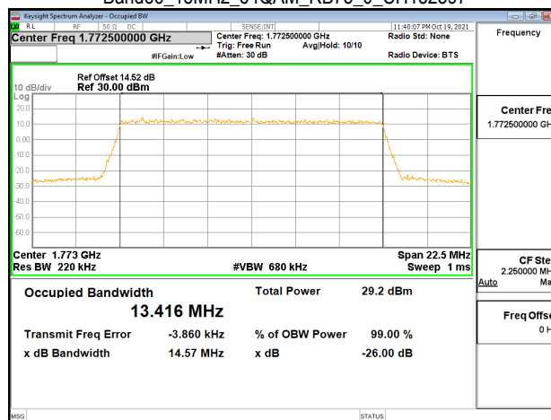
Band66_15MHz_64QAM_RB75_0_CH132597
