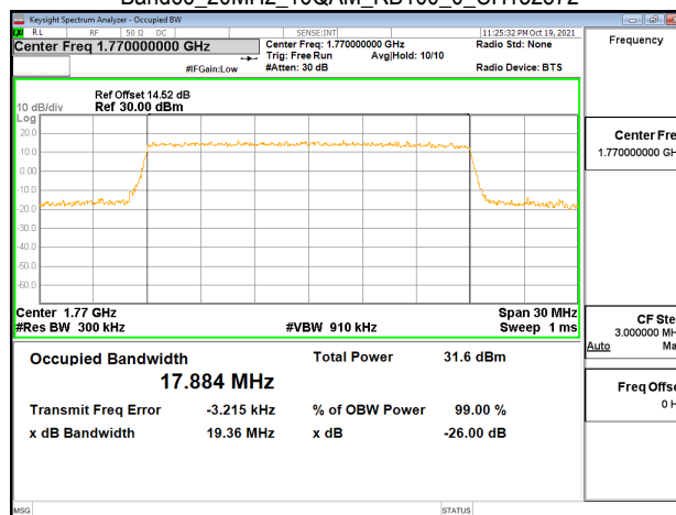
Band66_20MHz_16QAM_RB100_0_CH132572
