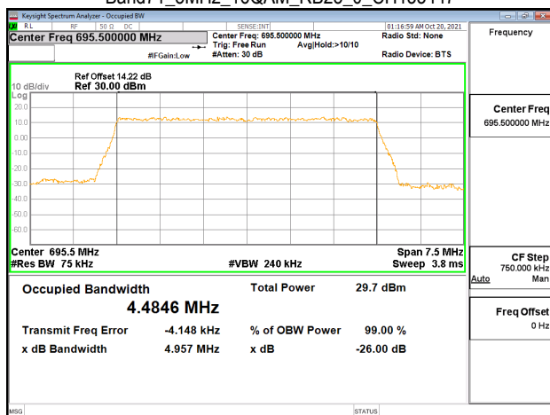
Band71_5MHz_16QAM_RB25_0_CH133447
