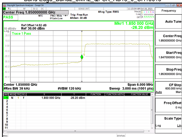
Band Edge_Band2_3MHz_QPSK_RB15_0_CH19185
