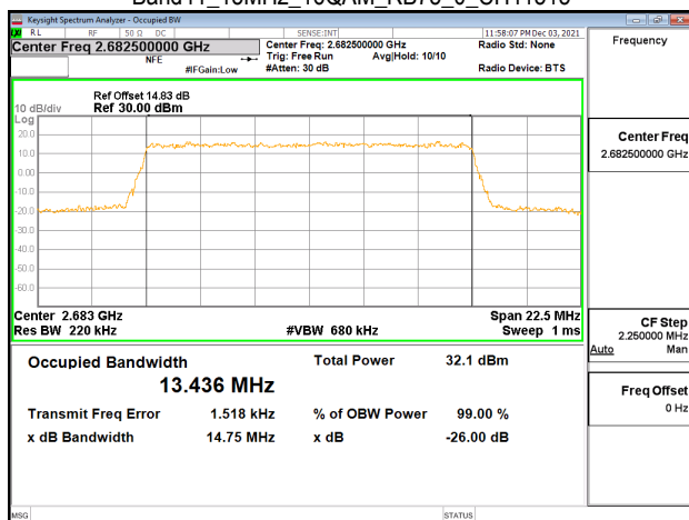
Band41_15MHz_16QAM_RB75_0_CH41515
