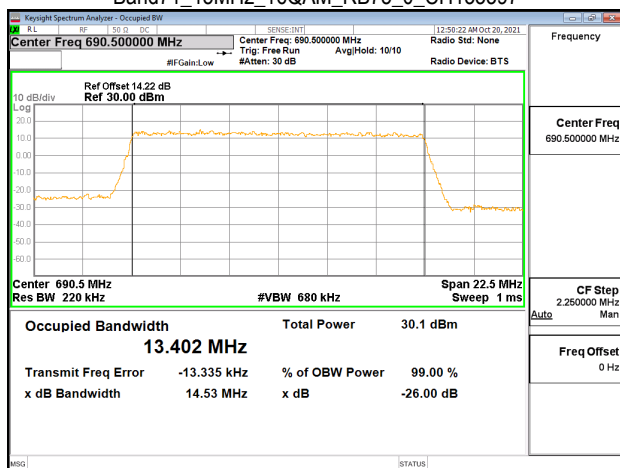
Band71_15MHz_16QAM_RB75_0_CH133397
