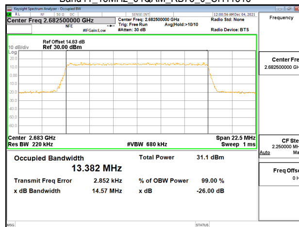
Band41_15MHz_64QAM_RB75_0_CH41515
