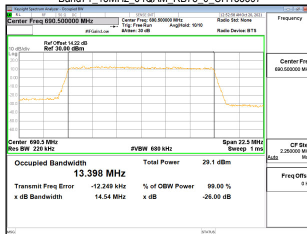
Band71_15MHz_64QAM_RB75_0_CH133397
