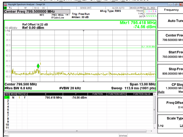
Band13_5MHz_QPSK_RB25_0_CH23205
