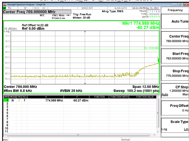
Band13_5MHz_QPSK_RB25_0_CH23255
