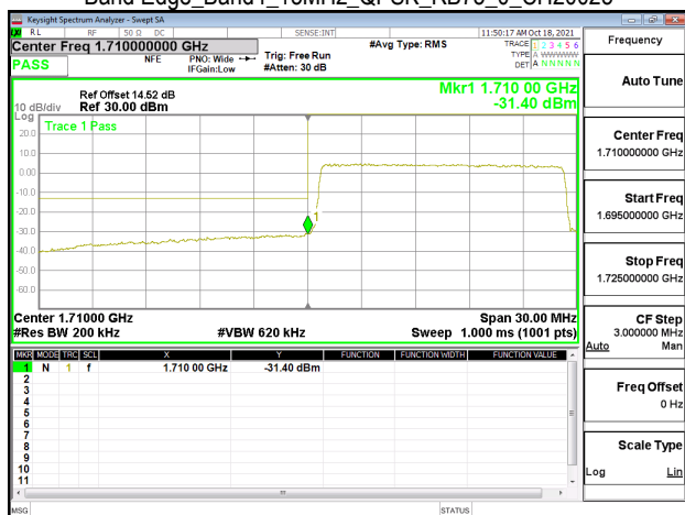
Band Edge_Band4_15MHz_QPSK_RB75_0_CH20325
