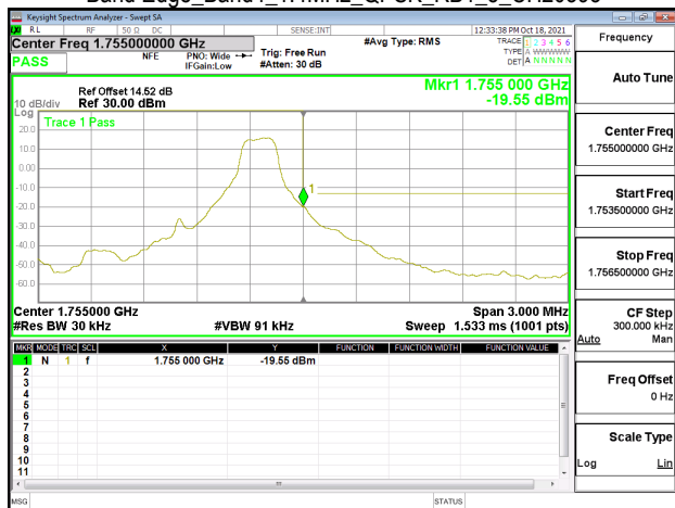
Band Edge_Band4_1.4MHz_QPSK_RB6_0_CH19957
