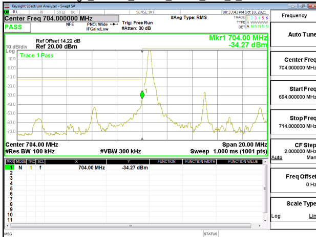
Band Edge_Band17_10MHz_QPSK_RB1_0_CH23780
