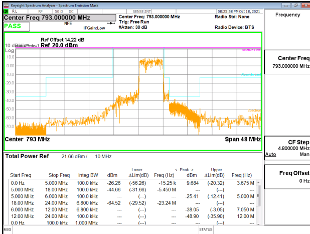
Emission Mask_Band14_10MHz_QPSK_RB1_0_CH23330
