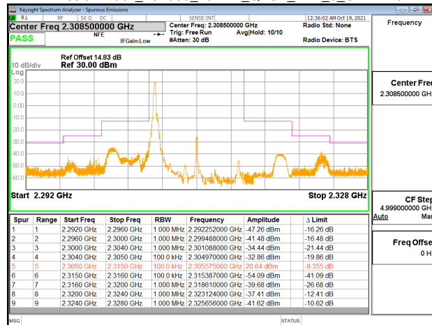
Emission Mask_Band30_10MHz_QPSK_RB1_0_CH27710
