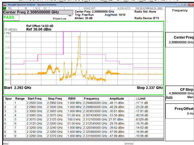
Emission Mask_Band30_5MHz_QPSK_RB1_24_CH27735
