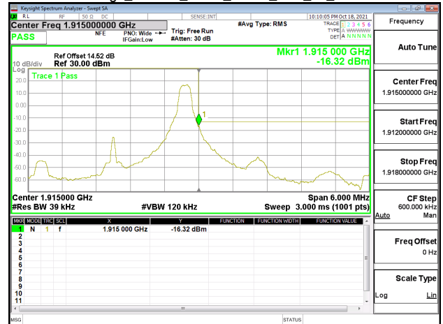
Band Edge_Band25_3MHz_QPSK_RB1_14_CH26675
