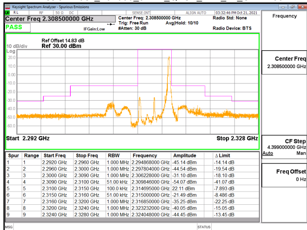
Emission Mask_Band30_5MHz_QPSK_RB25_0_CH27685
