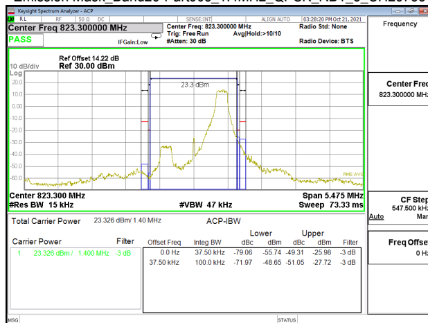
Emission Mask_Band26-Part90s_1.4MHz_QPSK_RB1_5_CH26783
