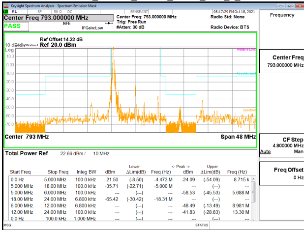
Emission Mask_Band14_10MHz_QPSK_RB1_49_CH23330
