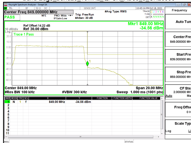
Band Edge_Band26_15MHz_QPSK_RB1_0_CH26865
