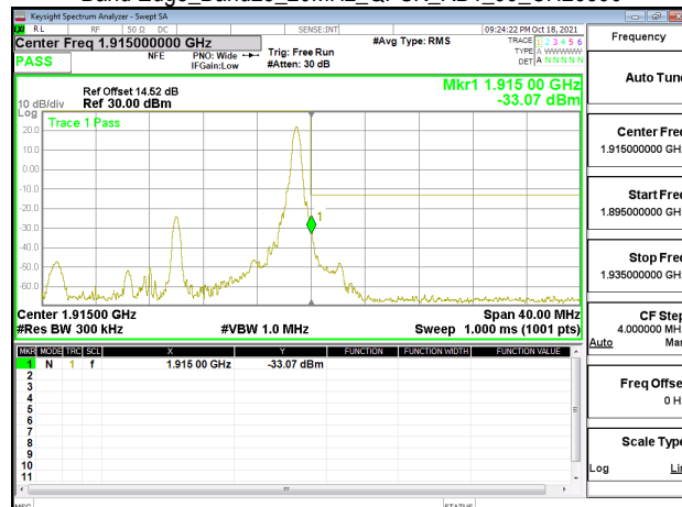
Band Edge_Band25_20MHz_QPSK_RB100_0_CH26140
