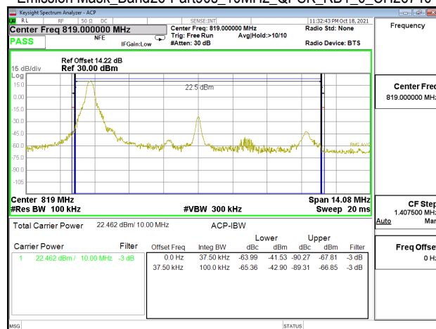
Emission Mask_Band26-Part90s_10MHz_QPSK_RB1_49_CH26740
