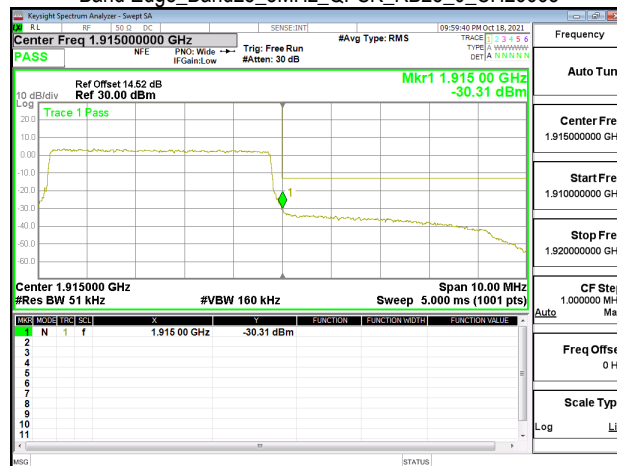
Band Edge_Band25_5MHz_QPSK_RB25_0_CH26665
