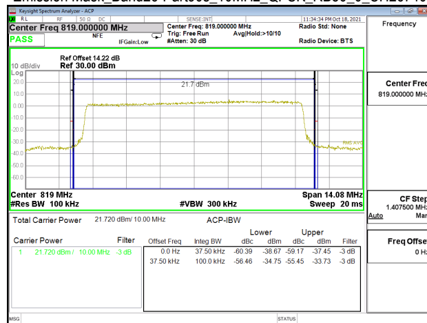
Emission Mask_Band26-Part90s_10MHz_QPSK_RB50_0_CH26740
