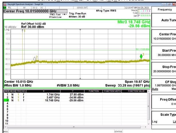
Band66_3MHz_QPSK_RB1_0_CH132657
