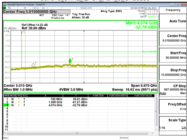
Band13_5MHz_QPSK_RB1_0_CH23255
