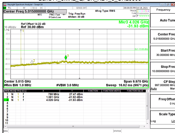
Band14_5MHz_QPSK_RB1_0_CH23330
