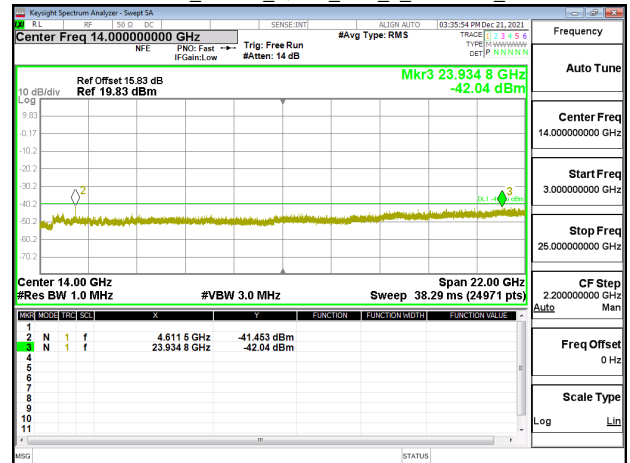
Band38_15MHz_QPSK_RB1_0_CH37825
