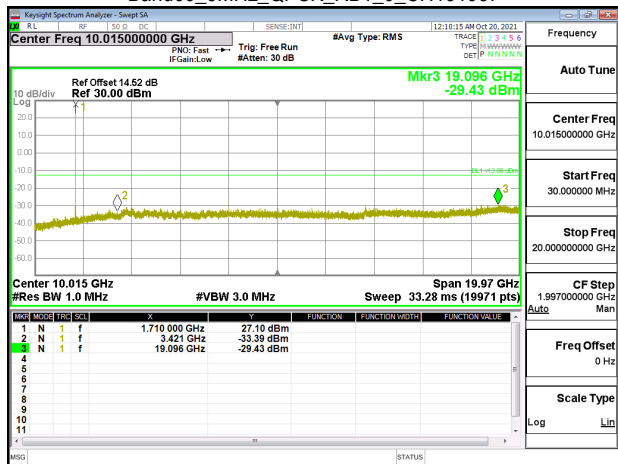
Band66_3MHz_QPSK_RB1_0_CH131987
