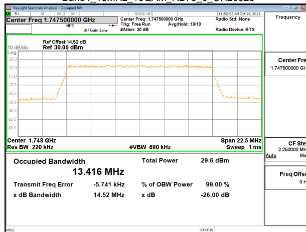
Band4_15MHz_16QAM_RB75_0_CH20325
