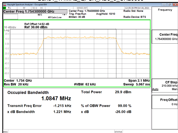
Band4_1.4MHz_QPSK_RB6_0_CH20393
