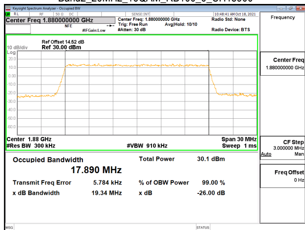
Band2_20MHz_16QAM_RB100_0_CH19100
