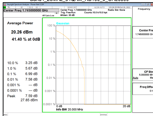
Band4_20MHz_64QAM_RB100_0_CH20300
