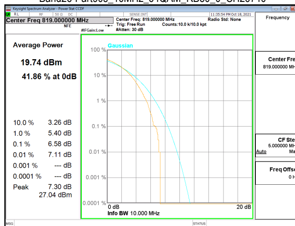
Band26-Part90s_10MHz_64QAM_RB50_0_CH26740
