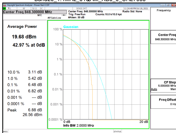
Band26_1.4MHz_64QAM_RB6_0_CH27033
