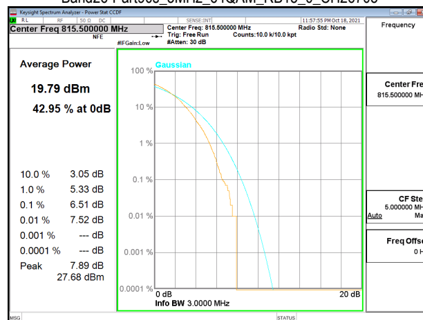
Band26-Part90s_3MHz_64QAM_RB15_0_CH26705
