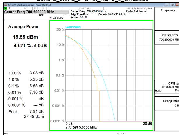
Band12_3MHz_64QAM_RB15_0_CH23095
