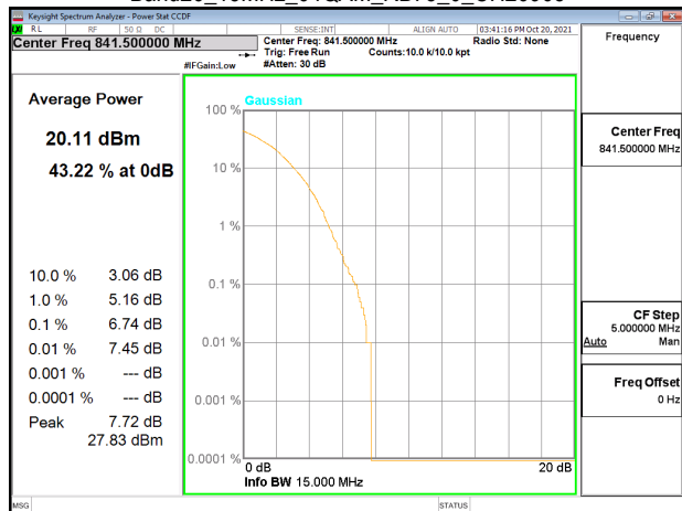
Band26_15MHz_64QAM_RB75_0_CH26965
