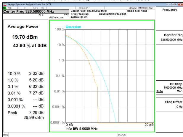
Band26_5MHz_64QAM_RB25_0_CH26915
