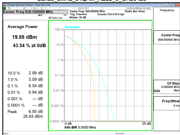
Band5_5MHz_64QAM_RB25_0_CH20525
