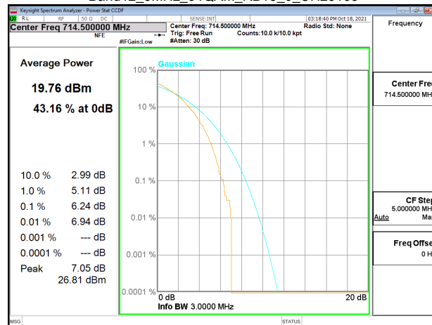
Band12_3MHz_64QAM_RB15_0_CH23165
