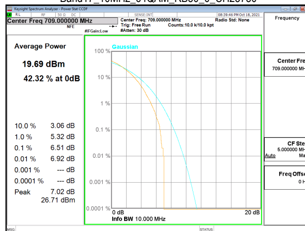
Band17_10MHz_64QAM_RB50_0_CH23780
