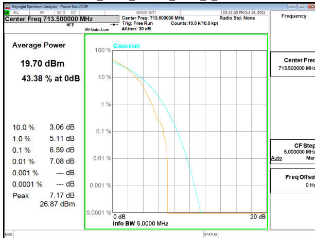
Band12_5MHz_64QAM_RB25_0_CH23155
