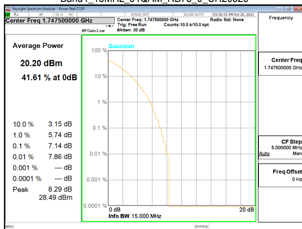
Band4_15MHz_64QAM_RB75_0_CH20325
