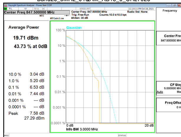
Band26_3MHz_64QAM_RB15_0_CH27025
