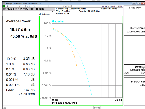
Band38_5MHz_64QAM_RB25_0_CH38000
