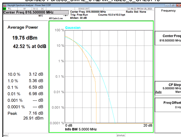
Band26-Part90s_5MHz_64QAM_RB25_0_CH26715
