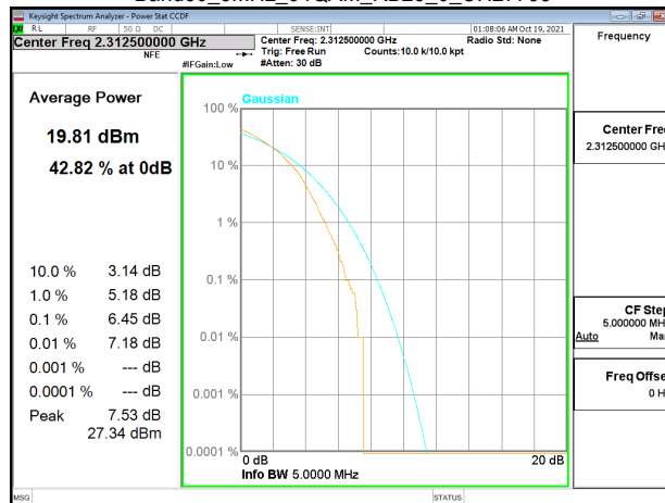
Band30_5MHz_64QAM_RB25_0_CH27735
