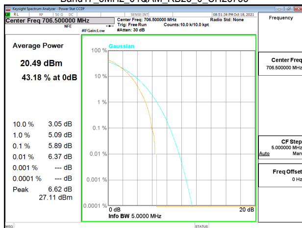
Band17_5MHz_64QAM_RB25_0_CH23755
