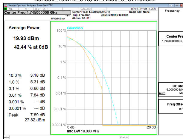
Band66_10MHz_64QAM_RB50_0_CH132322
