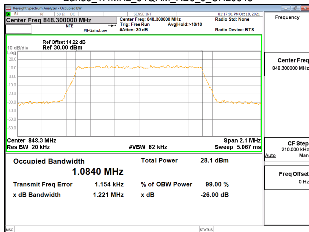
Band5_1.4MHz_64QAM_RB6_0_CH20643
