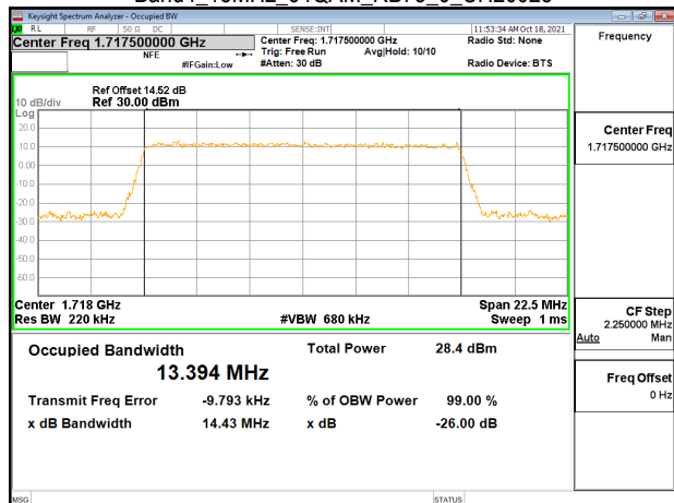
Band4_15MHz_64QAM_RB75_0_CH20175
