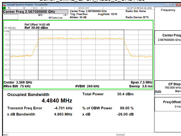
Band7_5MHz_QPSK_RB25_0_CH21425
