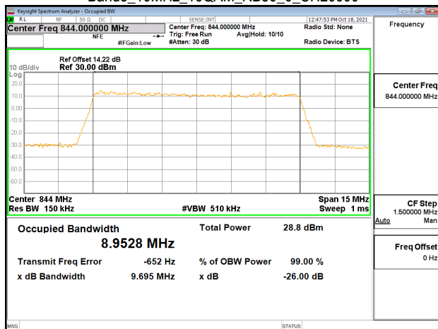
Band5_10MHz_16QAM_RB50_0_CH20600
