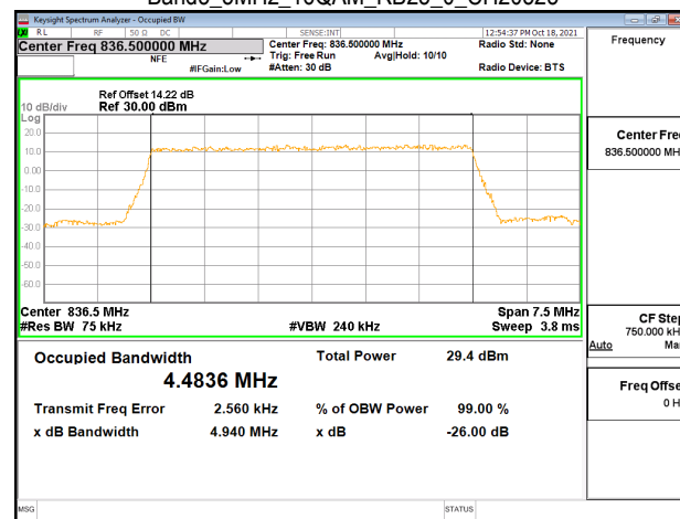
Band5_5MHz_16QAM_RB25_0_CH20625
