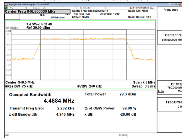
Band5_5MHz_16QAM_RB25_0_CH20625
