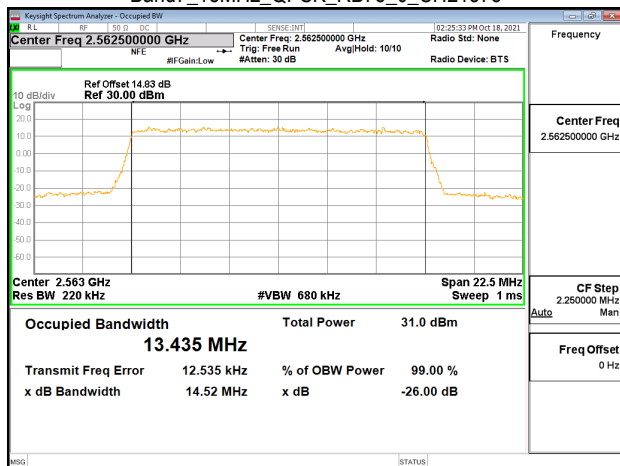
Band7_15MHz_QPSK_RB75_0_CH21375
