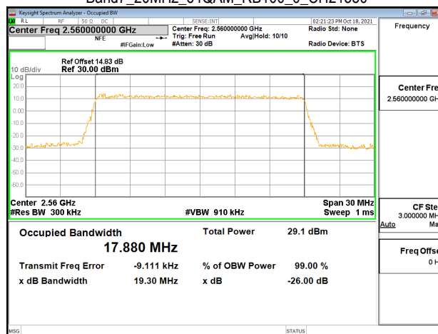
Band7_20MHz_64QAM_RB100_0_CH21350
