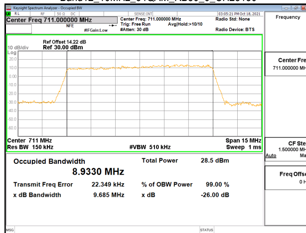
Band12_10MHz_64QAM_RB50_0_CH23130
