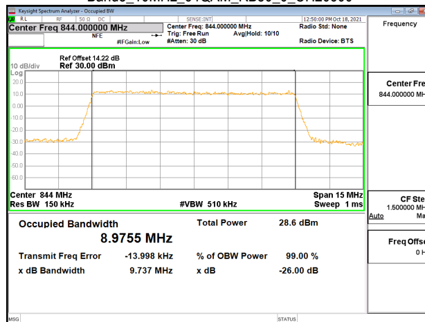
Band5_10MHz_64QAM_RB50_0_CH20600
