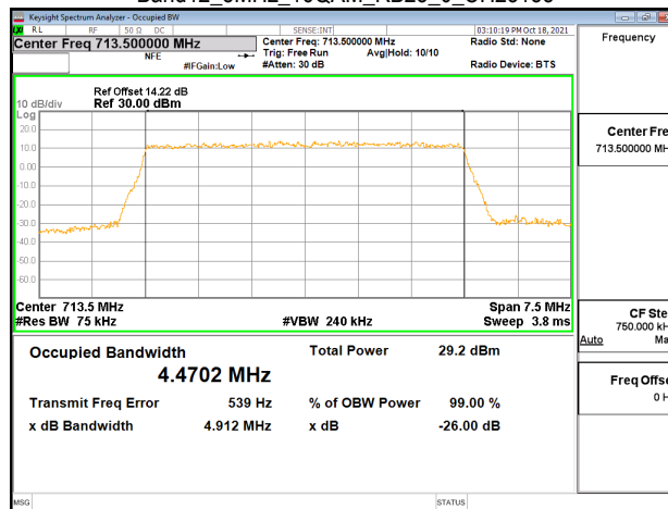
Band12_5MHz_16QAM_RB25_0_CH23155
