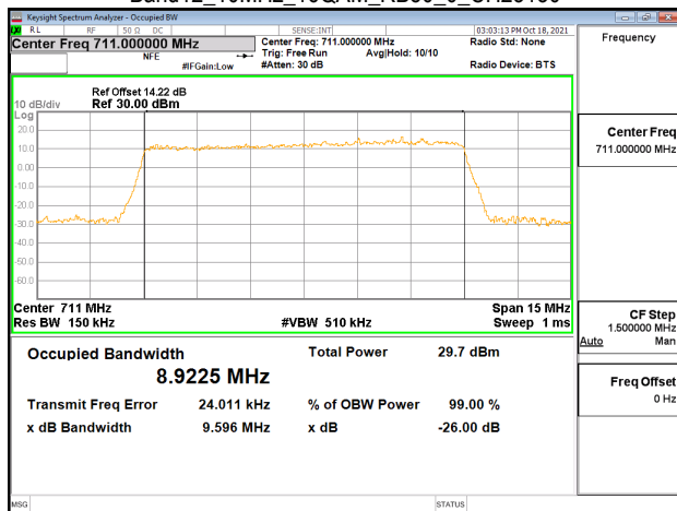
Band12_10MHz_16QAM_RB50_0_CH23130
