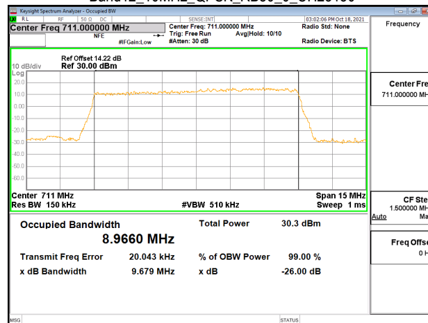
Band12_10MHz_QPSK_RB50_0_CH23130
