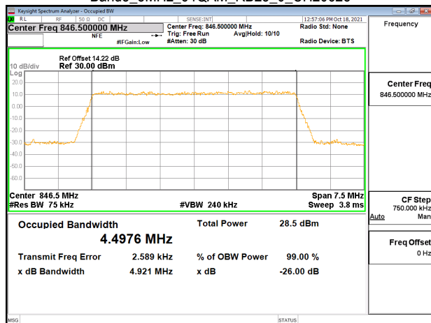
Band5_5MHz_64QAM_RB25_0_CH20625
