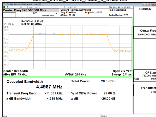
Band5_5MHz_64QAM_RB25_0_CH20525
