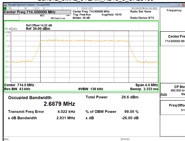
Band12_3MHz_64QAM_RB15_0_CH23165
