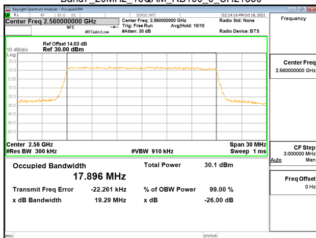
Band7_20MHz_16QAM_RB100_0_CH21350
