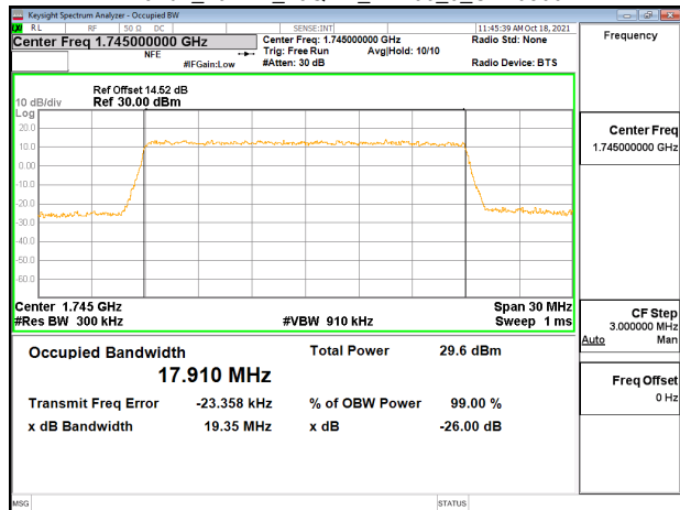
Band4_20MHz_16QAM_RB100_0_CH20300
