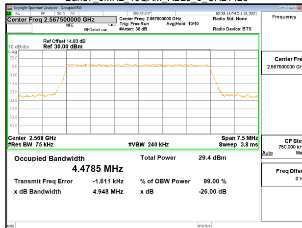
Band7_5MHz_16QAM_RB25_0_CH21425
