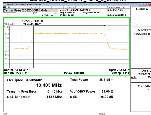
Band38_15MHz_64QAM_RB75_0_CH38175
