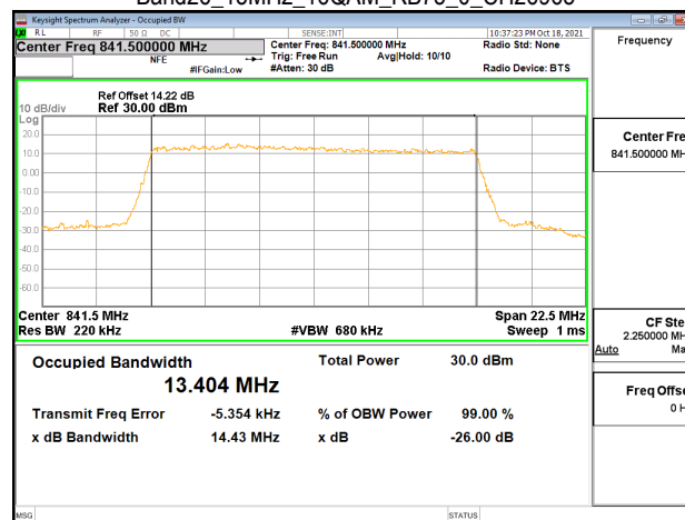
Band26 15MHz 16QAM RB75_0 CH26965
