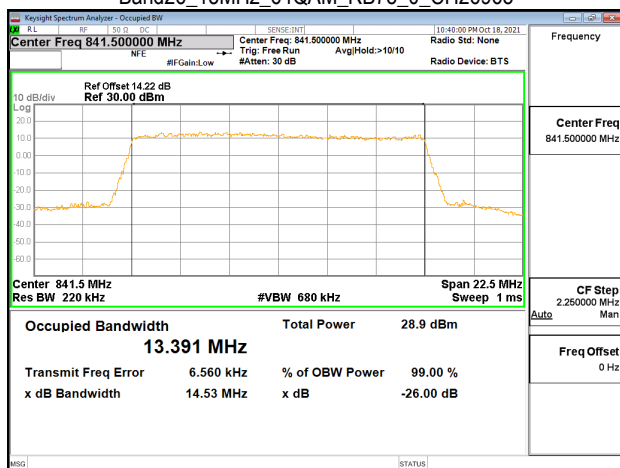
Band26 15MHz 64QAM RB75_0_CH26965
