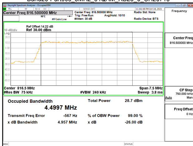
Band26-Part90s_5MHz_64QAM_RB25_0_CH26740
