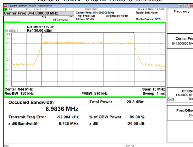
Band26_10MHz_64QAM_RB50_0_CH26990
