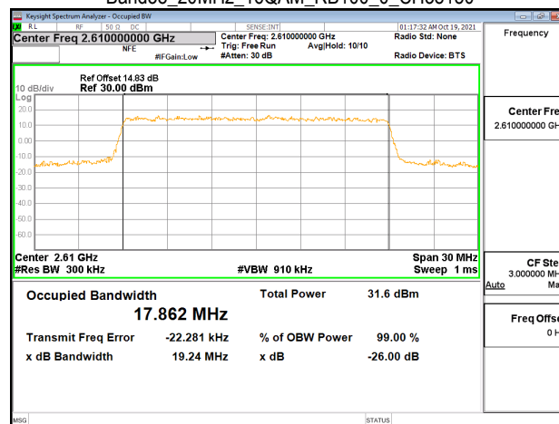
Band38_20MHz_16QAM_RB100_0_CH38150
