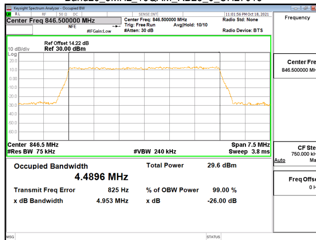
Band26_5MHz_16QAM_RB25_0_CH27015
