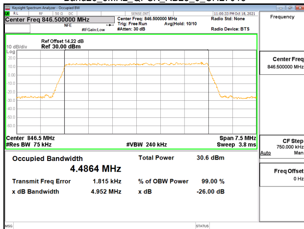
Band26_5MHz_QPSK_RB25_0_CH27015
