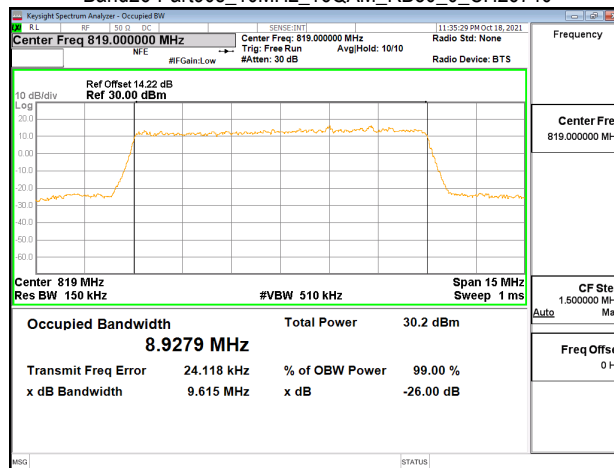
Band26-Part90s_10MHz_64QAM_RB50_0_CH26740
