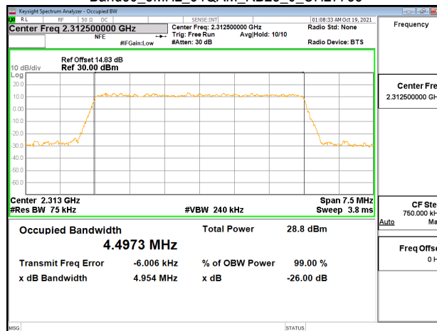
Band30_5MHz_64QAM_RB25_0_CH27735
