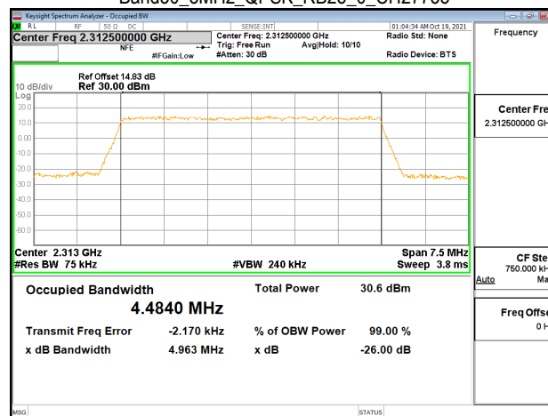
Band30 5MHz QPSK RB25_0_CH27735
