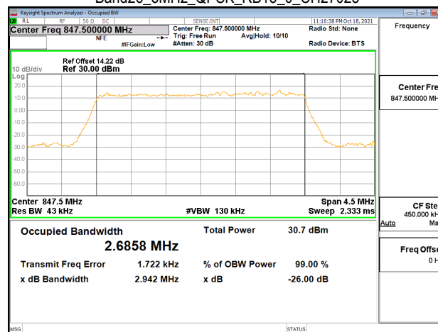
Band26_3MHz_QPSK_RB15_0_CH27025
