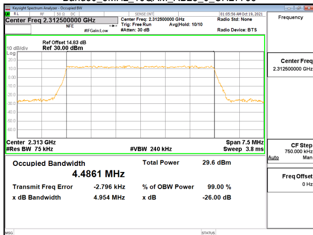
Band30_5MHz_16QAM_RB25_0_CH27735
