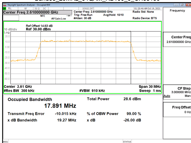
Band38_20MHz_64QAM_RB100_0_CH38150
