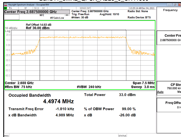
Band41_5MHz_QPSK_RB25_0_CH41565
