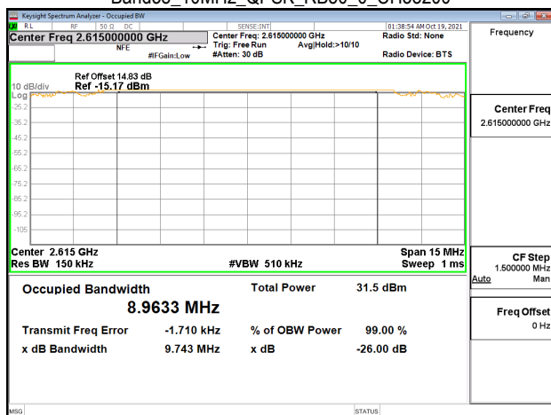
Band38_10MHz_QPSK_RB50_0_CH38200
