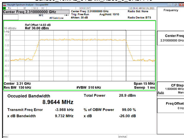
Band30_10MHz_64QAM_RB50_0_CH27710
