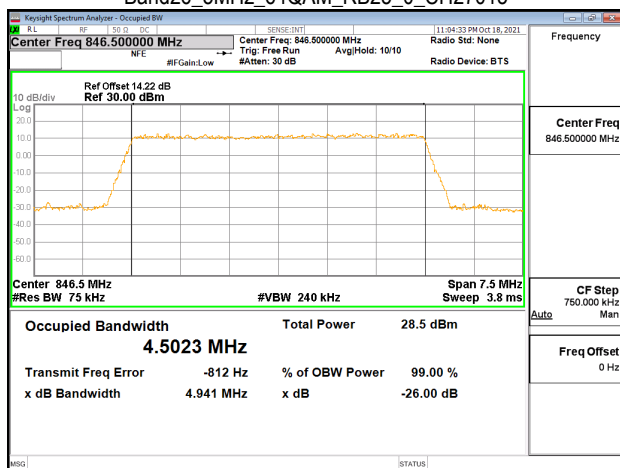
Band26_5MHz_64QAM_RB25_0_CH27015
