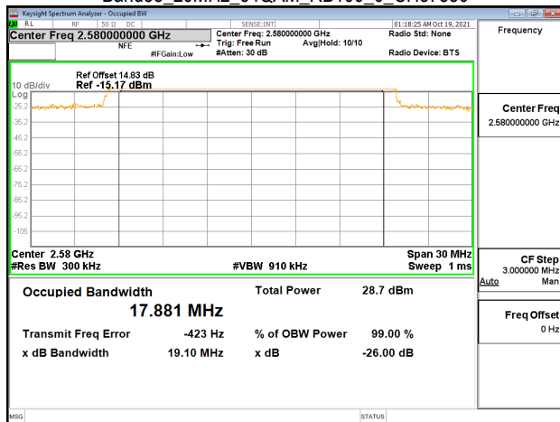
Band38_20MHz_64QAM_RB100_0_CH38000
