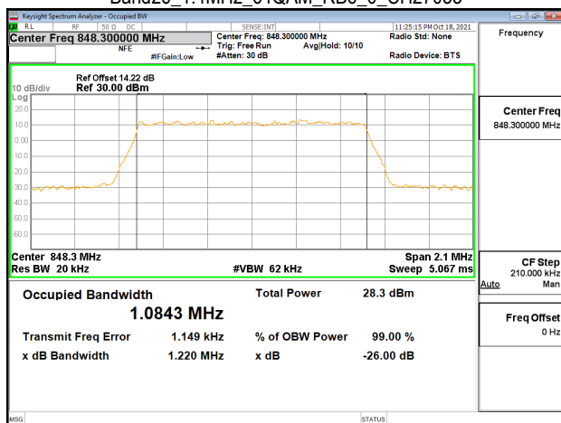
Band26_1.4MHz_64QAM_RB6_0_CH27033
