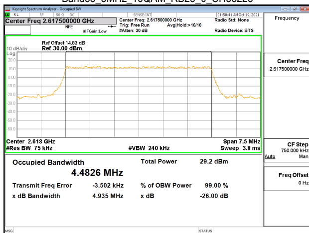
Band38_5MHz_16QAM_RB25_0_CH38225
