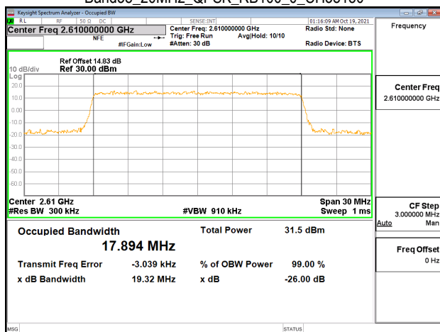
Band38_20MHz_QPSK_RB100_0_CH38150
