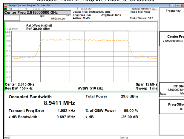
Band38_10MHz_16QAM_RB50_0_CH38200
