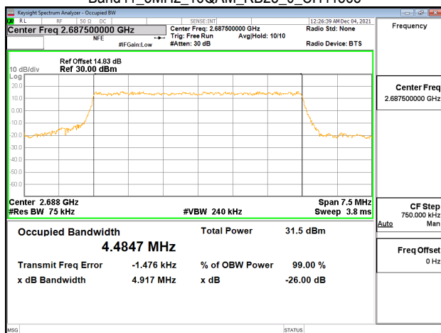
Band41_5MHz_16QAM_RB25_0_CH41565
