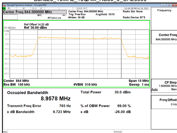
Band26_10MHz_16QAM_RB50_0_CH26990
