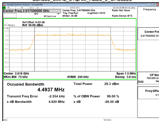
Band38_5MHz_64QAM_RB25_0_CH38225
