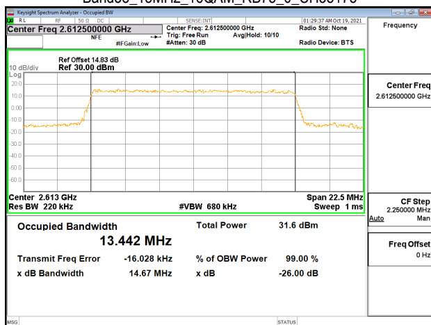
Band38_15MHz_16QAM_RB75_0_CH38175
