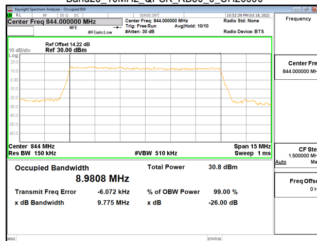
Band26_10MHz_QPSK_RB50_0_CH26990
