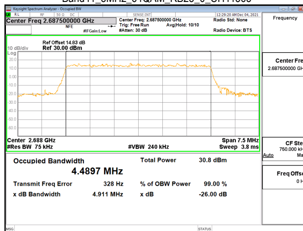
Band41_5MHz_64QAM_RB25_0_CH41565
