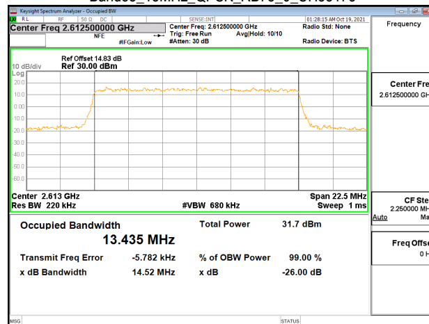
Band38_15MHz_QPSK_RB75_0_CH38175
