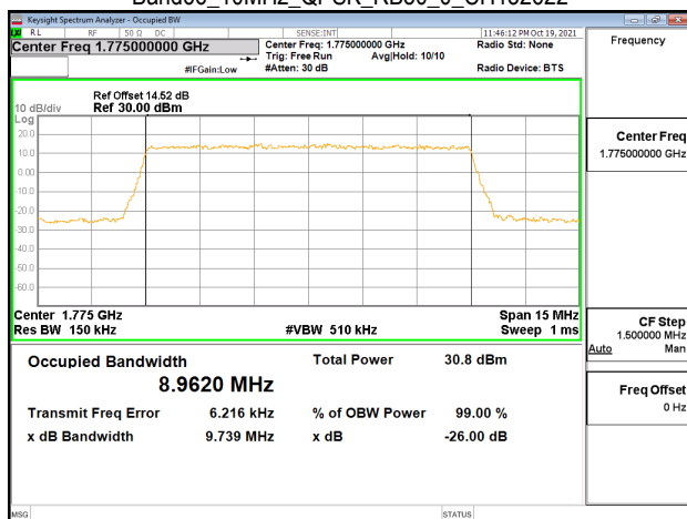
Band66_10MHz_QPSK_RB50_0_CH132622
