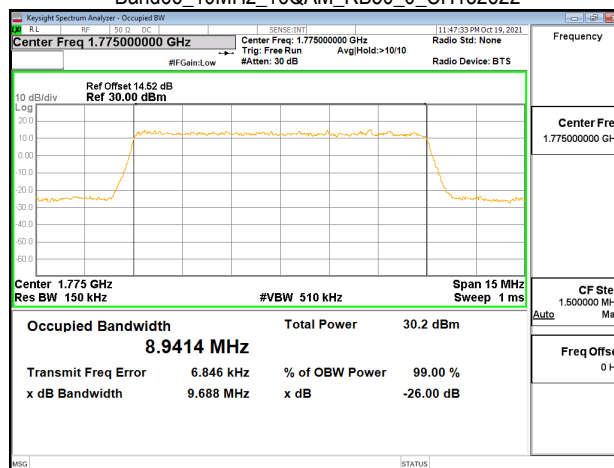
Band66_10MHz_16QAM_RB50_0_CH132622
