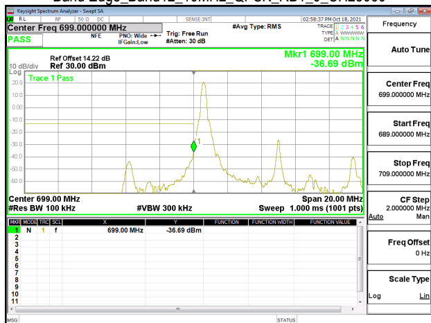
Band Edge_Band12_10MHz_QPSK_RB1_0_CH23060
