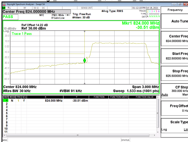
Band Edge_Band5_1.4MHz_QPSK_RB6_0_CH20407
