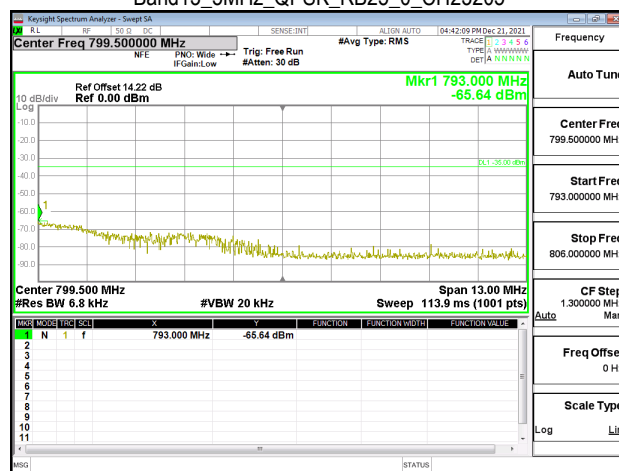
Band13_5MHz_QPSK_RB25_0_CH23255
