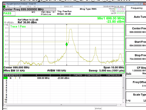
Band Edge_Band12_5MHz_QPSK_RB1_24_CH23155
