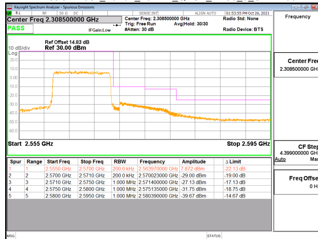
Emission Mask_Band7_10MHz_QPSK_RB50_0_CH21400
