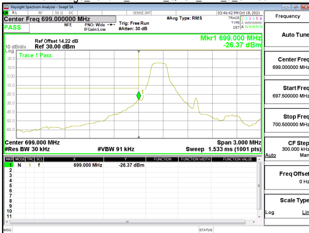
Band Edge_Band12_1.4MHz_QPSK_RB1_0_CH23017
