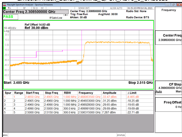
Emission Mask_Band7_15MHz_QPSK_RB75_0_CH20825
