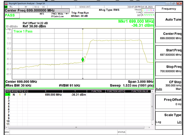
Band Edge_Band12_1.4MHz_QPSK_RB6_0_CH23173
