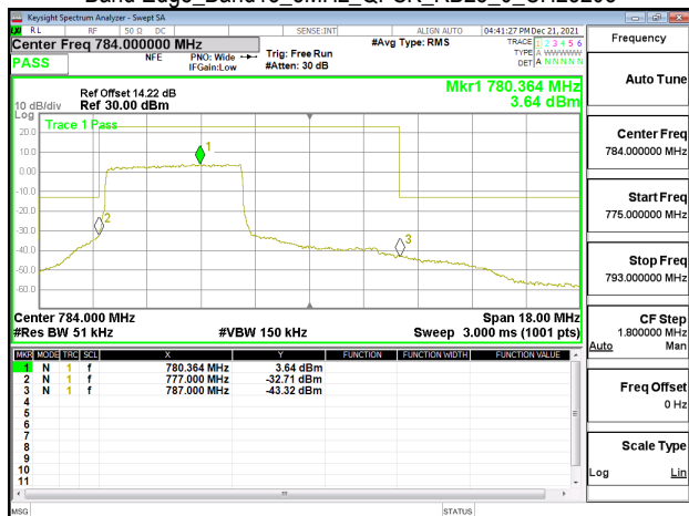
Band Edge_Band13_5MHz_QPSK_RB25_0_CH23205
