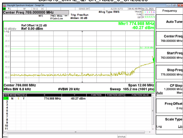
Band13_5MHz_QPSK_RB25_0_CH23255
