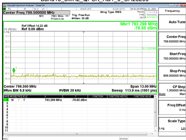
Band13_5MHz_QPSK_RB1_0_CH23205
