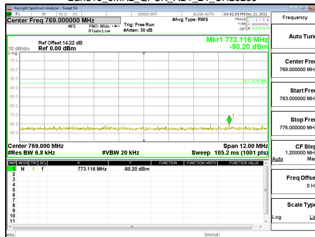
Band13_5MHz_QPSK_RB1_24_CH23255
