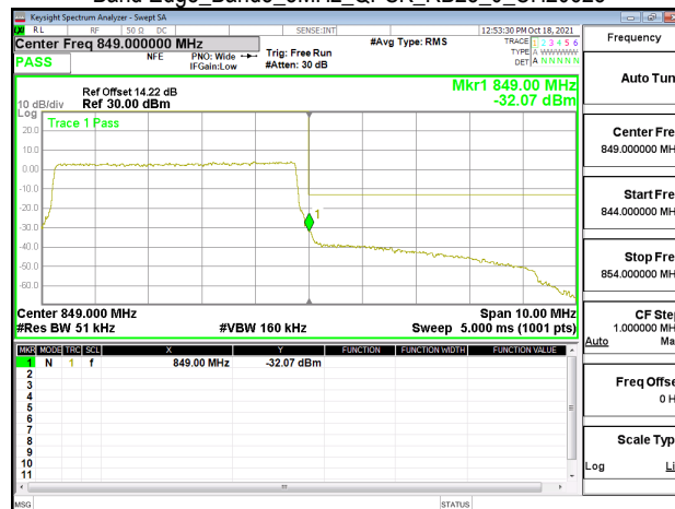
Band Edge_Band5_5MHz_QPSK_RB25_0_CH20625
