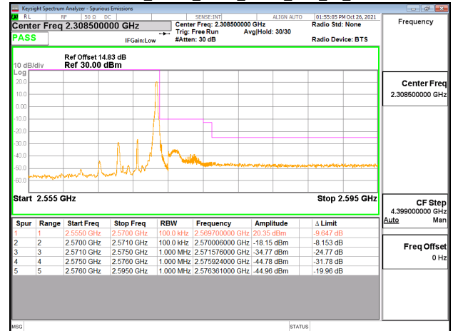
Emission Mask_Band7_5MHz_QPSK_RB1_24_CH21425
