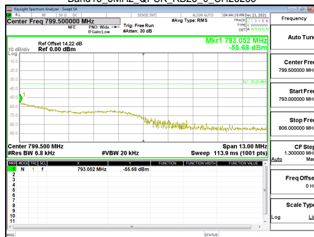
Band13_5MHz_QPSK_RB25_0_CH23255
