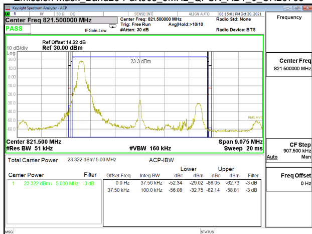
Emission Mask_Band26-Part90s_5MHz_QPSK_RB1_0_CH26765
