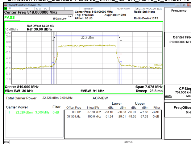
Emission Mask_Band26-Part90s_3MHz_QPSK_RB15_0_CH26775
