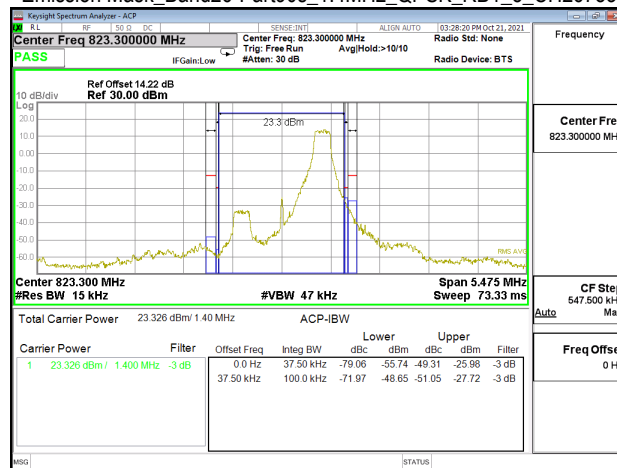
Emission Mask_Band26-Part90s_1.4MHz_QPSK_RB1_5_CH26783
