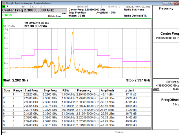
Emission Mask_Band30_5MHz_QPSK_RB1_24_CH27735
