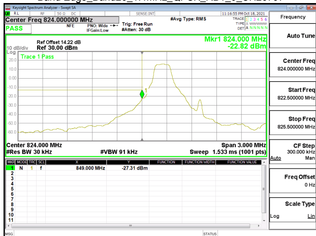
Band Edge_Band26_1.4MHz_QPSK_RB1_5_CH27033
