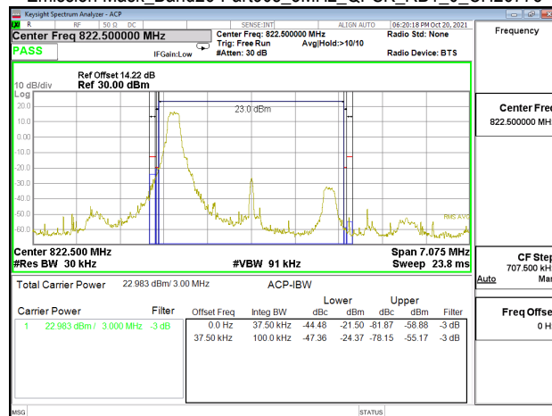
Emission Mask_Band26-Part90s_3MHz_QPSK_RB1_0_CH26775
