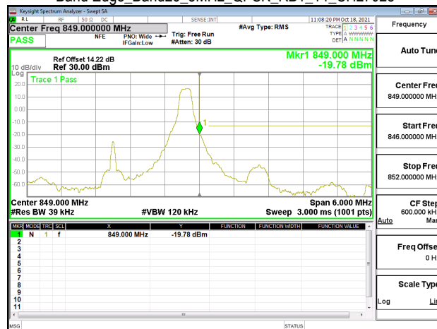
Band Edge_Band26_3MHz_QPSK_RB1_14_CH27025
