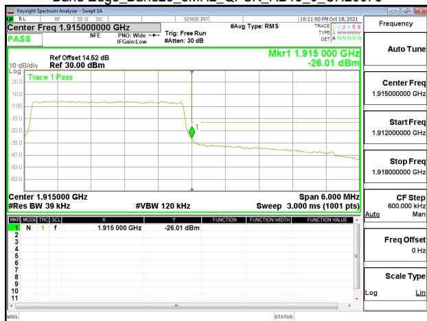
Band Edge_Band25_5MHz_QPSK_RB1_0_CH26065
