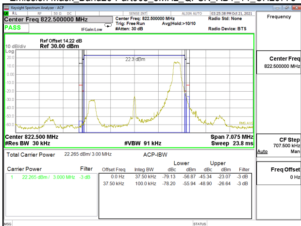
Emission Mask_Band26-Part90s_3MHz_QPSK_RB1_14_CH26775
