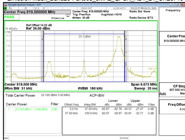
Emission Mask_Band26-Part90s_5MHz_QPSK_RB1_24_CH26765
