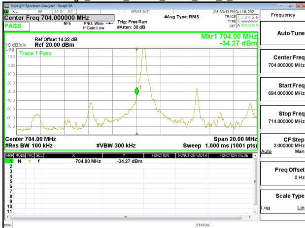
Band Edge_Band17_10MHz_QPSK_RB1_0_CH23780
