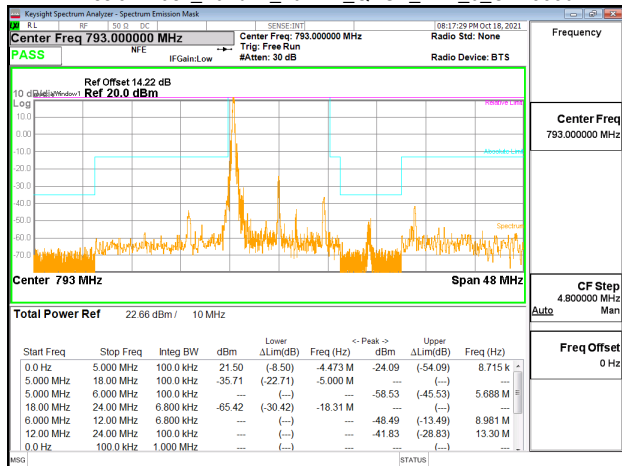
Emission Mask_Band14_10MHz_QPSK_RB1_49_CH23330
