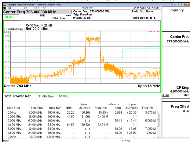
Emission Mask_Band14_10MHz_QPSK_RB1_0_CH23330
