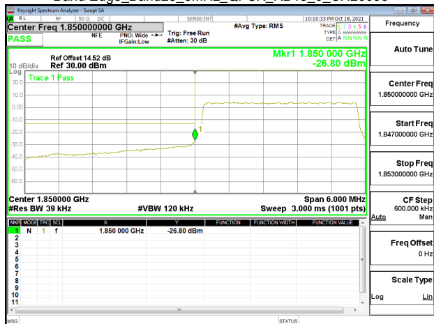
Band Edge_Band25_3MHz_QPSK_RB15_0_CH26675
