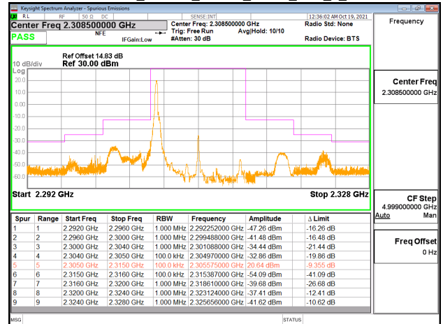
Emission Mask_Band30_10MHz_QPSK_RB1_0_CH27710
