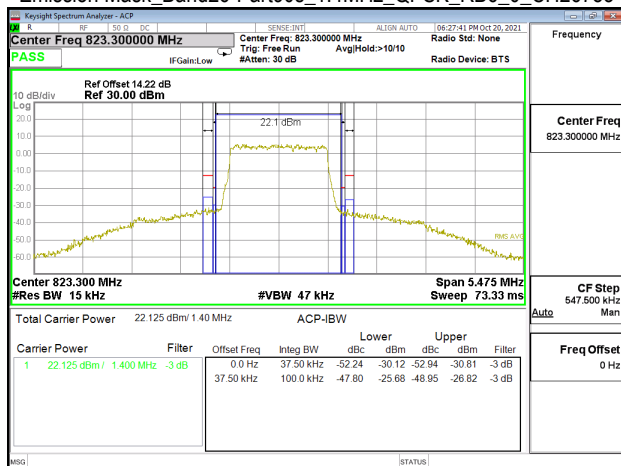
Emission Mask_Band26-Part90s_1.4MHz_QPSK_RB6_0_CH26783
