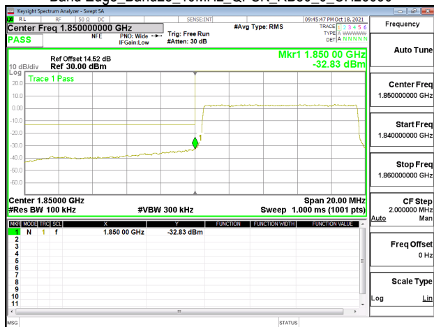
Band Edge_Band25_10MHz_QPSK_RB50_0_CH26090
