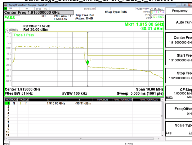
Band Edge_Band25_5MHz_QPSK_RB25_0_CH26665
