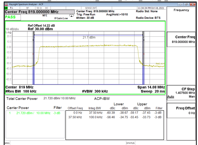
Emission Mask_Band26-Part90s_10MHz_QPSK_RB50_0_CH26740
