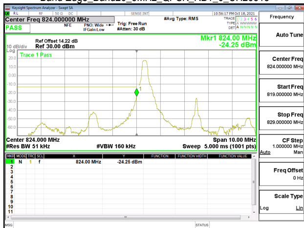
Band Edge_Band26_5MHz_QPSK_RB1_0_CH26815
