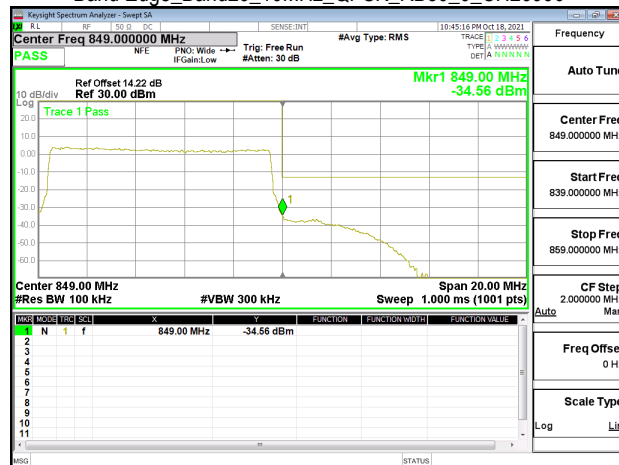
Band Edge_Band26_15MHz_QPSK_RB1_0_CH26865
