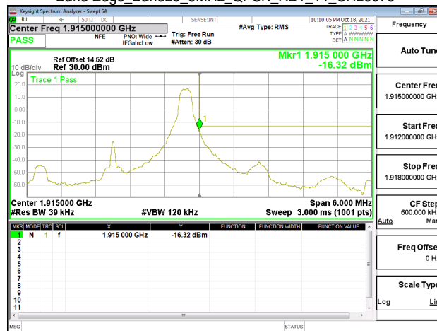
Band Edge_Band25_3MHz_QPSK_RB1_14_CH26675
