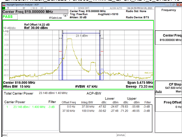
Emission Mask_Band26-Part90s_1.4MHz_QPSK_RB1_0_CH26783
