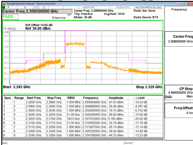
Emission Mask_Band30_5MHz_QPSK_RB25_0_CH27685
