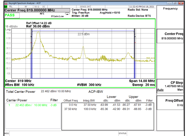
Emission Mask_Band26-Part90s_10MHz_QPSK_RB1_49_CH26740
