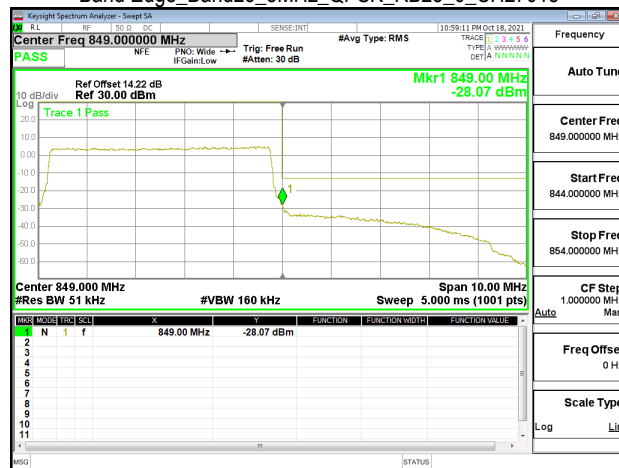
Band Edge_Band26_5MHz_QPSK_RB25_0_CH27015
