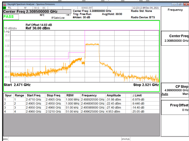
Emission Mask_Band41_5MHz_QPSK_RB25_0_CH39675
