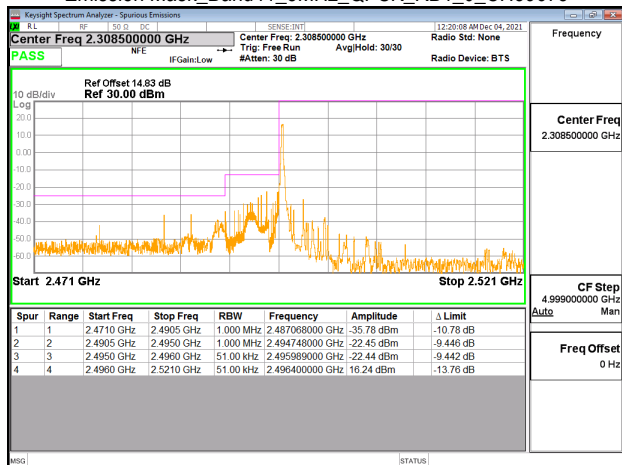
Emission Mask_Band41_5MHz_QPSK_RB1_24_CH41565
