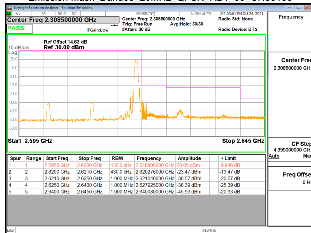
Emission Mask_Band38_20MHz_QPSK_RB100_0_CH37850
