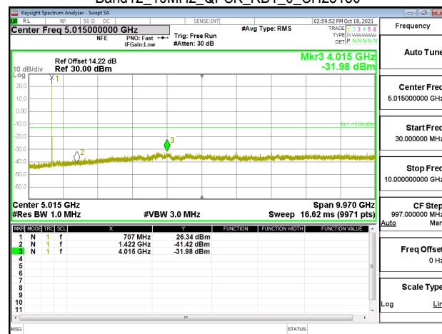
Band12_10MHz_QPSK_RB1_0_CH23130
