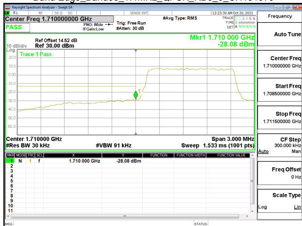
Band Edge_Band66_1.4MHz_QPSK_RB6_0_CH132665
