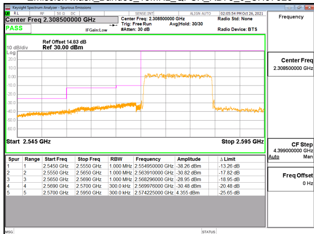
Emission Mask_Band38_15MHz_QPSK_RB75_0_CH38175
