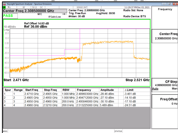
Emission Mask_Band41_20MHz_QPSK_RB100_0_CH39750
