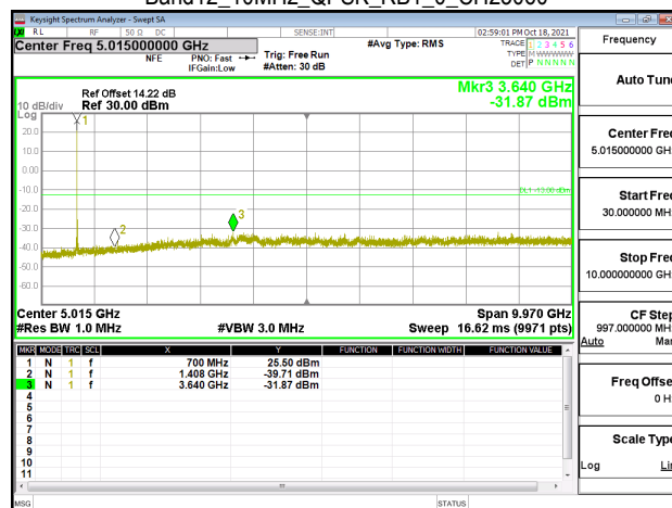
Band12_10MHz_QPSK_RB1_0_CH23095
