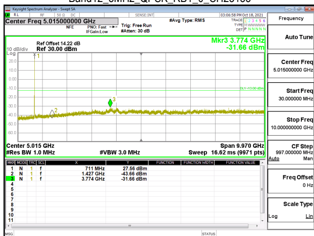
Band12_5MHz_QPSK_RB1_0_CH23155
