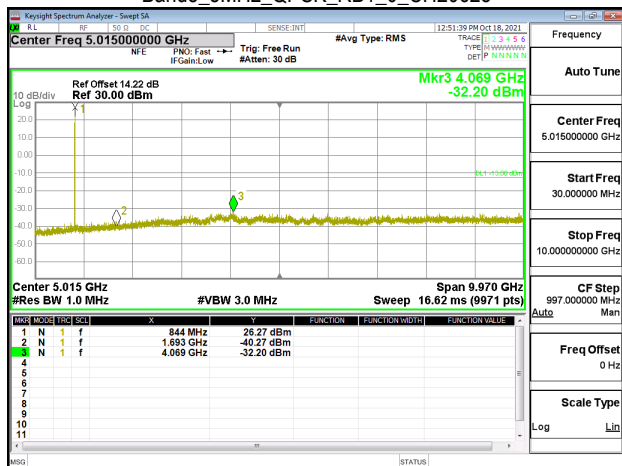
Band5_5MHz_QPSK_RB1_0_CH20625
