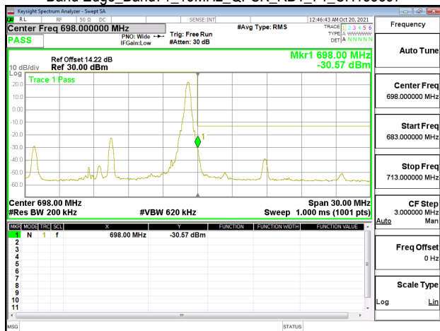
Band Edge_Band71_15MHz_QPSK_RB75_0_CH133197
