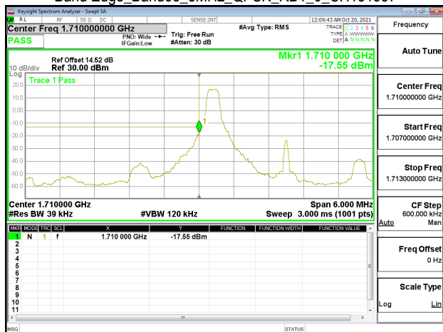
Band Edge_Band66_3MHz_QPSK_RB1_0_CH131987
