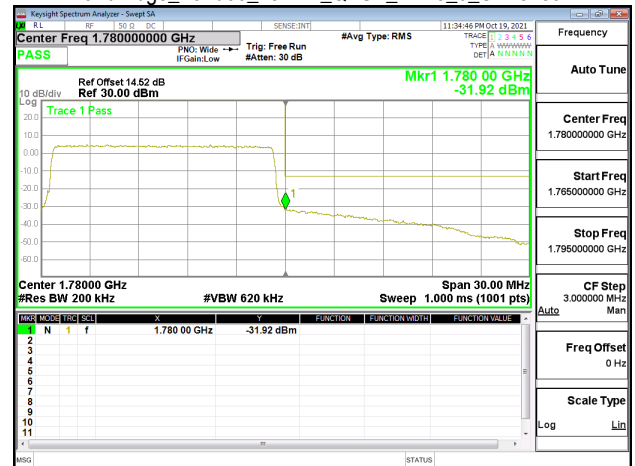
Band Edge_Band66_15MHz_QPSK_RB75_0_CH132597
