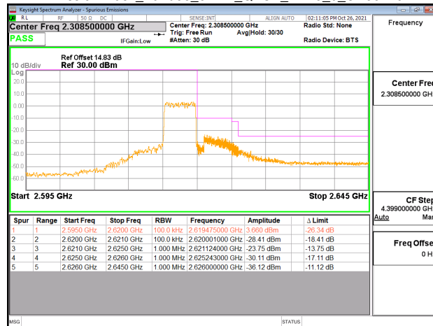
Emission Mask_Band38_5MHz_QPSK_RB25_0_CH38225
