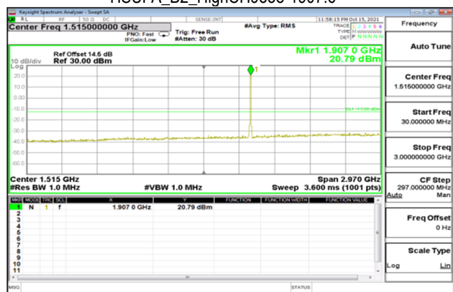
HSUPA_B2_HighCH9538-1907.6
