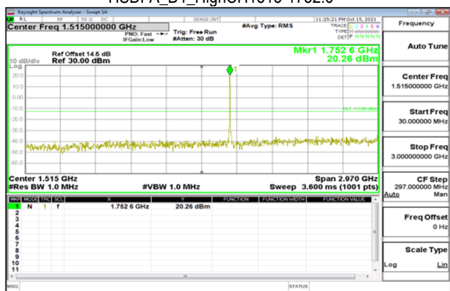
HSDPA_B4_HighCH1513-1752.6
