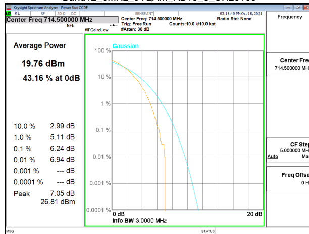
Band12_3MHz_64QAM_RB15_0_CH23165
