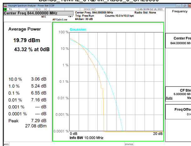
Band5_10MHz_64QAM_RB50_0_CH20600
