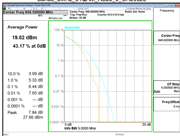
Band5_5MHz_64QAM_RB25_0_CH20625
