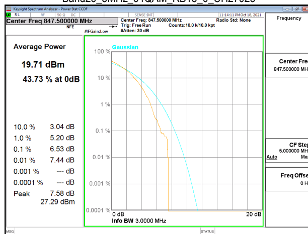
Band26_3MHz_64QAM_RB15_0_CH27025
