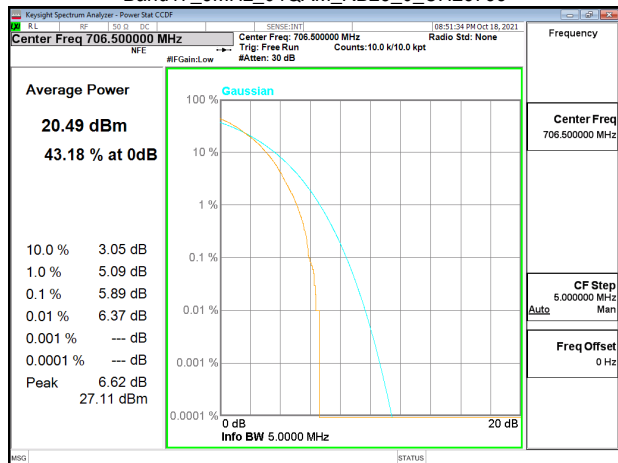
Band17_5MHz_64QAM_RB25_0_CH23755
