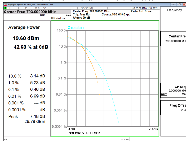
Band14_5MHz_64QAM_RB25_0_CH23330
