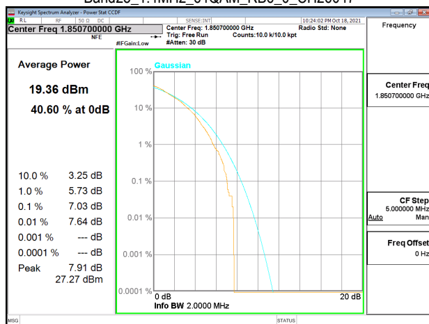
Band25_1.4MHz_64QAM_RB6_0_CH26047
