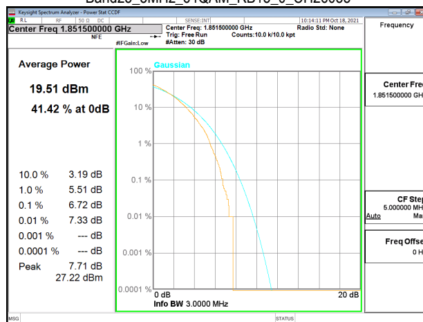
Band25_3MHz_64QAM_RB15_0_CH26055
