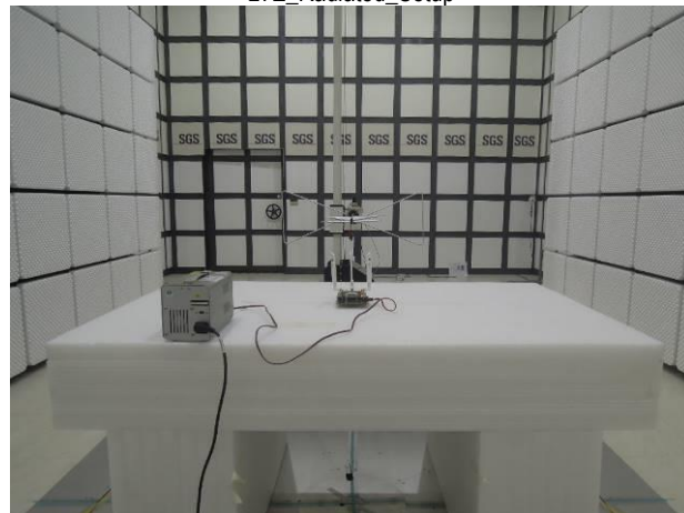
LTE_Radiated_Setup
