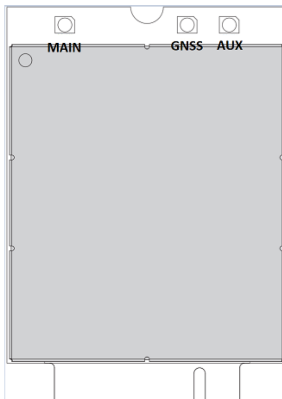
Figure 13: Antenna Configurations
