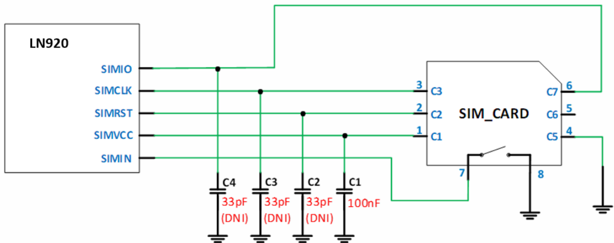
Figure 9: SIM Schematics
