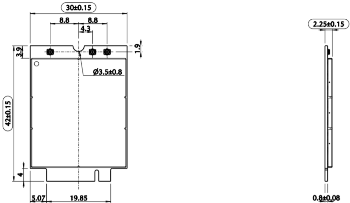
Figure 17: Mechanical Design Drawing
