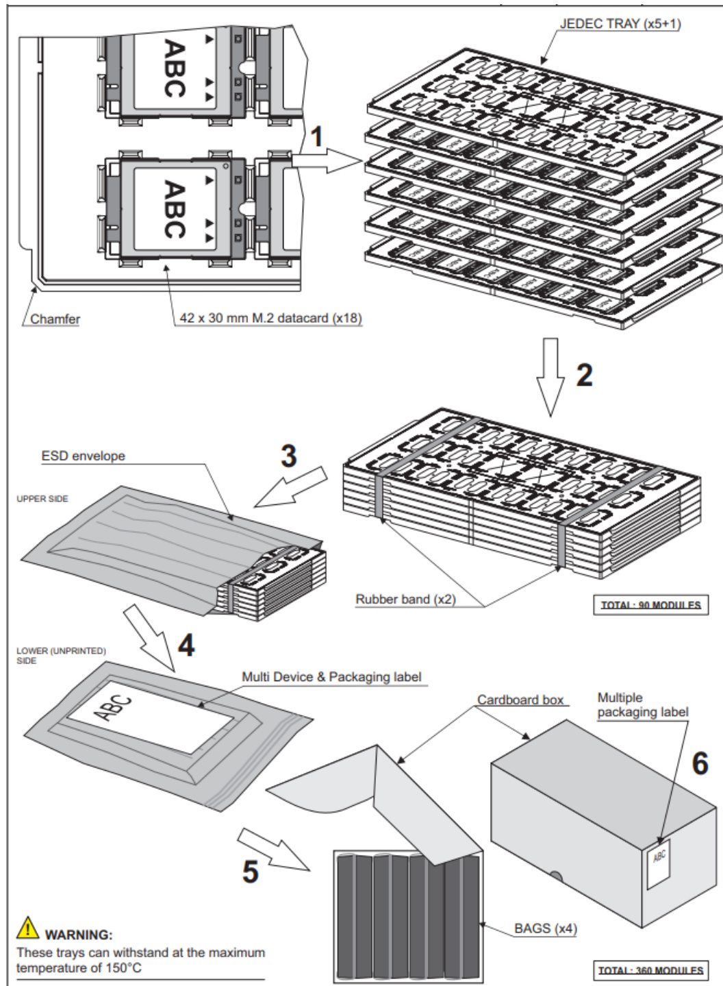
Figure 18: Tray Packaging
