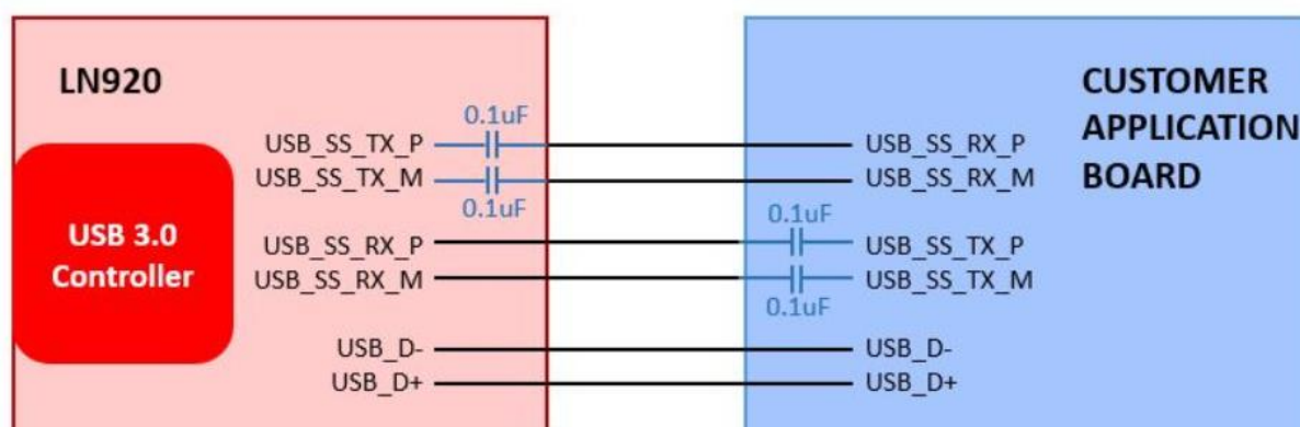
Figure 8: Connection for USB Interface
