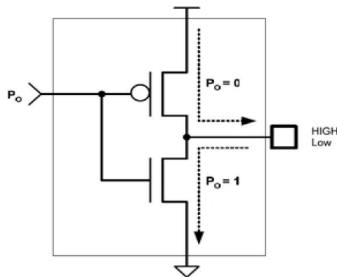
Figure 11: GPIO Output Pin Equivalent Circuit
