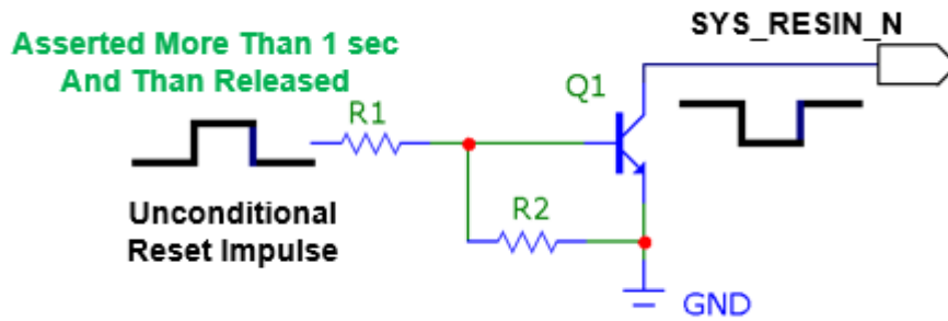
Figure 7: Circuit for RESTE by SYSTEM_RESET_N
