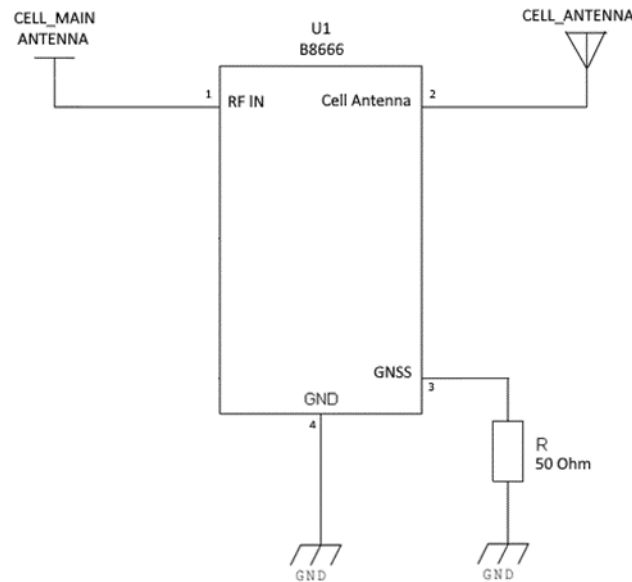
Figure 16: Reference Schematic
