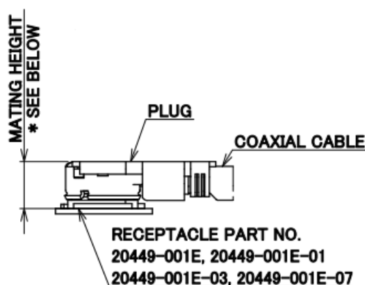
Figure 14: MHF-4 RF connector
