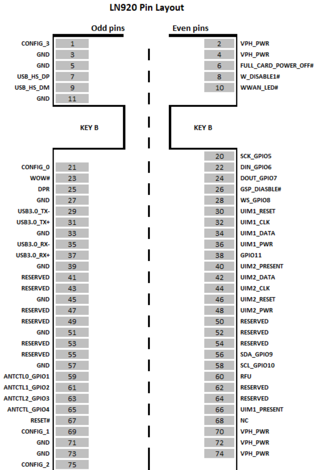
Figure 2: LN920 Pin-out
