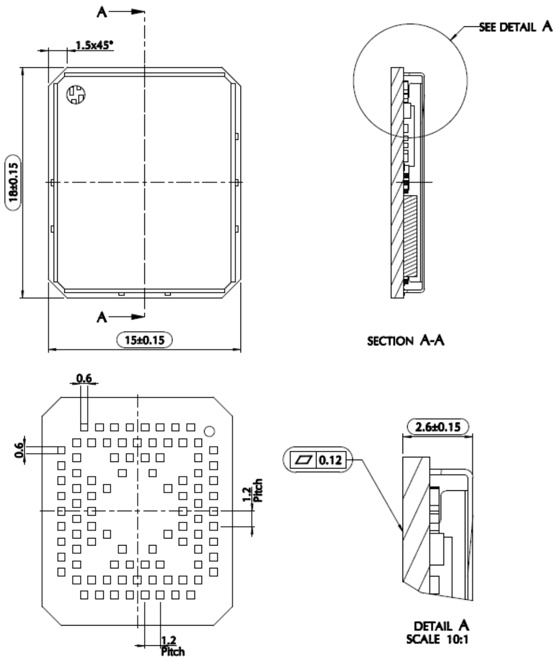
Figure 19: Mechanical Drawing of ME310G1-WW, ME310G1-WWV, ME310G1-W2, and ME310G1-W3
