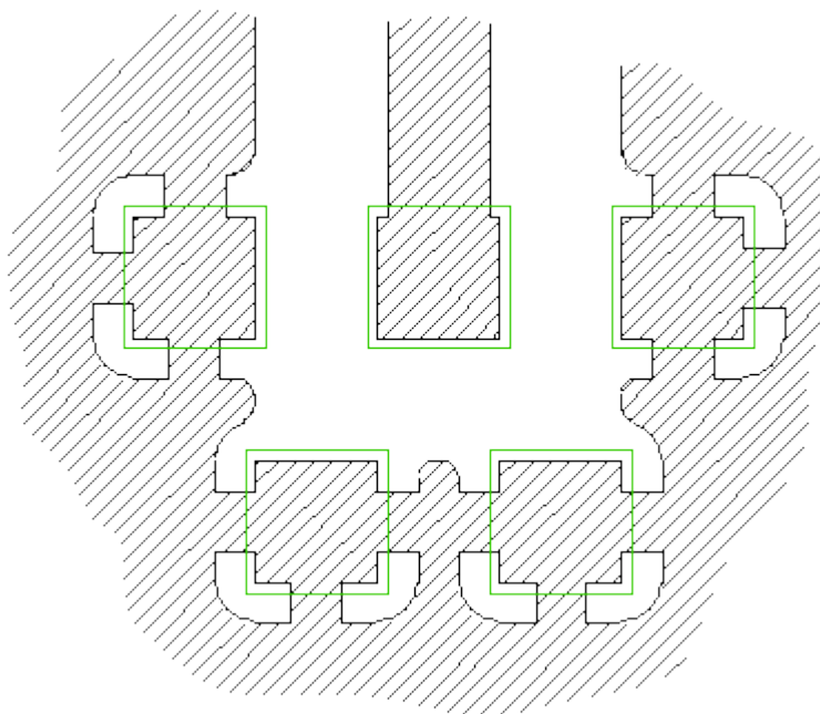
Figure 11: Layout for the Antenna pad connection
