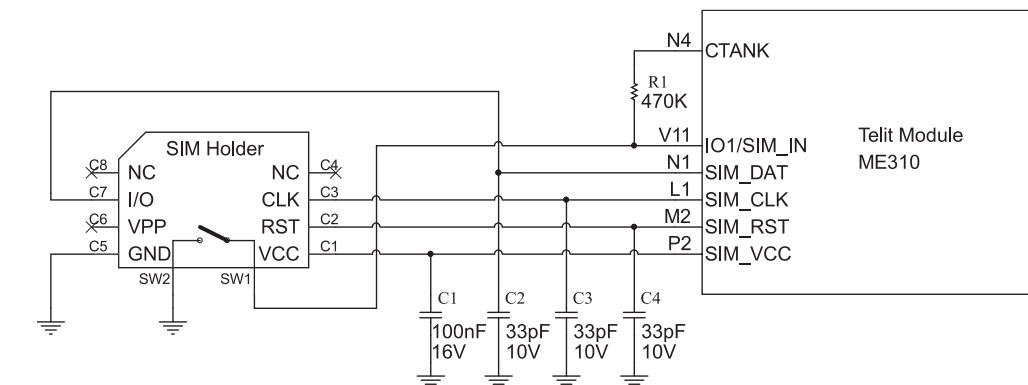
Figure 10: SIM Holder schematic
