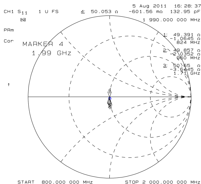
Figure 14: Line input impedance
