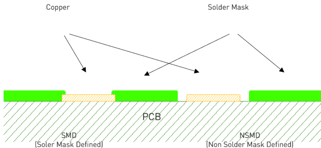
Figure 26: PCB solder pad recommendations
