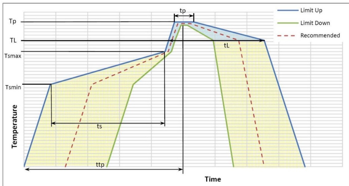
Figure 27: Recommended Solder reflow profile
