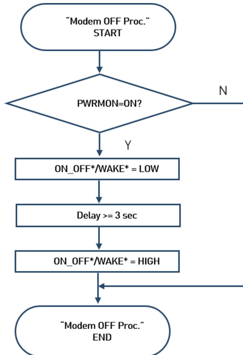
Figure 7: Modem OFF Process flow chart
