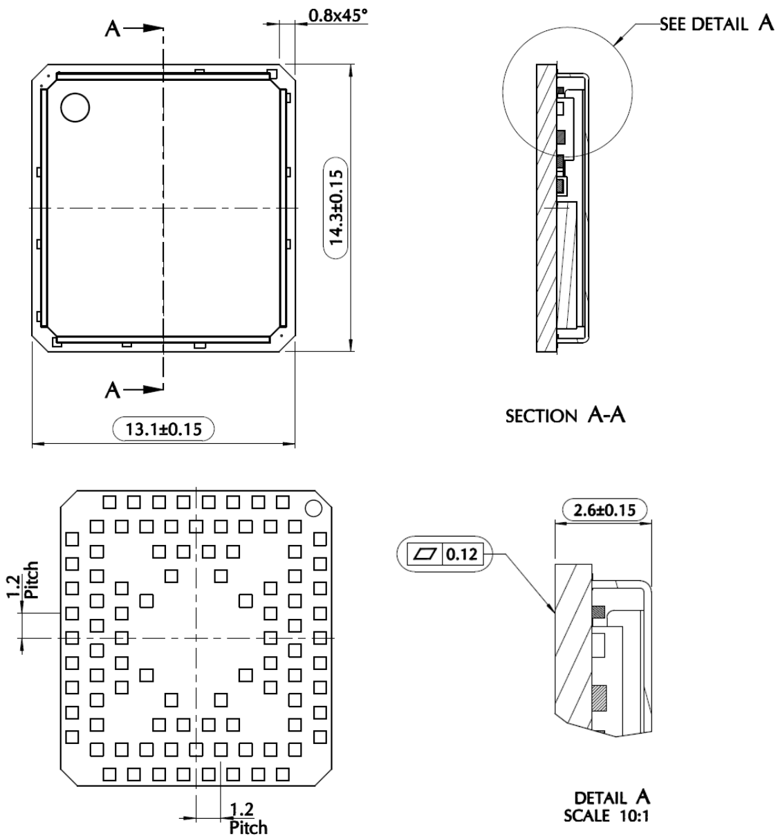
Figure 18: Mechanical Drawing of ME310G1-W1
