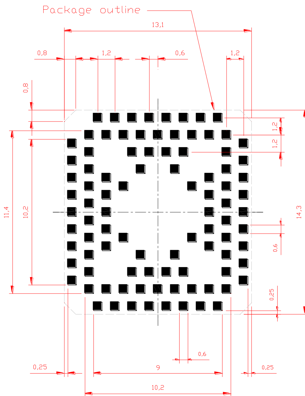
Figure 20: Copper Pattern (top view)
