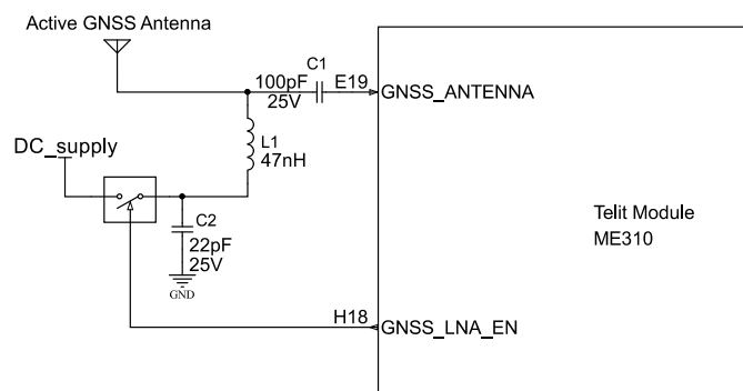
Figure 17: Antenna bias circuitry example
