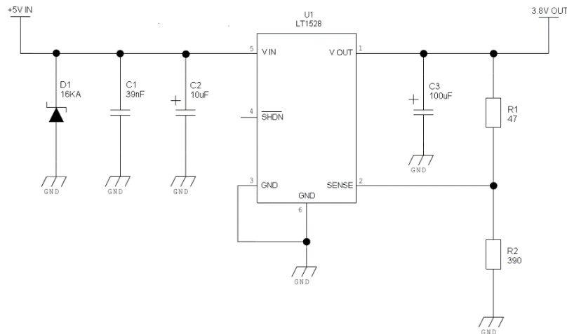
Figure 3: Example of a linear regulator with 5V input
