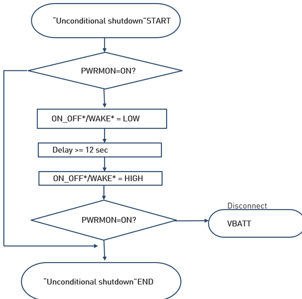
Figure 8: Unconditional shutdown of ME310G1
