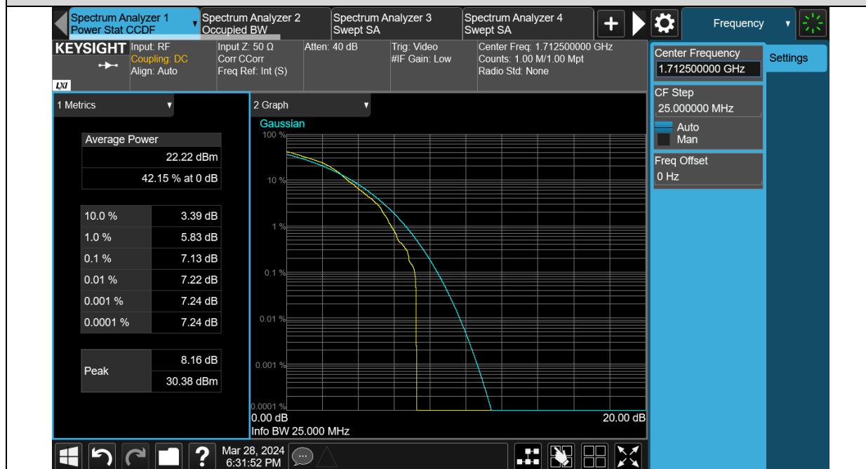
Band66-5MHz-16QAM-132322
