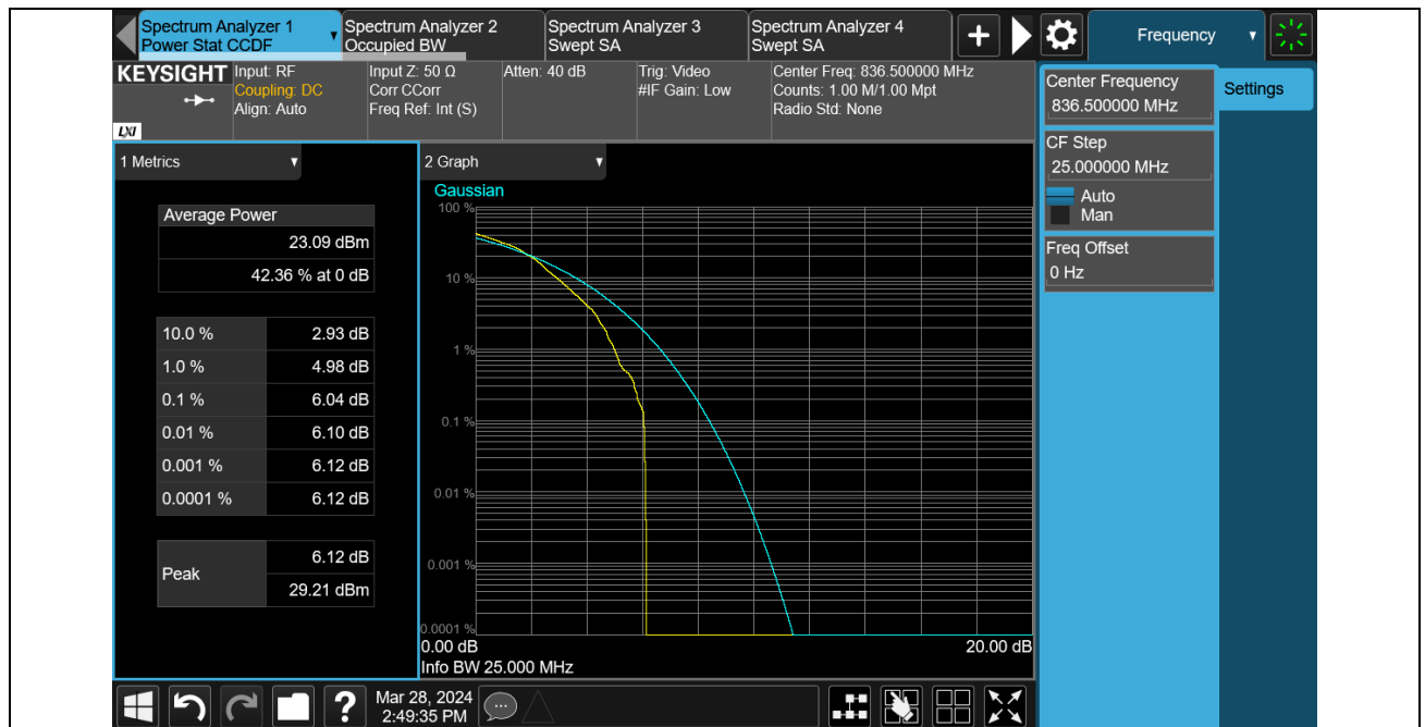
Band26-10MHz-16QAM-26990
