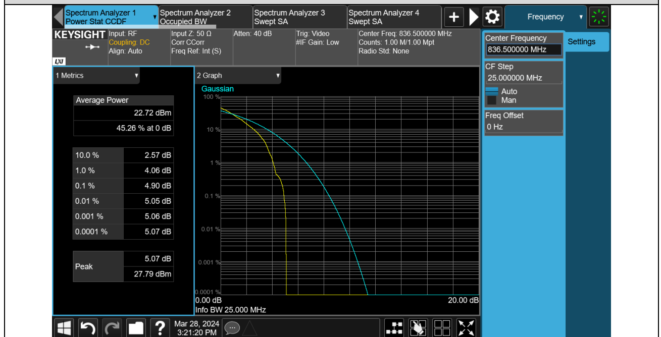
Band26-3MHz-QPSK-27025
