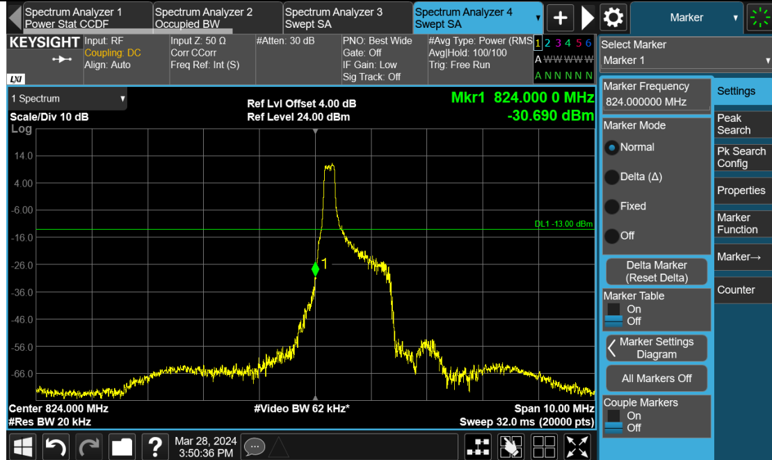
Band26-1.4MHz-QPSK-26797-6RB#0
