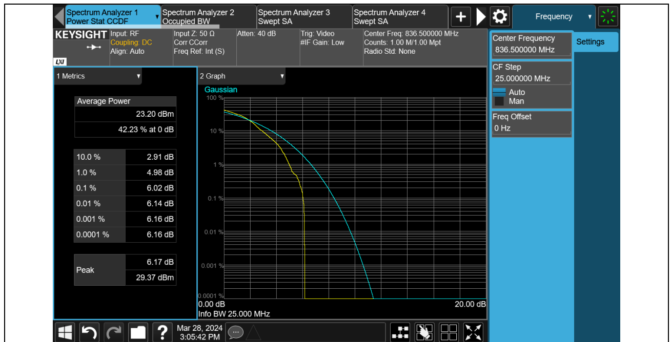
Band26-5MHz-16QAM-27015
