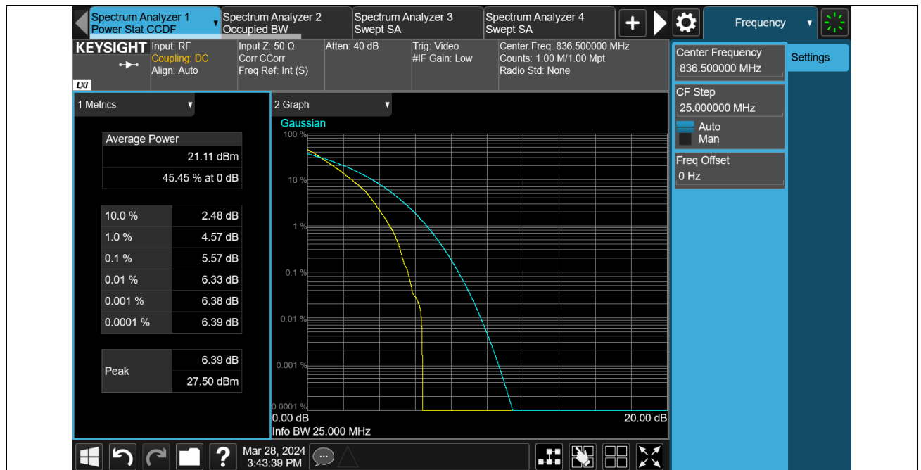
Band26-1.4MHz-16QAM-27033
