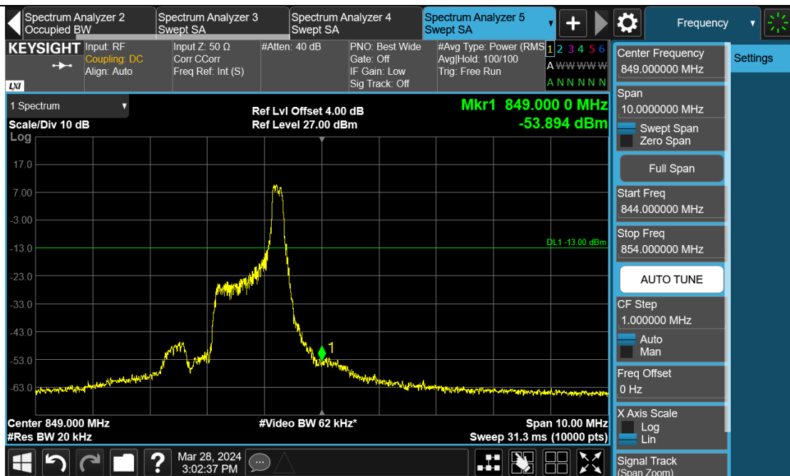
Band26-10MHz-QPSK-26990-6RB#0
