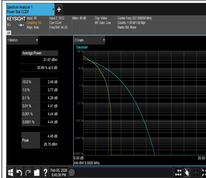
B18(824-830)-15KHz-QPSK-23998-12RB#0-PASS
