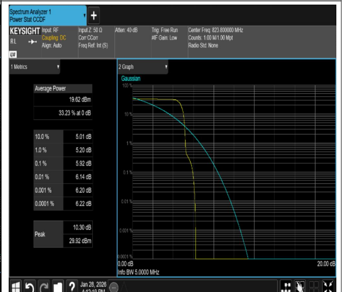
B18(815-824)-15KHz-QPSK-23938-1RB#0-PASS
