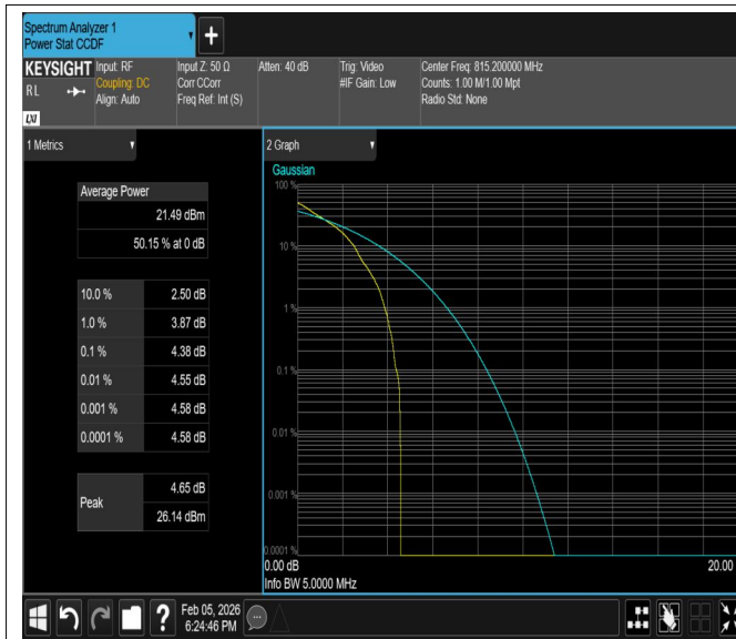
B18(815-824)-15KHz-QPSK-23895-12RB#0-PASS
