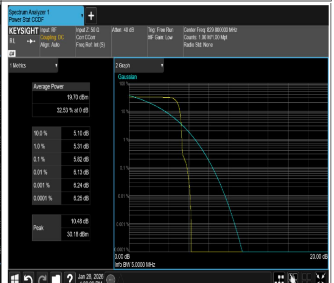
B18(824-830)-15KHz-QPSK-23998-1RB#0-PASS
