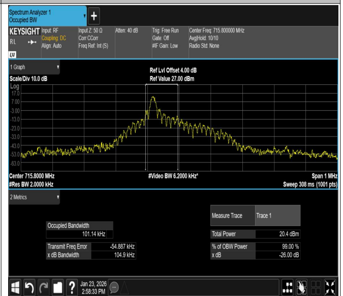
Band12-15KHz-QPSK-23178-1RB#0-PASS
