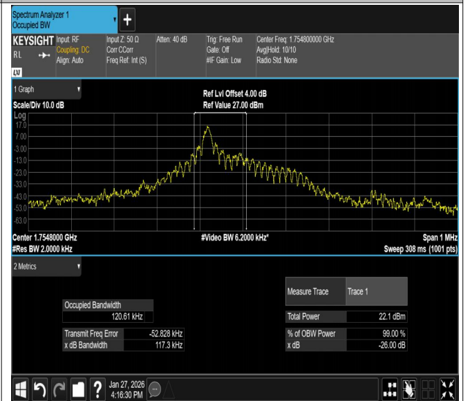
Band4-15KHz-QPSK-20398-1RB#0-PASS
