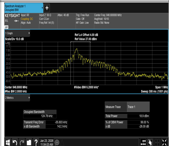
Band5-15KHz-QPSK-20648-1RB#0-PASS
