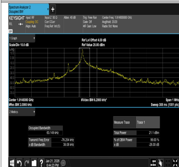
Band25-15KHz-QPSK-26042-12RB#0-PASS
