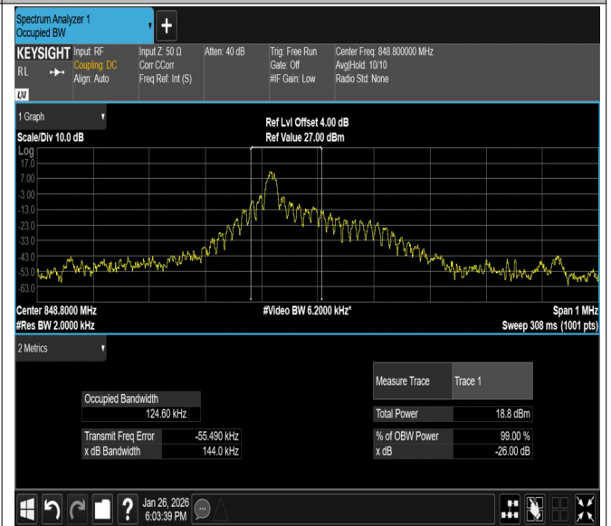
B26(824-849)-15KHz-QPSK-27038-1RB#0-PASS
