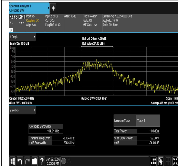
Band25-15KHz-QPSK-26688-12RB#0-PASS
