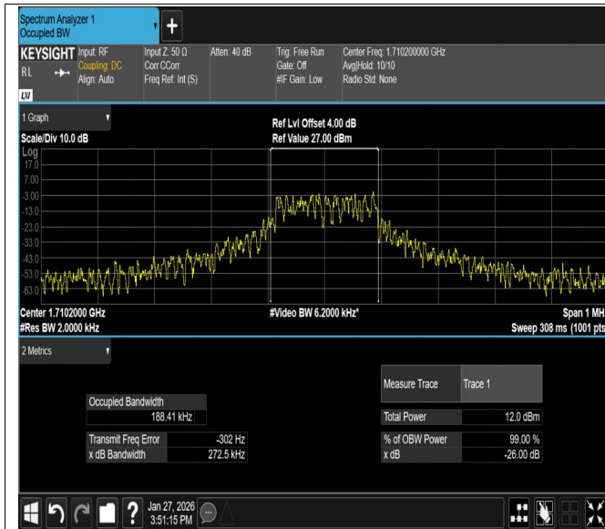
Band66-15KHz-QPSK-132322-12RB#0-PASS
