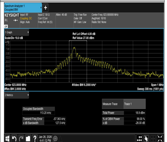
B26(814-824)-15KHz-QPSK-26788-1RB#0-PASS
