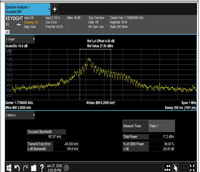
Band66-15KHz-QPSK-132670-1RB#0-PASS
