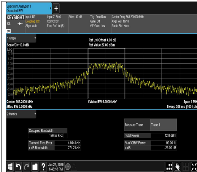
Band71-15KHz-QPSK-133297-12RB#0-PASS
