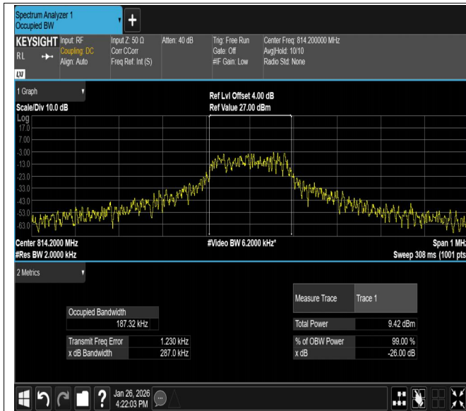
B26(814-824)-15KHz-QPSK-26740-12RB#0-PASS
