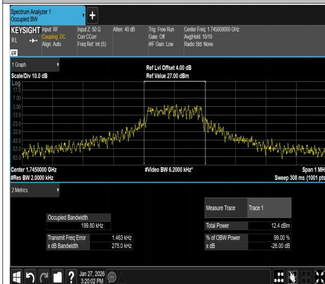
Band66-15KHz-QPSK-132670-12RB#0-PASS
