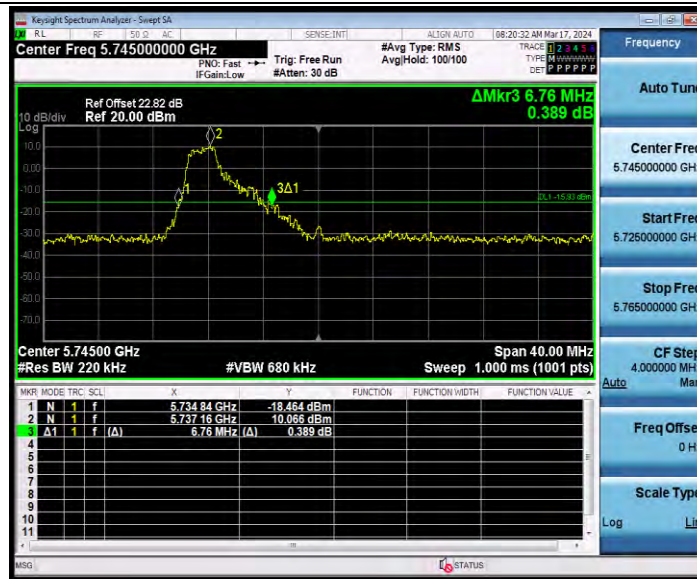
11AX20ISO_Ant1_5745_52Tone_RU37
