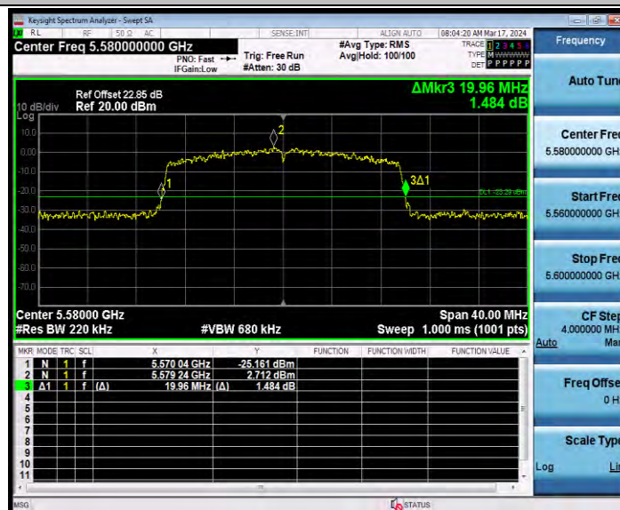
11AX20SISO_Ant1_5580_242Tone_RU61
