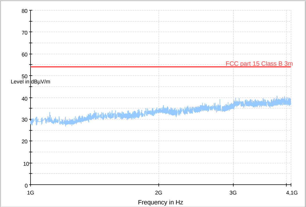
TX Spurious 1G-4G
