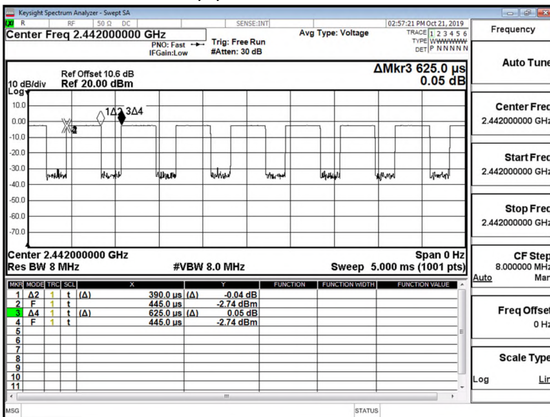
Duty Cycle_BLE_1M_MidCH20-2442
