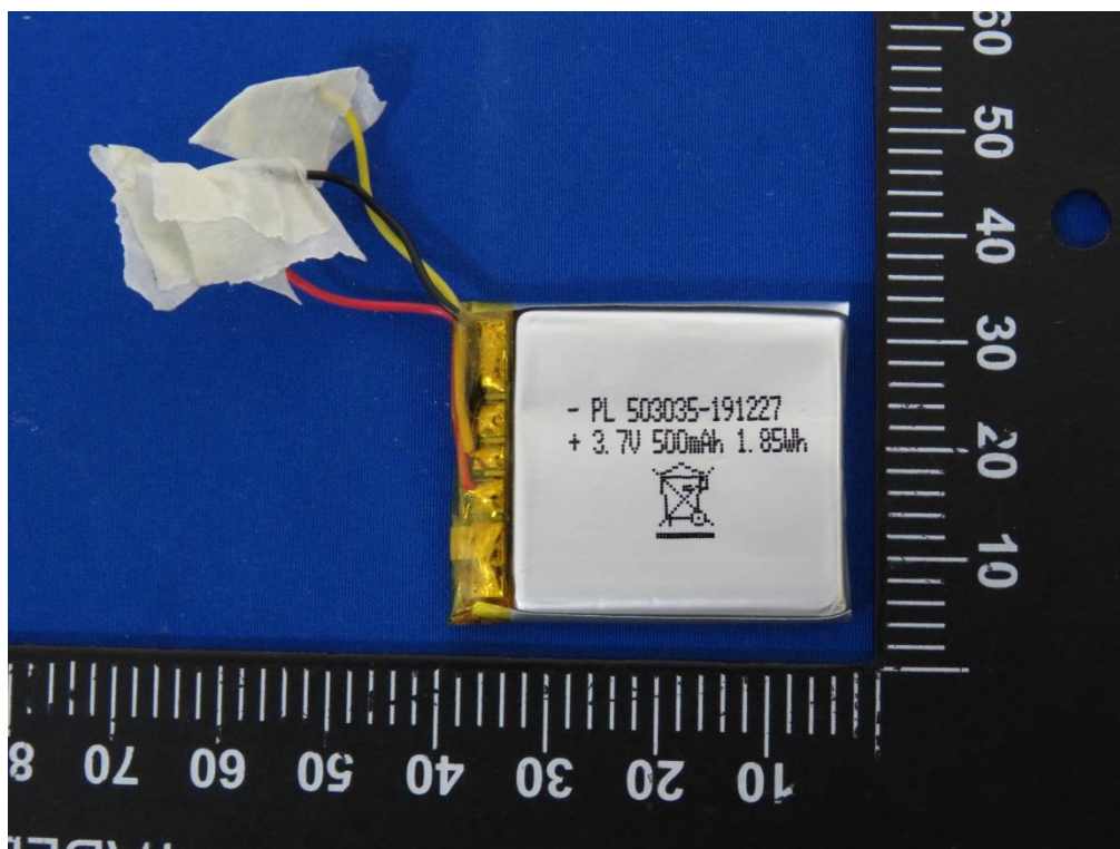
Battery: PL503035
